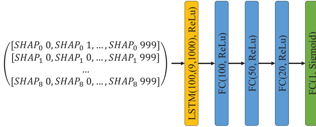
Fig. 3. Proposed adversarial attack detector. The yellow block indicates the LSTM layer which has an input shape of (9,1000) and an output space of 100. ReLu is applied as the activation function for the LSTM layer. The blue blocks are FC layers in the format of (units, activation). The green block indicates the output layer of the adversarial detector, which is also formed from the FC layer and outputs a Boolean to detect adversarial attacks. (For interpretation of the references to colour in this figure legend, the reader is referred to the web version of this article.)
