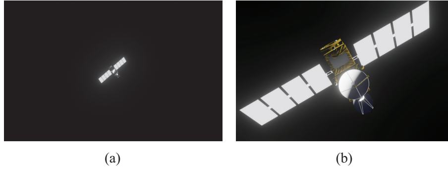
Fig. 4. Examples of synthetic data generated from Blender. (a) image captured at a camera position of (0, 0, 60 m). (b) image captured at a camera position of (0, 0, 10 m). Random rotation is applied to the target spacecraft.
