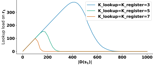
Figure 10: r_1 's lookup load as a function of increasing popularity of s_1 for |N| = 25000 , |D(s_2)| = 100 .
