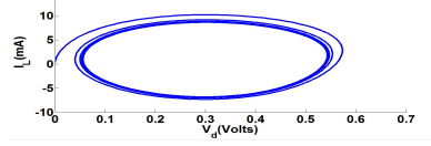
(a) TDO Limit Cycle Simulation
