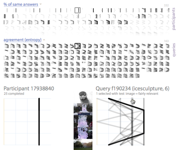
Figure 12: Most participants found the test image in query f190234 irrelevant as expected. This also applies to the last photograph. Three other images are believed to be relevant, which is confirmed by the previews. Hovering over test image \times fairly relevant reveals an insincere participant.
