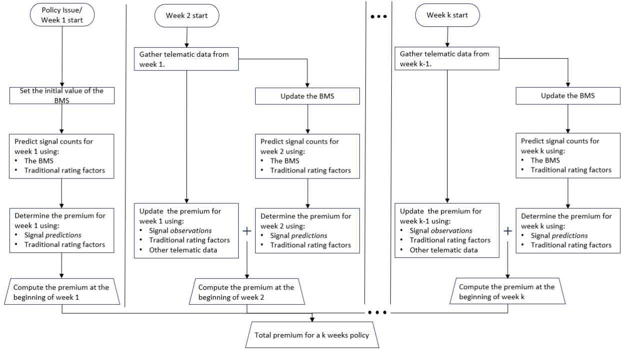
Figure 1: Flowchart of a weekly telematics signal BMS ratemaking scheme
