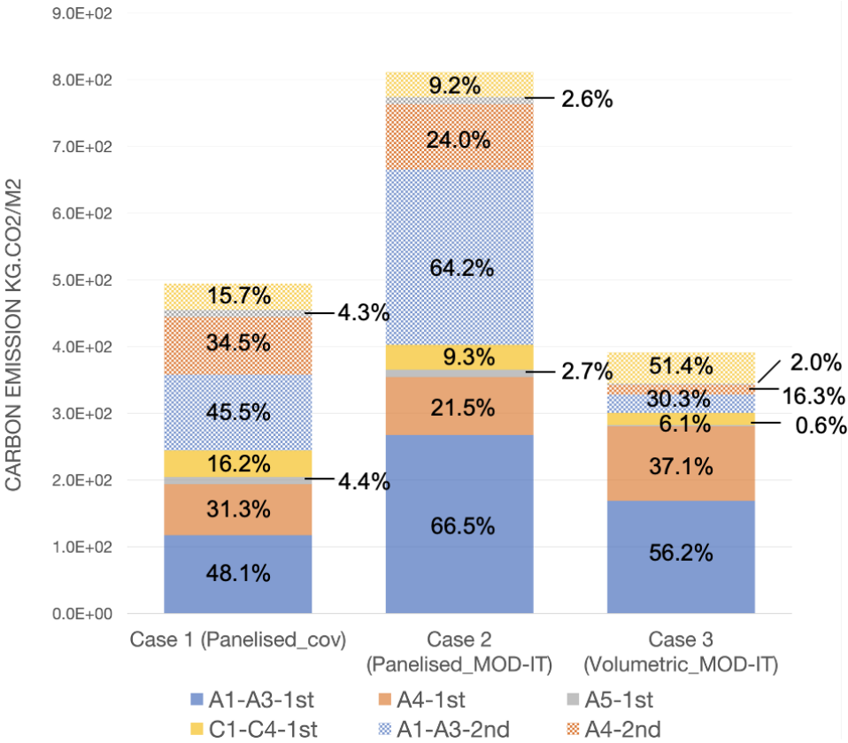
Figure 19. Relative contributions of the building's life cycle stages to the environmental impacts (Note: The above percentages refer to the proportion of each stage within their respective building life cycles.)
