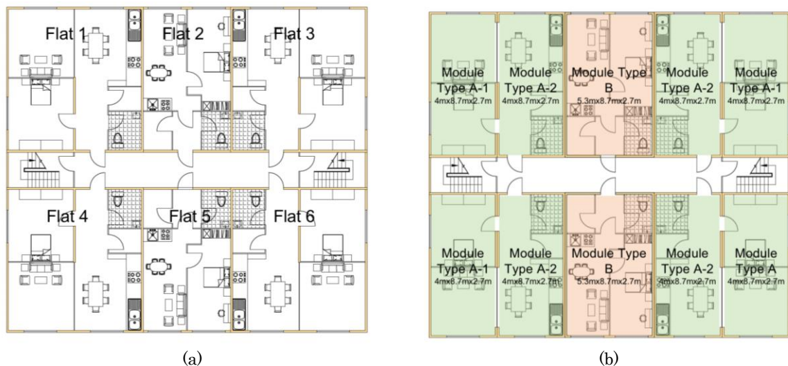
Figure 14. Floor plans and overall structure of the (a) panelised building and (b) the volumetric buildings
