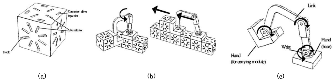
Figure 9. Hardware design of module assembler robot by Terada and Murata [44]
