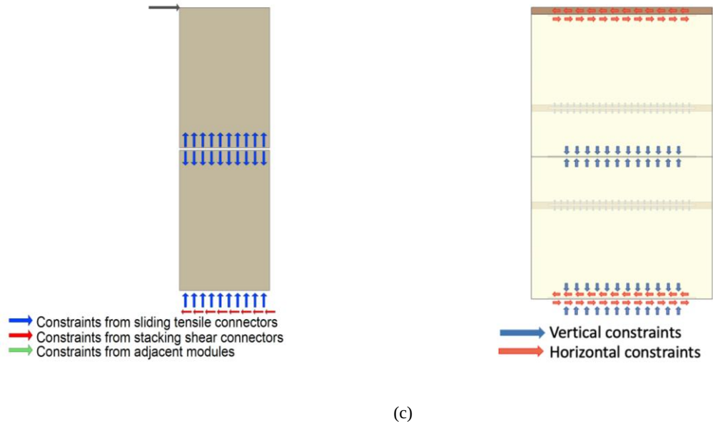
Figure 5. The illustrations of the interlocking connection working mechanism in single module and the sectional elevation of the structure showing the overall constraints in: (a) CLT volumetric structures; (b) CLT platform structures; (c) CLT balloon structures.
