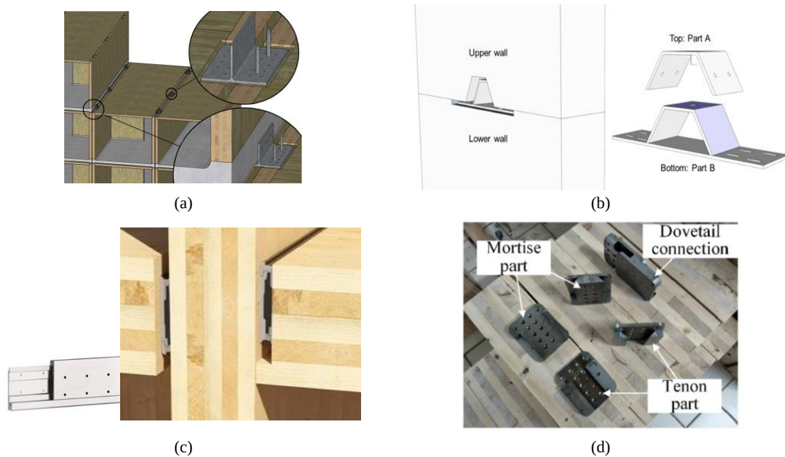
Figure 3. Novel interlocking metal connections for modular CLT structures: (a) Connection for Jakarta Hotel project [36] (b) An inter-module horizontal connection proposed by the University of British Columbia [37] (c) LOCK Connector from Rothoblaas Ltd. [38] (d) Prefabricated metal dovetail connector [39]
