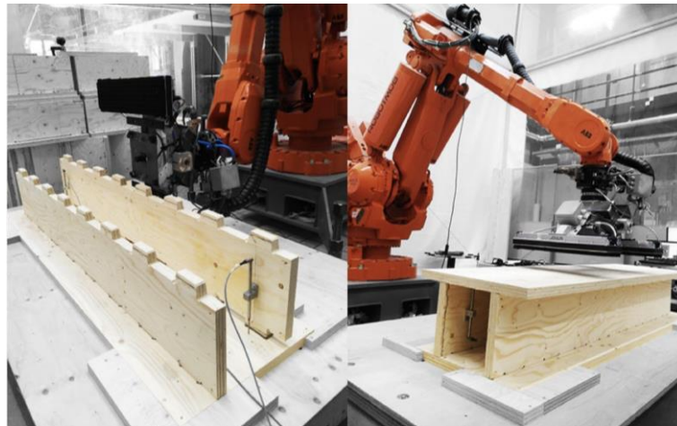
Figure 13. Robotic assembly of a box girder with through-tenon joints [49]
