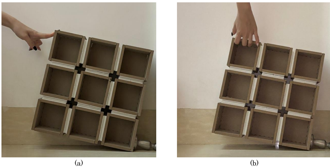
Figure 7. Interlocking connection-reinforced timber modules under (a) lateral and (b) vertical load.
