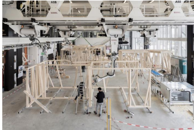
Figure 11. The assembly of the DFABHOUSE [47]
