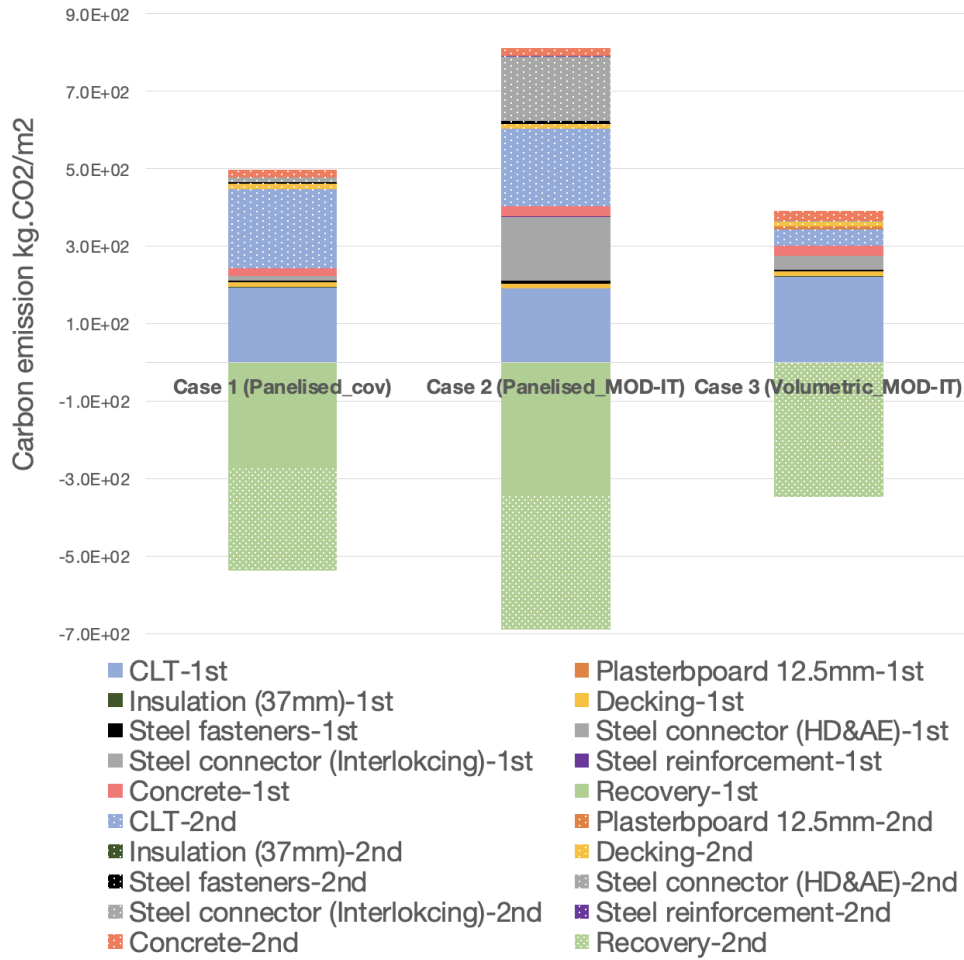
Figure 17. Contribution of different building components to the carbon emission
