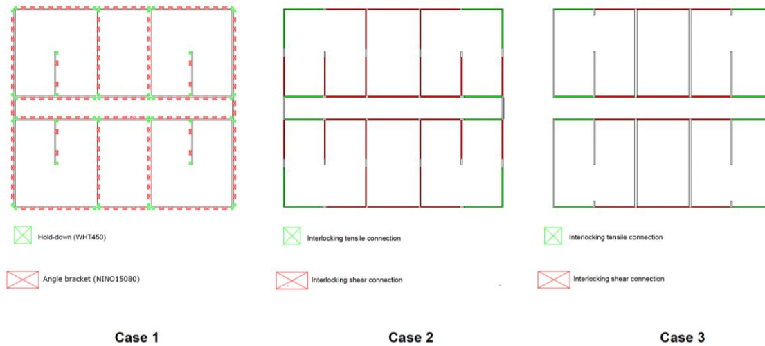
Figure 18. Interlocking connection locations in different buildings
