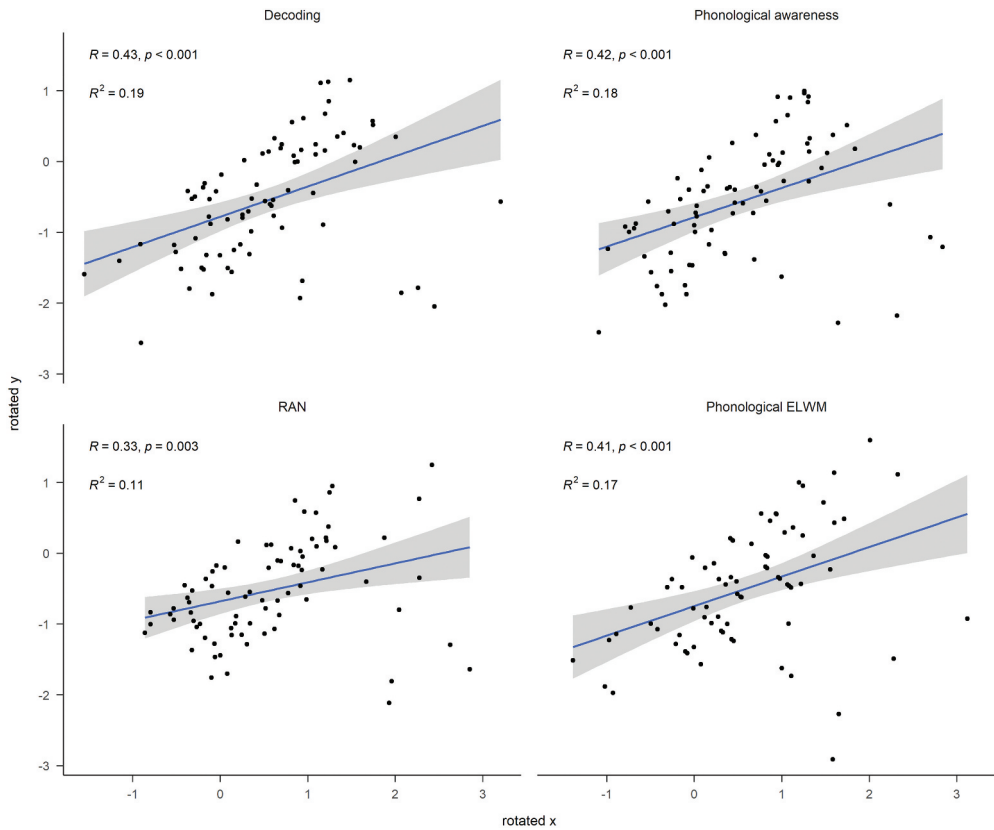
Figure 4. Visualization of rotated data for decoding, phonological awareness, RAN, and phonological ELWM. R^2 and r together with significance values are presented for each plot.
