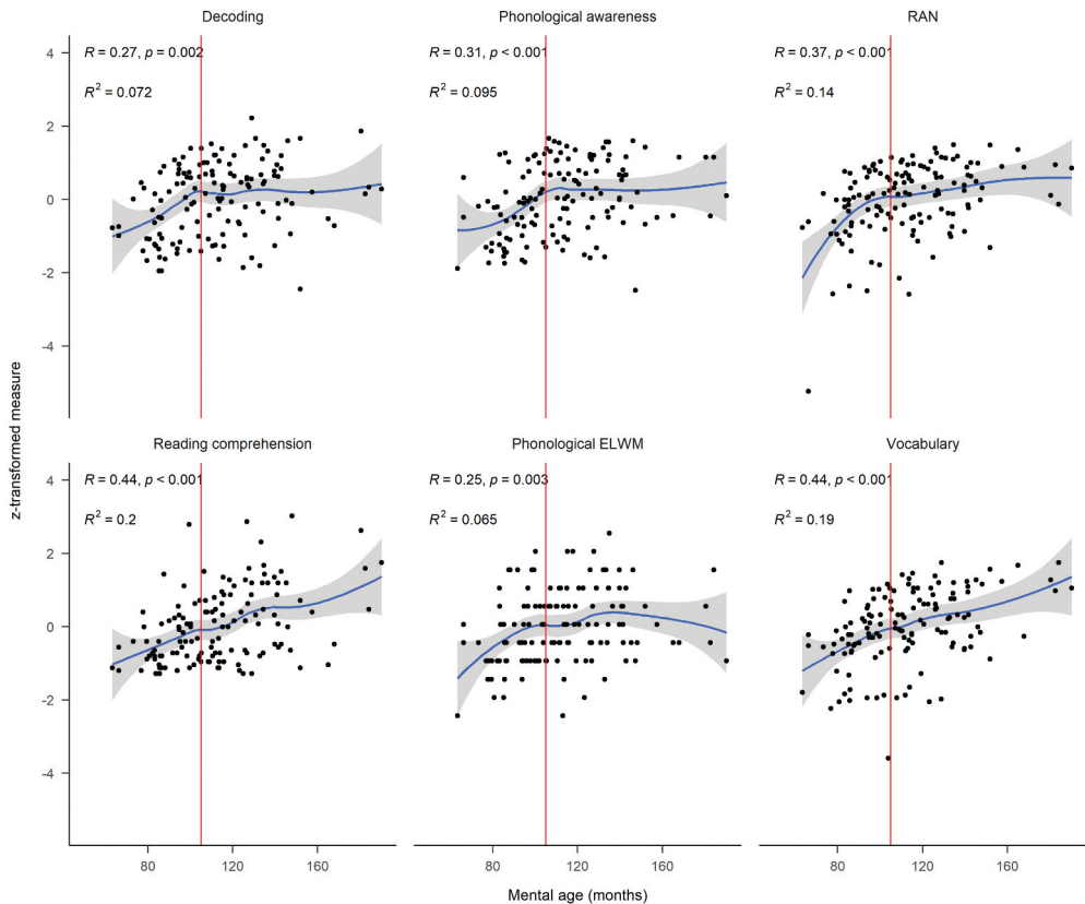
Figure 2. Visualization of all variables fitted against mental age using method = 'loess'. R^2 and r together with significance values are presented for each plot. At an MA of 105 months (indicated by the red line), there is a clear deceleration of growth for decoding, phonological awareness, RAN, and phonological ELWM.
