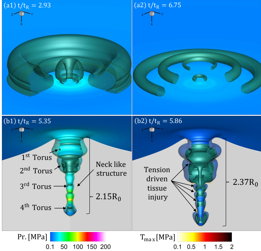
Figure 24: Secondary collapses for detached bubbles with initial stand-off distance S/R_0 = 1.2 . Colormap on solid surface: pressure distribution. Green iso-surface: The gas volume fraction level at a_g = 0.5 . Colormap on cross-subsection: maximum tensile stress distribution. (a1/a2) Collapse near the KS, with torus break up (b1/b2) Collapse near the soft tissue, tissue penetration, and tension-driven tissue damage.
