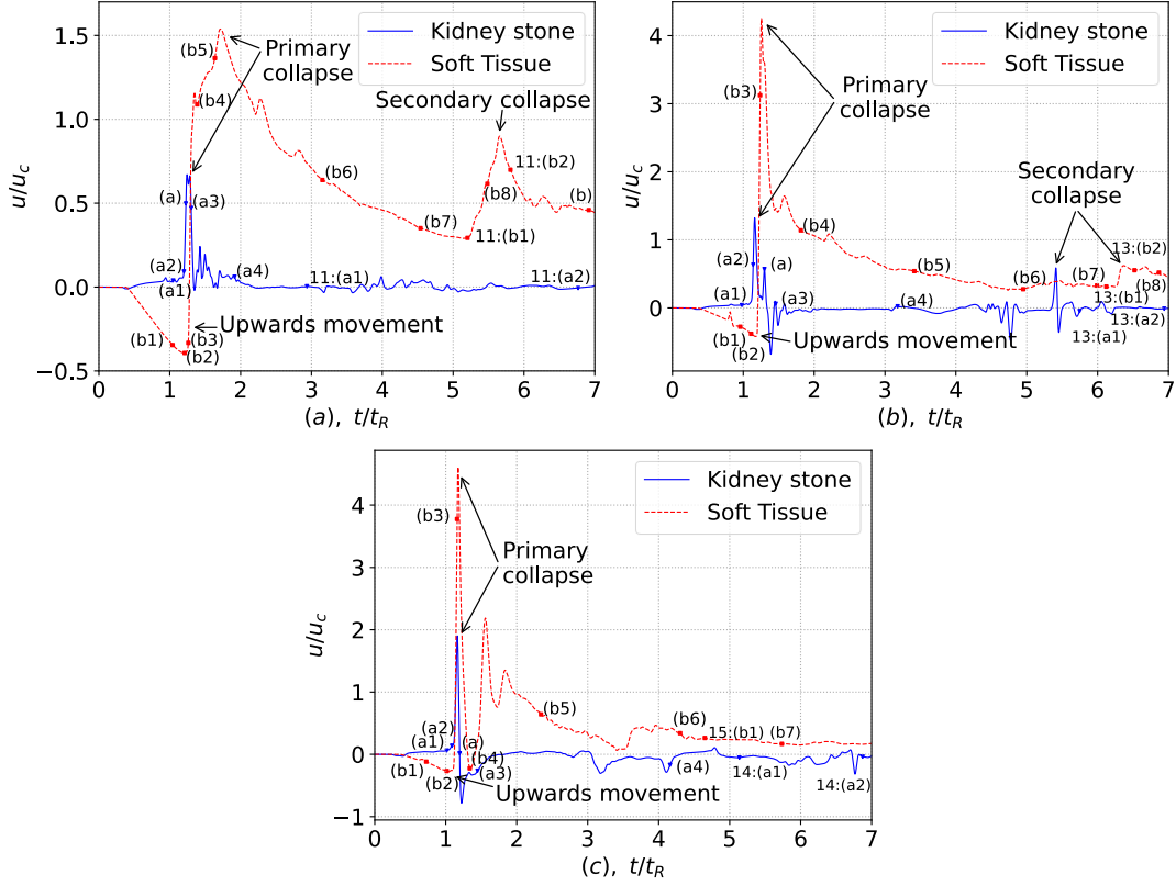
Figure 23: Effect of stand-off distance/attachment on solid boundary's velocity overtime at r/R_0 = 0 . (a) Detached bubbles with stand-off distance S/R_0 = 1.2 , (b) Attached bubbles with stand-off distance S/R_0 = 0.6 and an acute angle, (c) Attached bubbles with stand-off distance S/R_0 = -0.2 and obtuse angle. Time instances given are: (a-a4) for KS, and for ST (b-b8) from Figs. 21,25,27. References to secondary collapse figures 24,26,28 are given with their corresponding number.
