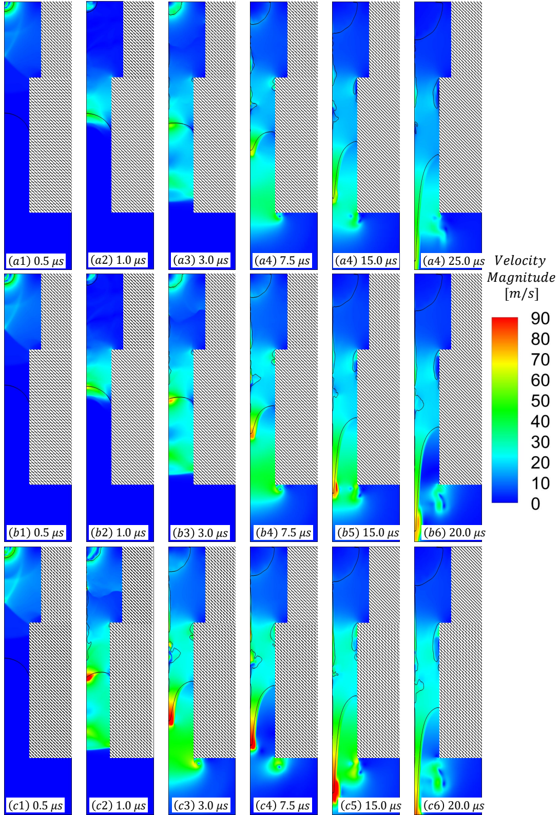
Figure 37: Needle-free injector simulations. Velocity magnitude contours are shown for Cases 6,7 and 8. Isosurfaces of the gas phase with black for vapor volume fraction \alpha_{gas} = 0.5
