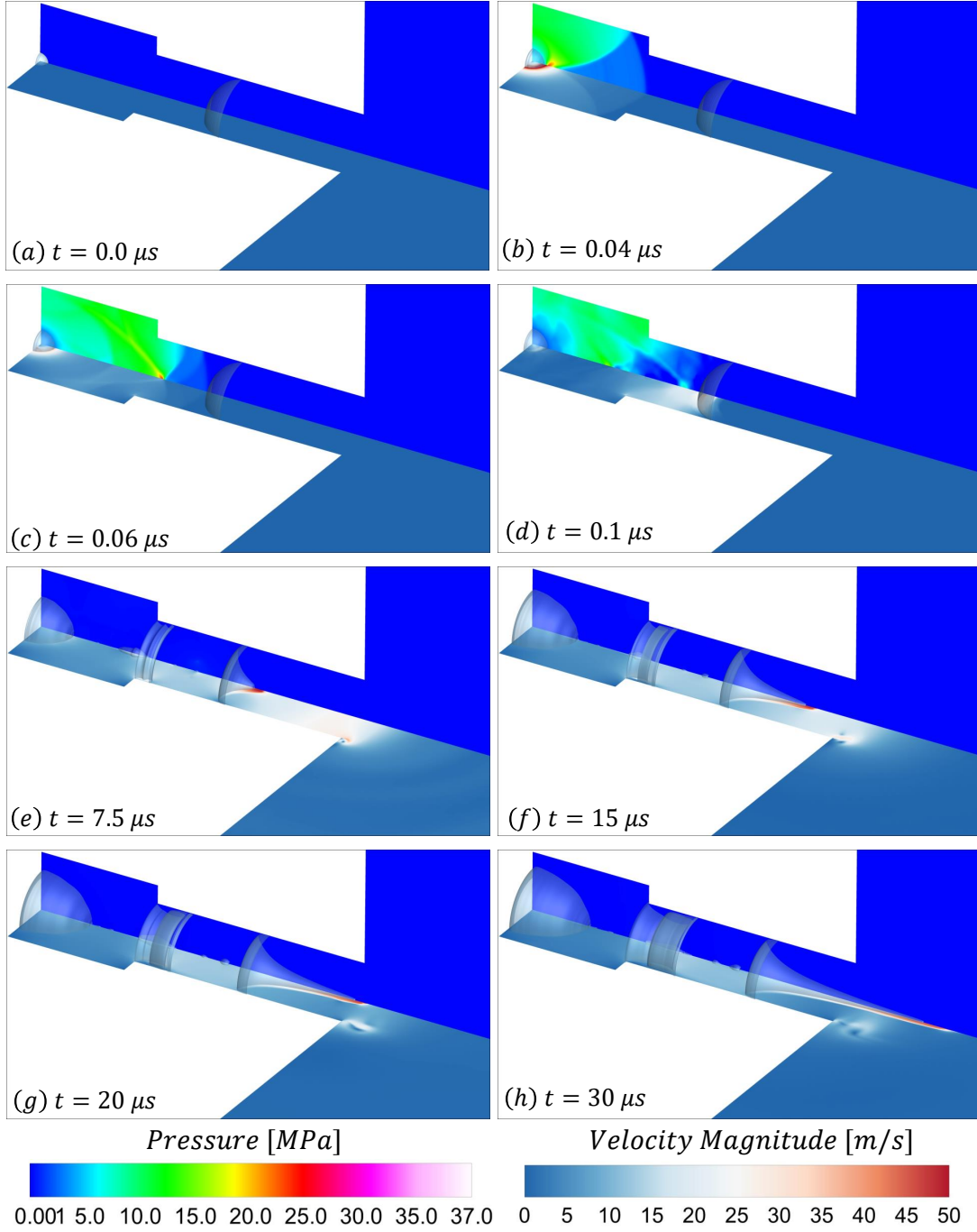
Figure 36: Needle-free injector simulation. Case 2. The pressure field on the x-y plane and velocity magnitude field on the x-z plane are shown. Isosurfaces of the gas phase for gas volume fraction \alpha_{gas} = 0.5
