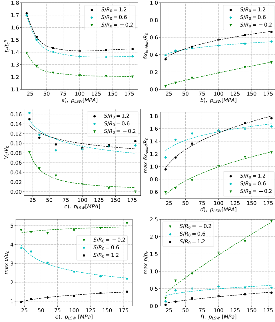
Figure 34: Effect of shock-wave amplitude on the bubble dynamics close to a soft tissue. (a) : normalised collapse time with Rayleigh collapse time. (b) : normalised bubble's collapse position in relation to the initial bubble center. (c) : normalised gas volume V_c of the bubble at the initial collapse time t_c . (d) : Maximum deformation of the solid interface at the axis of symmetry r/R_0 = 0 . (e) : Maximum velocity at the solid boundary interface overtime at r/R_0 = 0 . (f) : Maximum pressure on the solid interface due to the primary shock wave emission.
