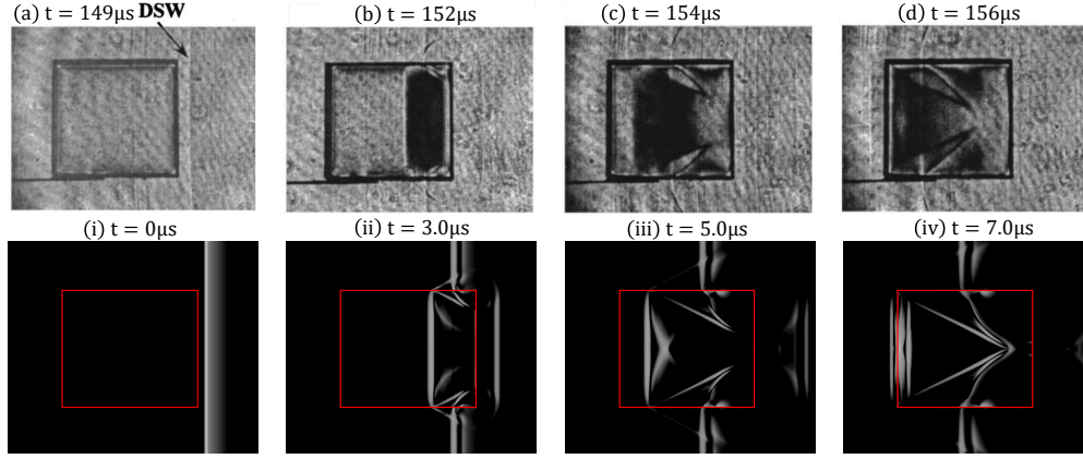
Figure 17: Qualitative comparison of a shock impact to a kidney stone phantom with photoelastic imaging. Top: Experimental work of Xi and Zhong [179] Bottom: Numerical results, contours depicting gradient of principal tensile stress.
