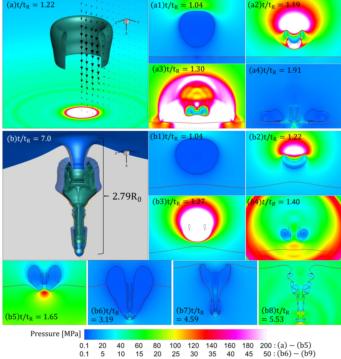
Figure 21: Shock-induced collapse of a detached gas bubble with initial stand-off distance S/R_0 = 1.2 . Colormap: pressure distribution. Black iso-surface: The gas volume fraction level at a_g = 0.5 corresponds to the bubble interface. Red iso-surface: The solid volume fraction at a_s = 0.5 represents the solid interface. (a-a4) Collapse near the KS, (b-b8) collapse near the soft tissue. (a) Detail of the jet formation (arrows velocity magnitude) and the impact of the shock on the KS (pressure contour on the KS surface), (b) detail of tissue deformation. Same magnification in all figures, except the (a/b), and (b5-b8)
