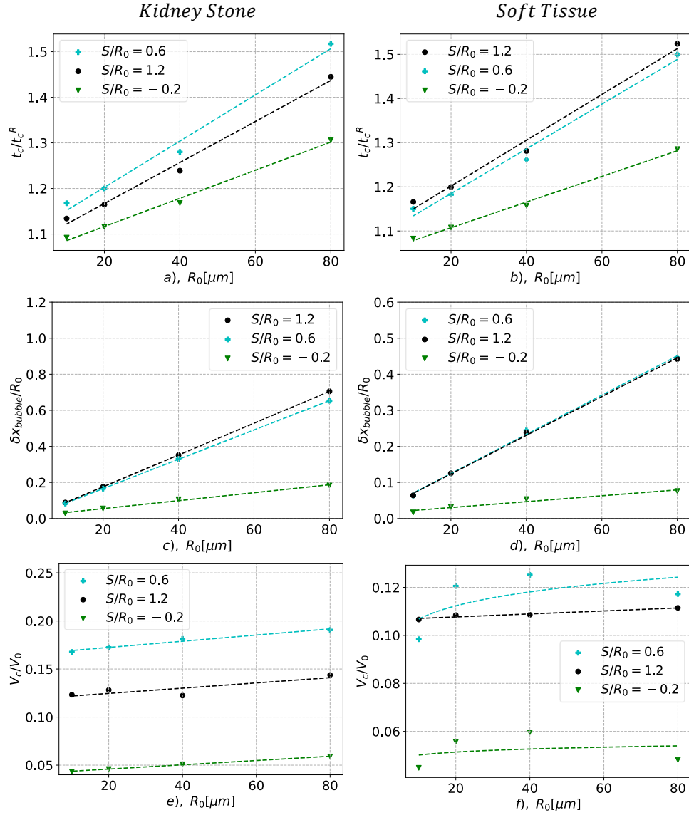
Figure 32: Effect of initial bubble size and attachment configuration on bubble dynamics. (a) : Normalised collapse time with Rayleigh collapse time for kidney stones and (b) for soft tissue. (c) : Normalised bubble's collapse position close to a kidney stone surface in relation to the initial bubble (d) close to soft tissue. (e) Normalised gas volume V_c of the bubble at the collapse time t_c close to a kidney stone and (f) close to soft tissue
