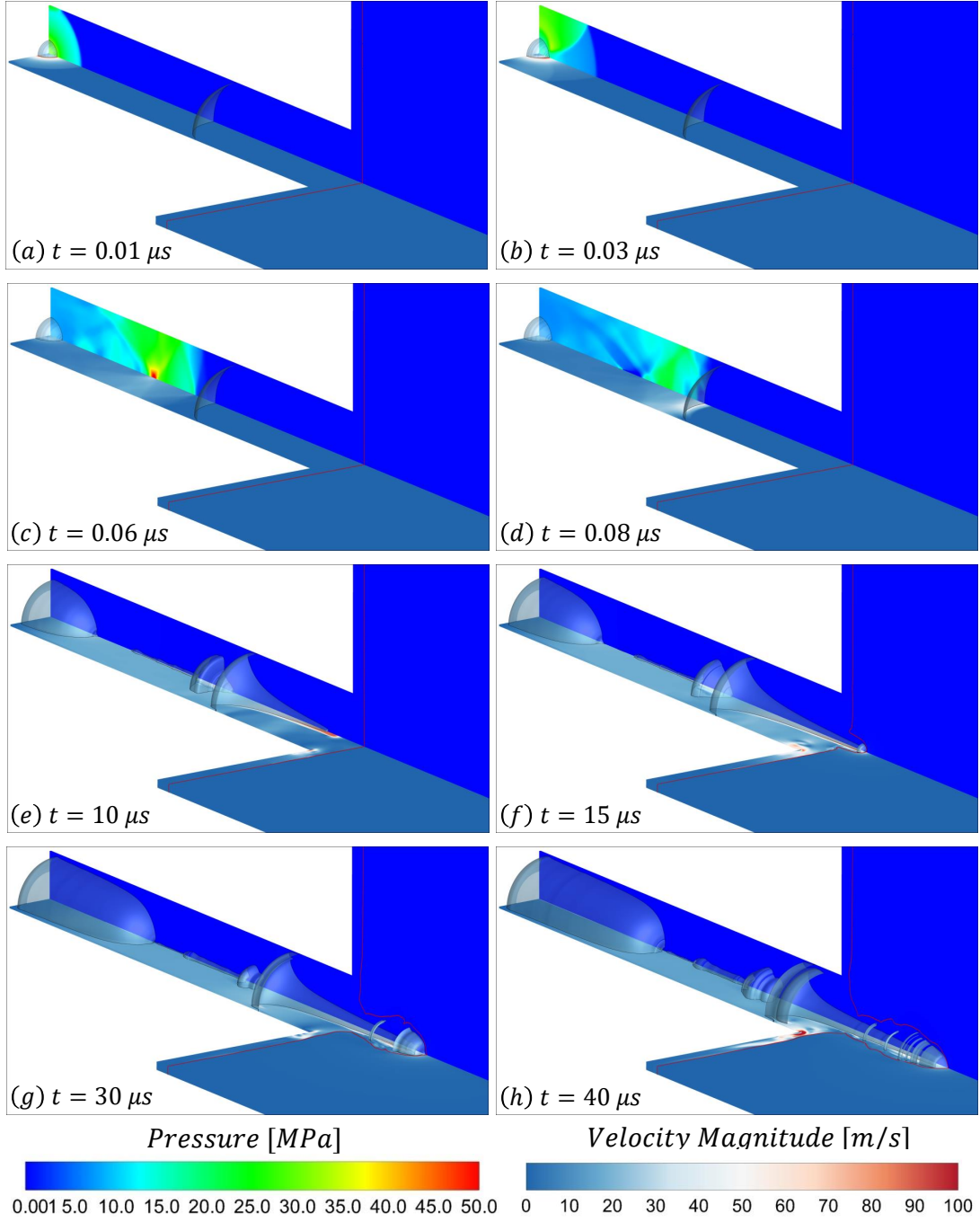
Figure 39: Needle-free injector simulation. The pressure field on the x-y plane and velocity magnitude field on the x-z plane are shown. Isosurfaces of the gas phase for gas volume fraction \alpha_{gas} = 0.5
