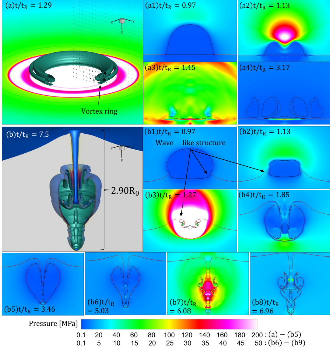
Figure 25: Shock-induced collapse of an attached gas bubble with initial stand-off distance S/R_0 = 0.6 . Colormap: pressure distribution. Black iso-surface: The gas volume fraction level at a_g = 0.5 corresponds to the bubble interface. Red iso-surface: The solid volume fraction at a_s = 0.5 represents the solid interface. (a-a4) Collapse near the KS, (b-b8) collapse near the soft tissue. (a) Detail of the jet formation (arrows velocity magnitude) and the impact of the shock on the KS (pressure contour on the KS surface), (b) detail of tissue deformation. Same magnification in all figures, except the (a/b), and (b5-b8)
