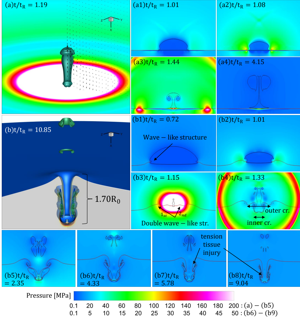
Figure 27: Shock-induced collapse of an attached gas bubble with initial stand-off distance S/R_0 = -0.2 . Colormap: pressure distribution. Black iso-surface: The gas volume fraction level at a_g = 0.5 corresponds to the bubble interface. Red iso-surface: The solid volume fraction at a_s = 0.5 represents the solid interface. (a-a4) Collapse near the KS, (b-b8) collapse near the soft tissue. (a) Detail of the jet formation (arrows velocity magnitude) and the impact of the shock on the KS (pressure contour on the KS surface), (b) detail of tissue deformation. Same magnification in all figures, except the (a/b), and (b6-b8)
