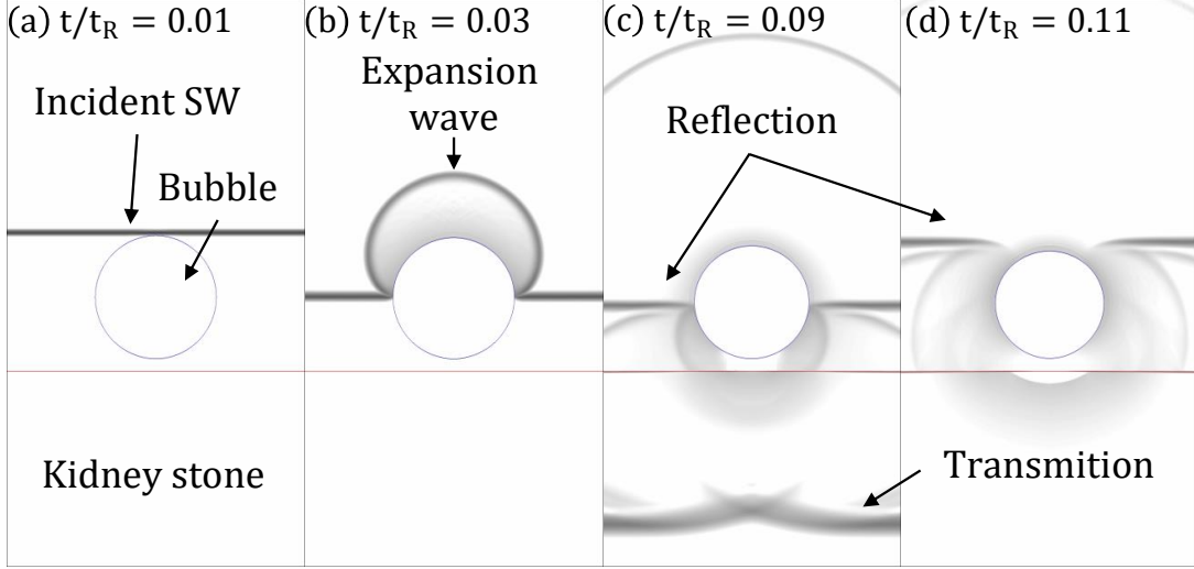
Figure 20: Contour map of the evolution of shock structure before the bubble collapse. The gray-scale colormap corresponds to the magnitude of the pressure field gradient. Blue iso-surface: The gas volume fraction level at a_g = 0.5 , representing the bubble interface. Red iso-surface: The solid volume fraction at a_s = 0.5 represents the solid interface. (a) The initial configuration before the shock wave impact. (b) The expansion wave, (c) and (d) The reflection of the shock wave in the fluid and its transmission inside the solid phase.
