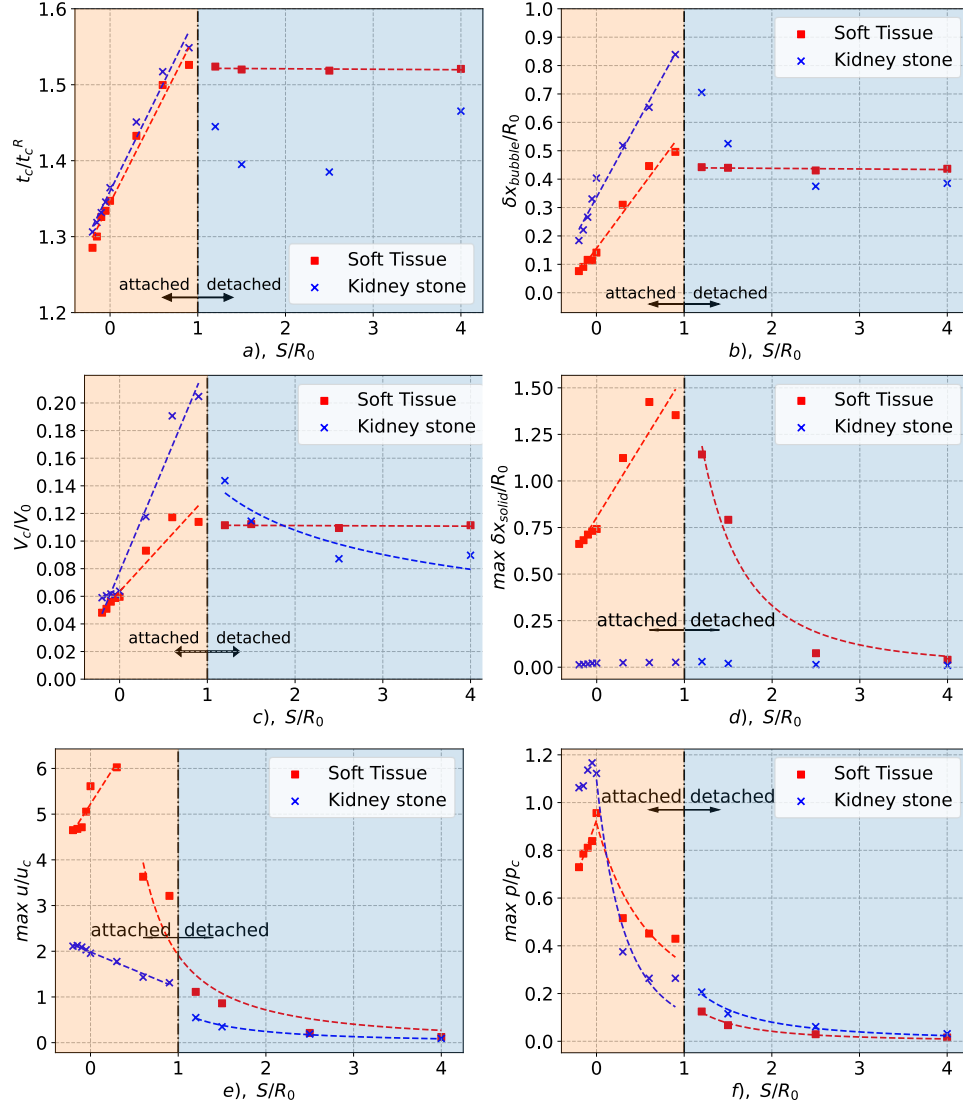
Figure 31: Effect of stand-off distance/attachment on bubble dynamics. (a) : normalised collapse time with Rayleigh collapse time. (b) : normalised bubble's collapse position in relation to the initial bubble center. (c) : normalised gas volume V_c of the bubble at the initial collapse time t_c . (d) : Maximum deformation of the solid interface at the axis of symmetry r/R_0 = 0 . (e) : Maximum velocity at the solid boundary interface overtime at r/R_0 = 0 . (f) : Maximum pressure on the solid interface due to the primary shock wave emission.
