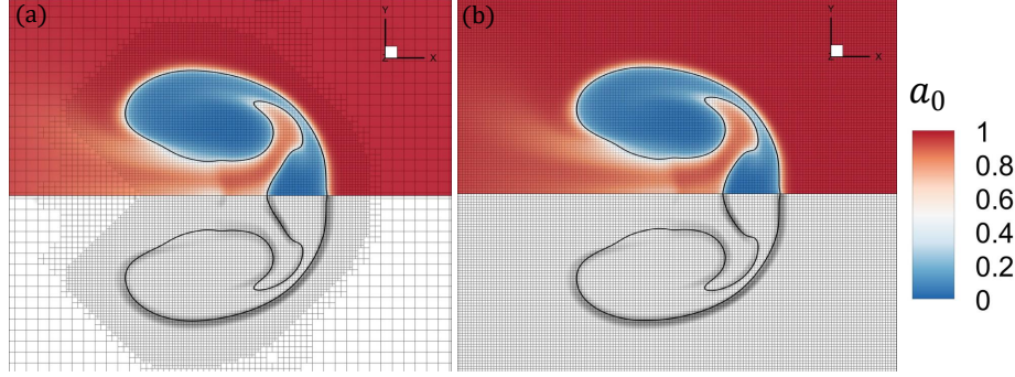
Figure 16: Shock-induced bubble collapse close to a rigid wall. Colormap: volume fraction ( \alpha_0 ) contour of water. Gray-scale: density gradient magnitude. Black iso-surface: bubble interface. Left : AMR with 3 levels of refinement on the interfaces, Right : Uniform refinement with 3 levels.
