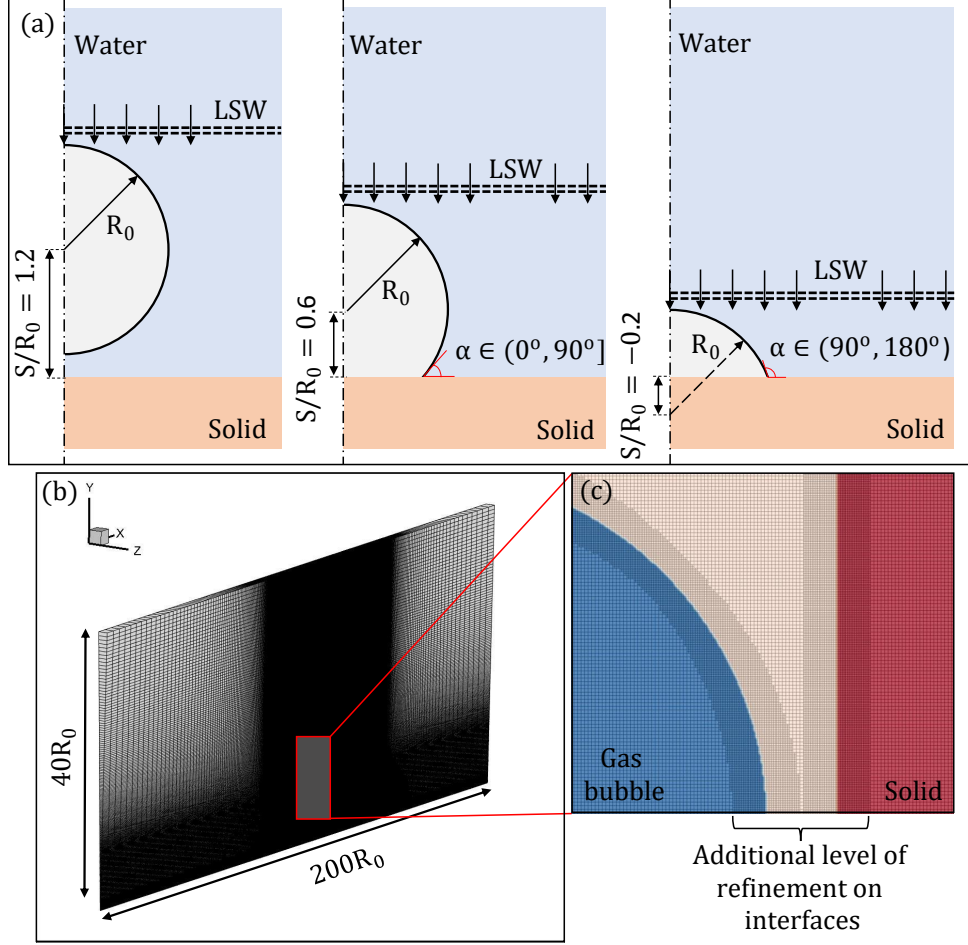
Figure 19: Shock-induced gas bubble collapse case configurations. (a) Types of bubble attachment on the solid surface based on the angle \alpha (b) Computational domain. The initial ancestral mesh consists of 125K elements, (c) Detail of Gas/Liquid/Solid interfaces, additional levels of refinement on the bubble and solid interfaces
