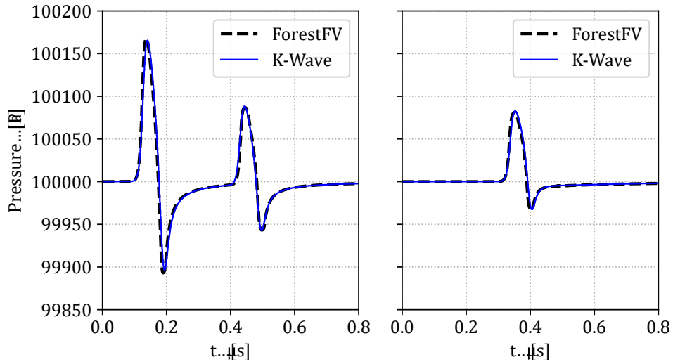
Figure 14: Comparison of numerical solution of the wave transmission across a fluid/solid interface, using the developed ForestFV solver presented in this paper and the K-Wave [163] linear elastic-acoustic model. Left: Pressure time series at probe point (a) (0,2.5)mm. Right: Pressure time series at probe point (c) (0,-2.5)mm
