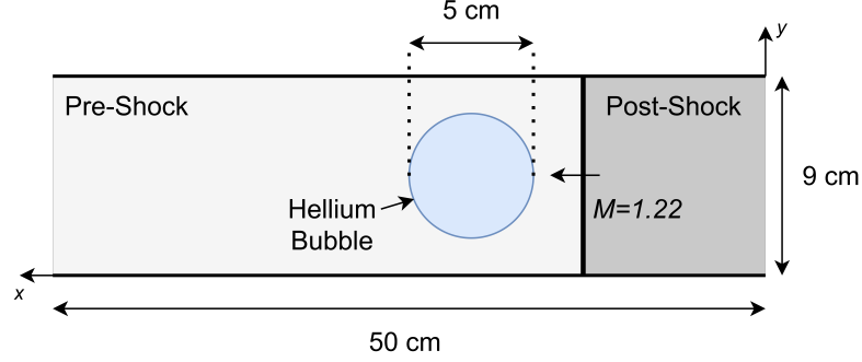
Figure 9: Initial configuration of shock-induced bubble collapse.
