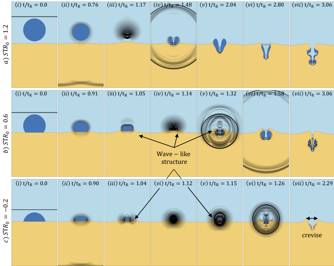
Figure 30: Shock-induced collapse of gas bubbles close to the soft tissue. Color map: represents the areas of different materials (gas/liquid/solid). The gray-scale colormap corresponds to the magnitude of the pressure field gradient. (a(i))-(a(vii)) : detached gas bubble with initial stand-off distance S/R_0 = 1.2 . (b(i))-(b(vii)) : attached gas bubble with an acute interface angle and initial stand-off distance S/R_0 = 0.6 . (c(i))-(c(vii)) : attached gas bubble with an obtuse interface angle and initial stand-off distance S/R_0 = -0.2 .
