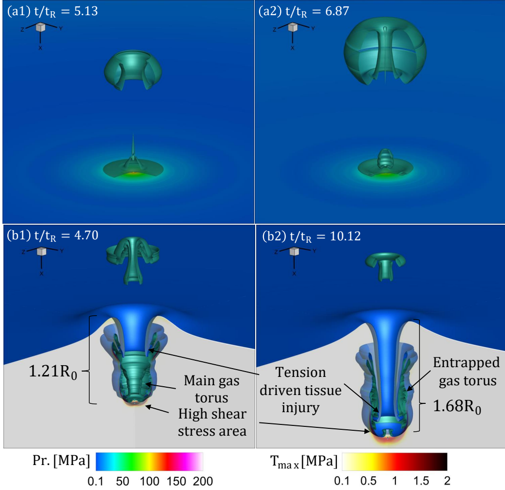
Figure 28: Secondary collapses for detached bubbles with initial stand-off distance S/R_0 = 1.2 . Colormap on solid surface: pressure distribution. Green iso-surface: The gas volume fraction level at a_g = 0.5 . Colormap on cross-subsection: maximum tensile stress distribution. (a1/a2) Collapse near the KS, with torus break up (b1/b2) Collapse near the soft tissue, tissue penetration, and tension-driven tissue damage.
