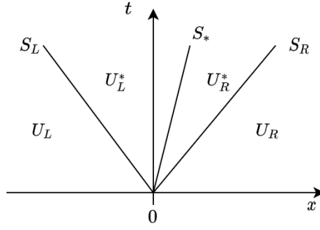
Figure 1: Wave structure of HLLC Riemann solver. The star region is separated into two constant states, by a middle wave with speed S_*
