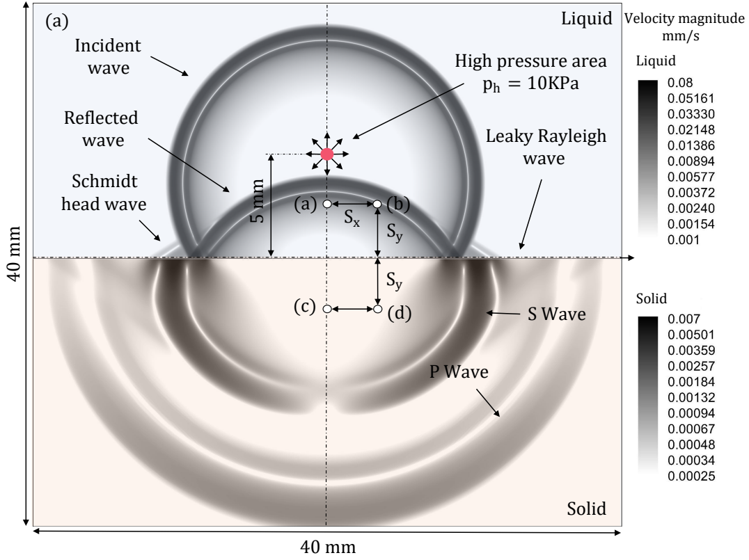
Figure 13: Wave propagation across a fluid-solid interface case setup and velocity magnitude distribution. Top half: fluid region, bottom half: solid region. (a)-(d) pressure sensors with S_x = S_y = 2.5\text{mm} . The initial area of high pressure ( 10\text{KPa} ) is denoted with red. Wave structure in the fluid region consists of the incident wave, the reflection, and the Schmidt head wave. In the solid region S/P and leaky Rayleigh waves.
