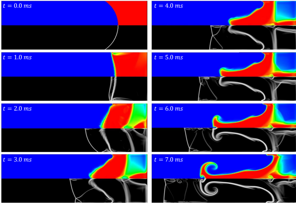
Figure 12: Richtmyer–Meshkov instability. Bottom half presents Schlieren images of each time frame, Top half volume fraction of water.
