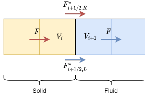
Figure 2: Ghost fluid method, numerical fluxes of Riemann problems across a solid-fluid interface
