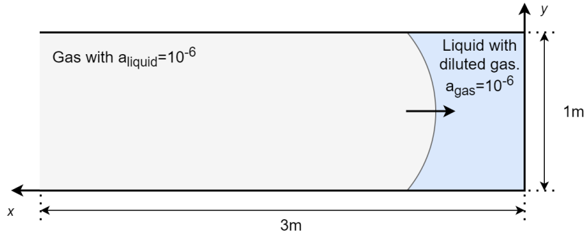
Figure 11: Initial configuration of Richtmyer–Meshkov instability.
