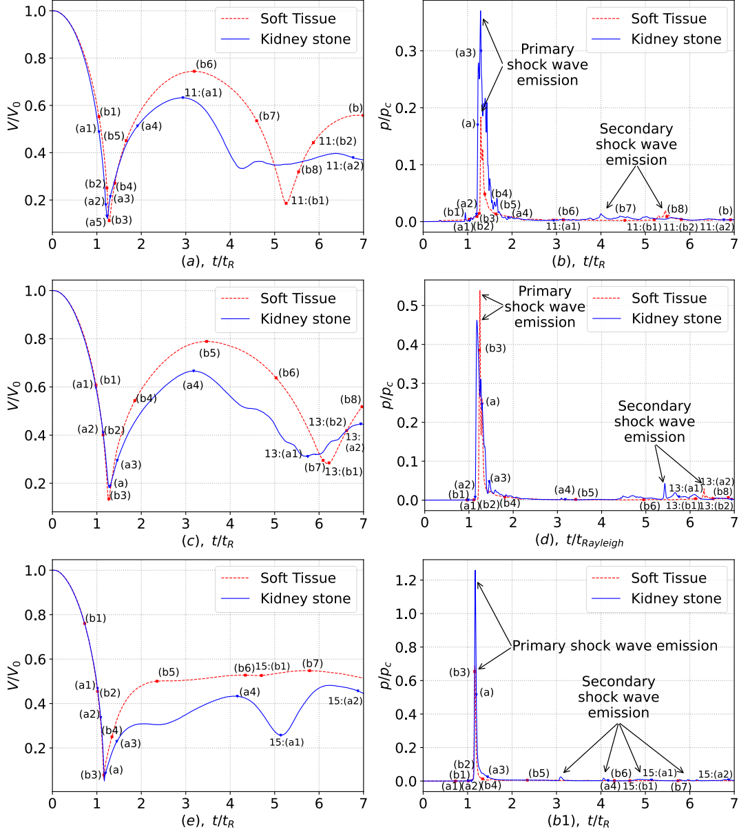
Figure 22: Effect of stand-off distance/attachment on non-dimensionalized gas volume evolution over time and non-dimensionalized pressure on the solid interface at r/R_0 = 0 . (a)/(b) Detached bubbles with stand-off distance S/R_0 = 1.2 , (c)/(d) Attached bubbles with stand-off distance S/R_0 = 0.6 and acute angle, (e)/(f) Attached bubbles with stand-off distance S/R_0 = -0.2 and obtuse angle. Time instances given are: (a-a4) for KS, and for ST (b-b8) from Figs. 21,25,27. References to secondary collapse figures 24,26,28 are given with their corresponding number. Same magnification in all figures, except the (a/b), and (b5-b8)
