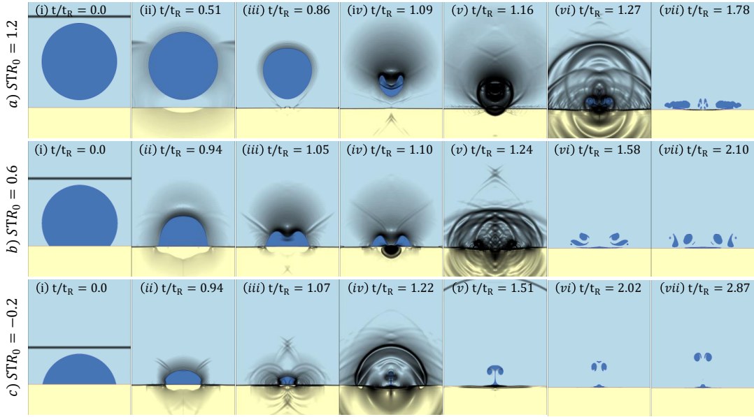
Figure 29: Shock-induced collapse of gas bubbles close to a kidney stone. Color map: represents the areas of different materials (gas/liquid/solid). The gray-scale colormap corresponds to the magnitude of the pressure field gradient. (a(i))-(a(vii)) : detached gas bubble with initial stand-off distance S/R_0 = 1.2 . (b(i))-(b(vii)) : attached gas bubble with an acute interface angle and initial stand-off distance S/R_0 = 0.6 . (c(i))-(c(vii)) : attached gas bubble with an obtuse interface angle and initial stand-off distance S/R_0 = -0.2 .
