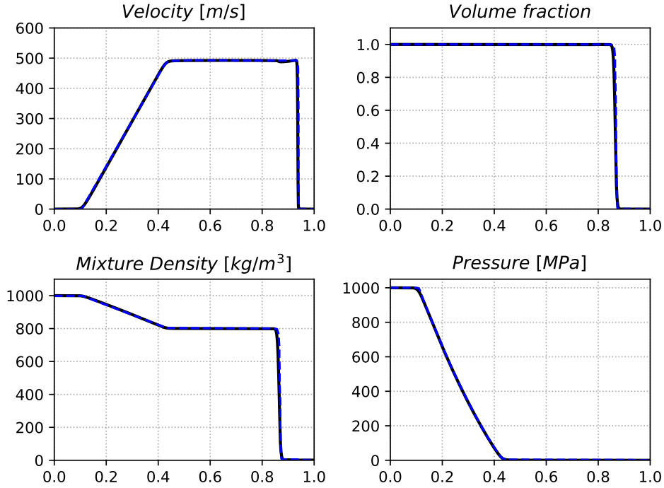
Figure 5: Shock-Tube case: High-pressure water, low-pressure gas. Black symbols represent the results from the presented solver, and the exact solution is shown with the solid blue line. Time: t = 240\mu s
