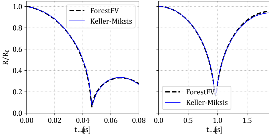
Figure 8: Temporal evolution of the normalized bubble radius for the symmetric gaseous bubble collapse and rebound test case validation. Dashed line: (---) ForestFV result. Solid line(—): Keller-Miksis model. Left: High-pressure ratio case. Right: Low-pressure ratio case. 50 cells were used for the initial bubble radius R_0 .
