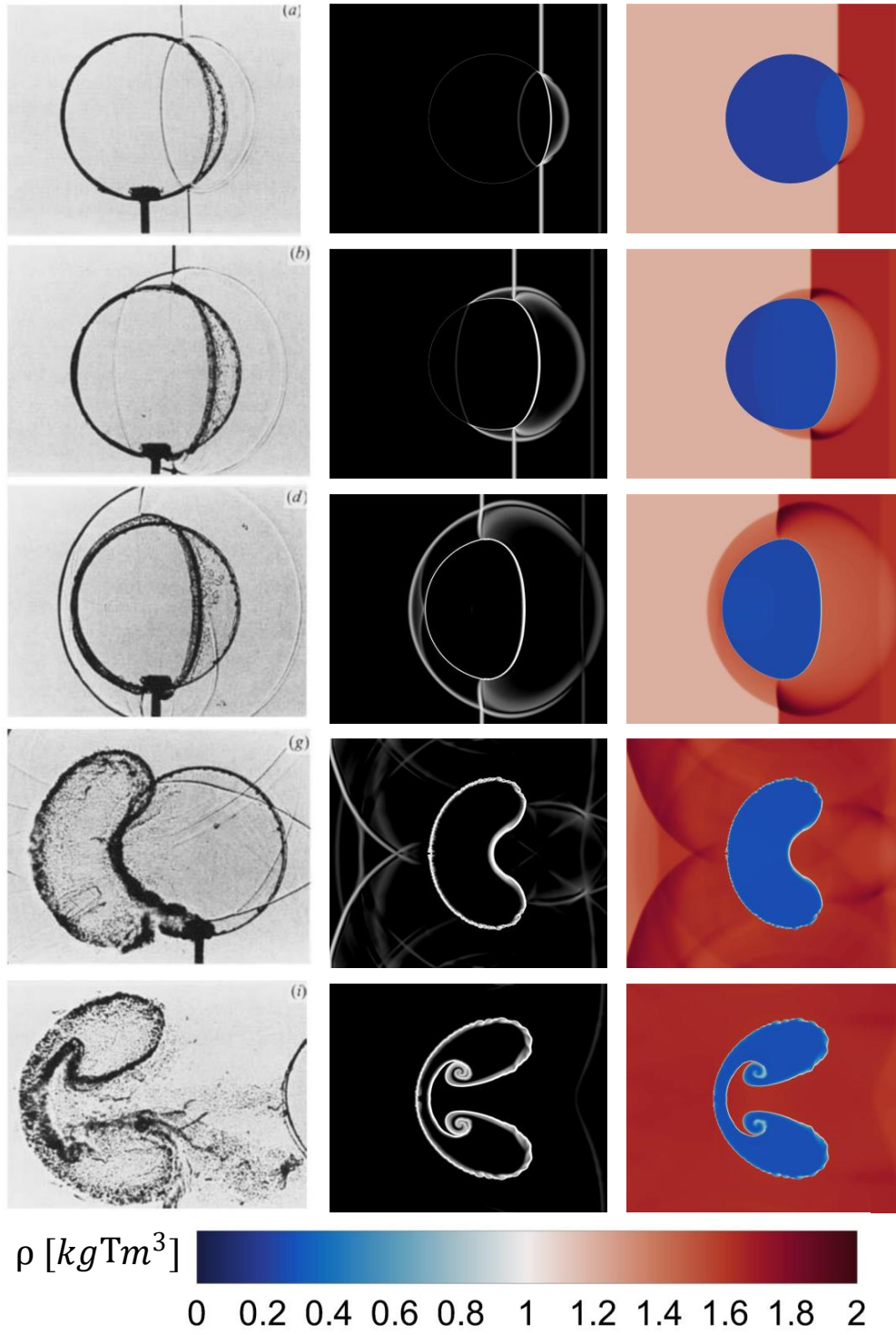
Figure 10: Shock-induced bubble collapse. Left row , shadowgraphs from the experiment of Haas and Sturtevant, Middle row , Schlieren images from the present solver Right row , density contours at times t = 32 \text{ [ms]} , t = 62 \text{ [ms]} , t = 72 \text{ [ms]} , t = 245 \text{ [ms]} , t = 674 \text{ [ms]}
