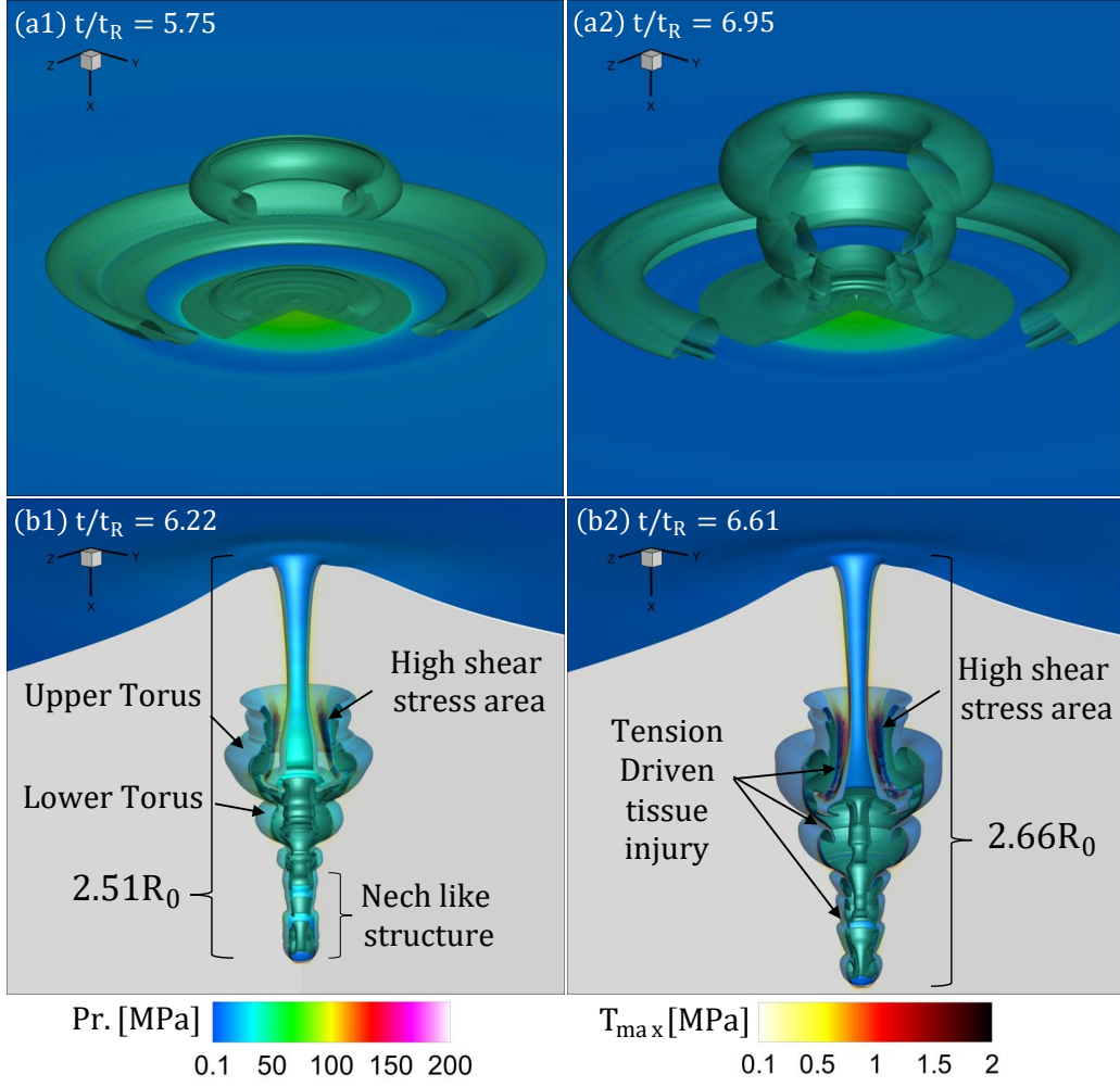
Figure 26: Secondary collapses for detached bubbles with initial stand-off distance S/R_0 = 0.6 . Colormap on solid surface: pressure distribution. Green iso-surface: The gas volume fraction level at a_g = 0.5 . Colormap on cross-subsection: maximum tensile stress distribution. (a1/a2) Collapse near the KS, with torus break up (b1/b2) Collapse near the soft tissue, tissue penetration, and tension-driven tissue damage.
