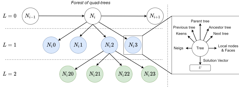
Figure 3: Forest of quad-trees with 2 levels of refined elements. On the left, the address of each element is depicted as N_i . On the right the tree data structure.
