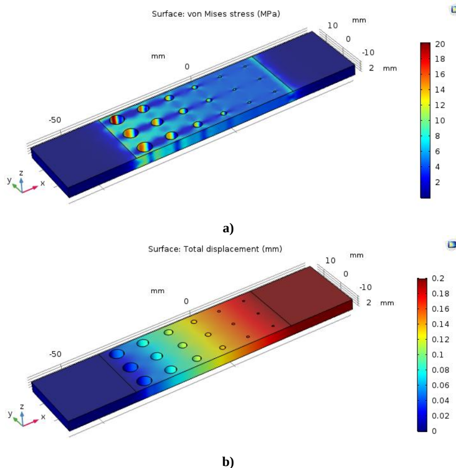
Figure 6. Results of Static Analysis, a) von Mises Stress: 22.8 MPa, b) Displacement: 0.2mm
