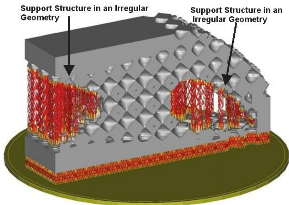
Figure 25. Support Structure in A Topologically-Optimized Part [36]
