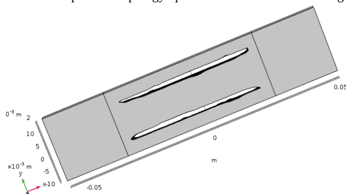
Figure 20. Final Configuration of the Sample after Topology Optimization with 10% Volume Fraction as Constraint
