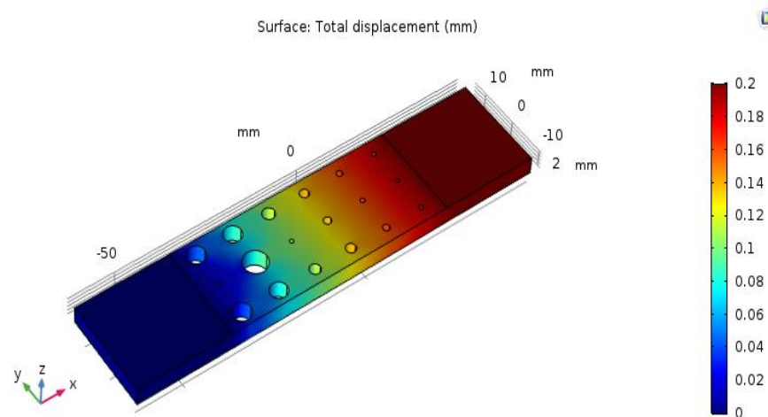
Figure 18. Results of Static Analysis after Optimization Process, a) von Mises Stress: 20 MPa, b) Displacement: 0.2mm
