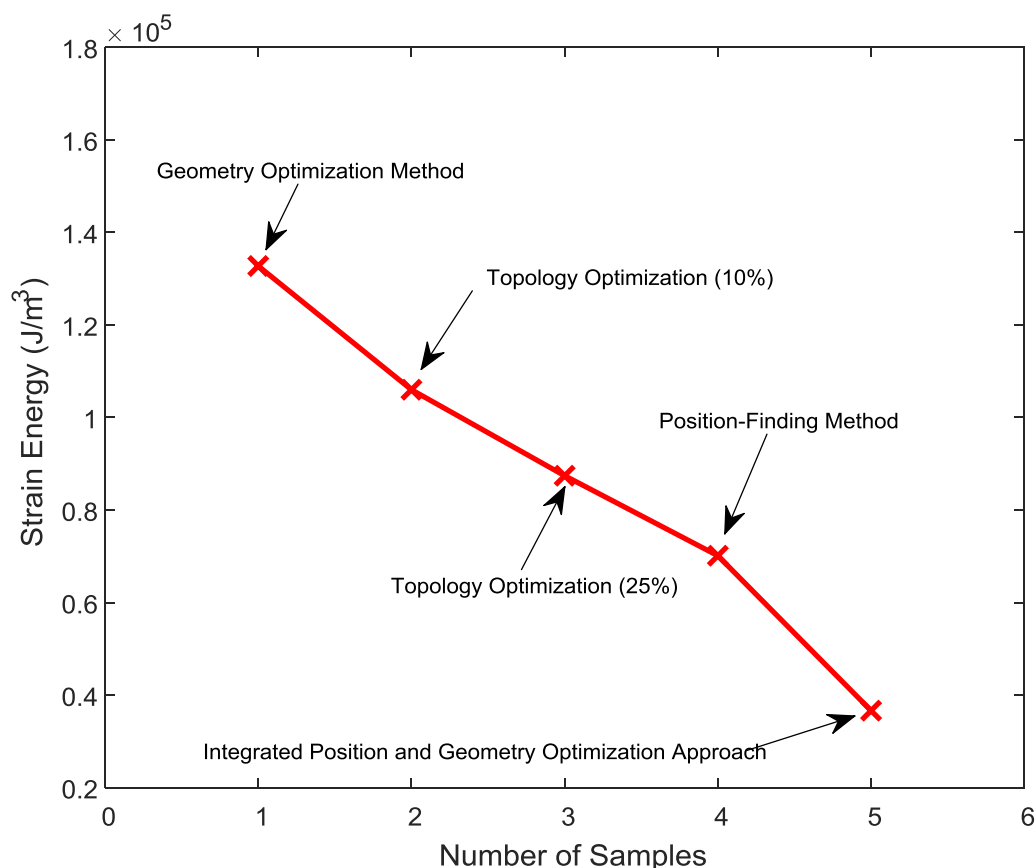
Figure 24. Comparison between Stiffness for each Sample in terms of Strain Energy per Unit Volume (J/m³)
