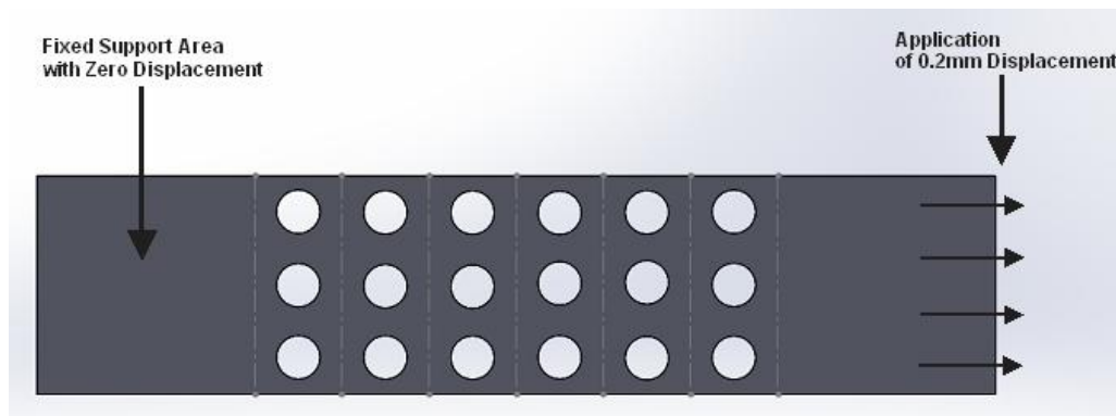
Figure 2. Boundary Condition and Applied Displacement
