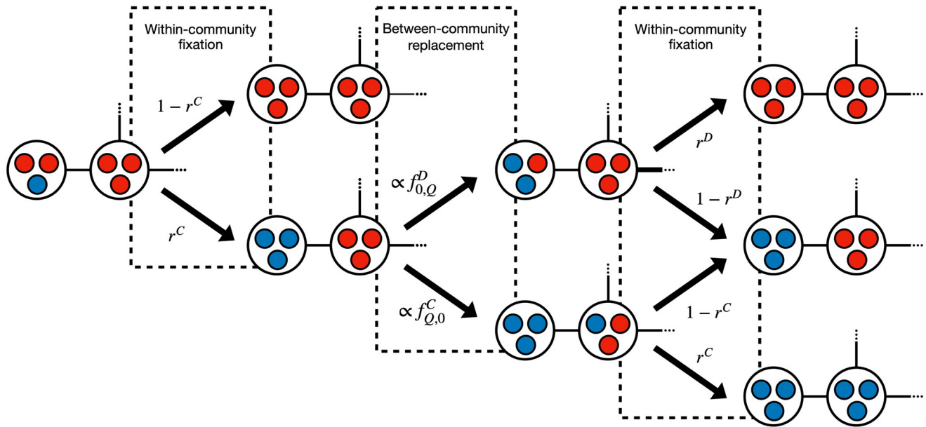
Fig 2. Fixation process in a population of connected communities under the asymptotic limit of high home fidelity. For simplicity, let us consider the scenario where one mutant cooperator emerges in a population of defectors. The new strategy will fixate within the community where it originated with a probability of r^C . The state attained has homogeneous communities and may change only through the occurrence of a between-community replacement. This involves either a cooperator replacing a defector from an adjacent community or the reverse, with probabilities proportional to their respective communal fitness f_{Q,0}^C and f_{0,Q}^D . Each of those events may be followed by the within-community fixation of the new type, with respective probabilities r^C and r^D . If within-community fixation is unsuccessful, it will result in the restoration of the previous number of homogeneous communities of cooperators. However, if within-community fixation is successful, it will respectively increase or decrease by one the number of communities of cooperators in the network. The transition probability ratio \Gamma (see Eq 10) between these two possible state transitions is constant and can be obtained from this diagram. The represented probabilities are the same under BDB, DBD, LB and LD dynamics. Under DBB and BDD dynamics, within-community fixation probabilities are computed from Eqs 15 and 16, and the transition probability ratio is obtained from Eq 17.
