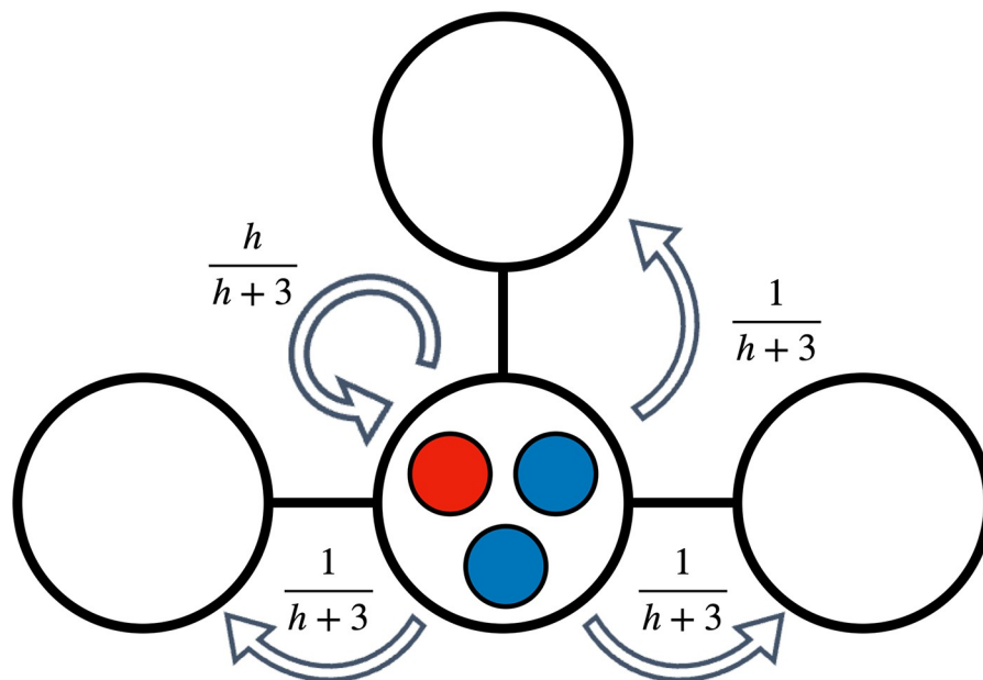
Fig 1. Representation of a small community network under the territorial raider model. At each time step, individuals initiate their movement from their home node, and can either remain there or move to any of the adjacent nodes, returning to their home node prior to the next time step. In this figure, we represent the resulting probability distribution for the community in the centre of the network.
