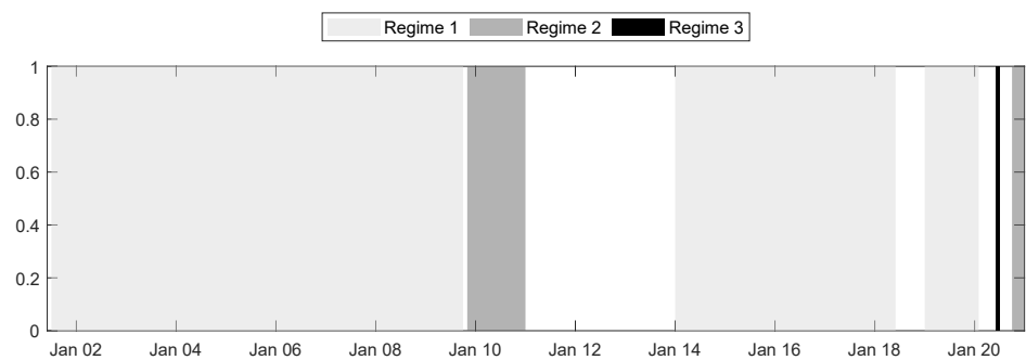
(b) Robustness 2
