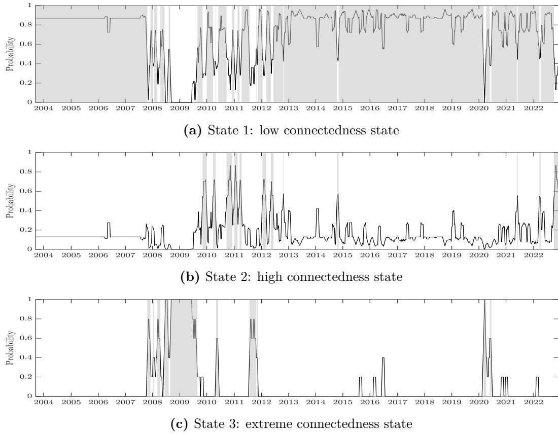
Figure 2.1 Estimated states. We present the mean posterior smoothed probability of the low (panel (a)), high (panel (b)) and extreme (panel (c)) connectedness states. Gray bars in each plot correspond to the periods where the probability of the corresponding state is the maximum. Model-implied turning points of the high and extreme connectedness states: 1) the high connectedness state (month/year): 11/09-12/09; 04/10; 09/10-11/10; 01/11; 03/11; 01/12-02/12; 05/12; 10/12; 10/14; 06/21; 03/22-04/22; 10/22-12/22. 2) the extreme connectedness state (month/year): 10/07-11/07; 01/08; 03/08-04/08; 06/08-07/08; 09/08-08/09; 05/10; 08/11-11/11; 03/20; 06/20. See the Internet Appendix D for discussions of the turning points.
