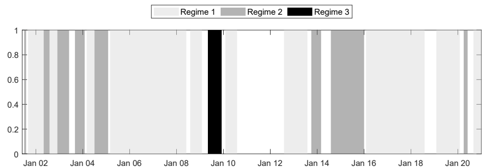
(a) Robustness 1
