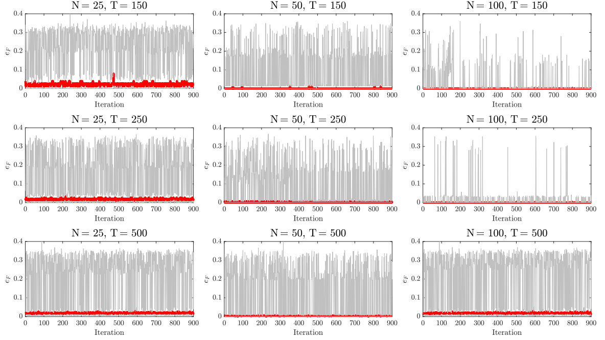
Figure 3.B.9 DGP 3 (WHeF + WS). The median (red line) and 10th and 90th quantile (grey line) values of the estimation error e_F computed through MCMC iterations from successful experiments that detect the true regime dimension of the panel.
