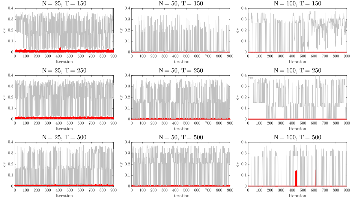
Figure 3.B.10 DGP 4 (WHeF + WSSS). The median (red line) and 10th and 90th quantile (grey line) values of the estimation error e_F computed through MCMC iterations from successful experiments that detect the true regime dimension of the panel.
