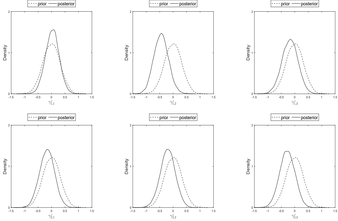
Figure 1.1 Prior-posterior distributions of the parameters \gamma_{i,s_{t-1}}^z . This figure plots the marginal posterior distributions (solid line) of the parameters \gamma_{i,s_{t-1}}^z , where i = 1, 2 and s_{t-1} = 1, 2, 3 , against their prior distributions (dashed line) for the selected model \mathcal{M}_{3,N=3} , i.e., the three-regime timing model in equation (1.16). Results are based on 12,500 MCMC iterations.
