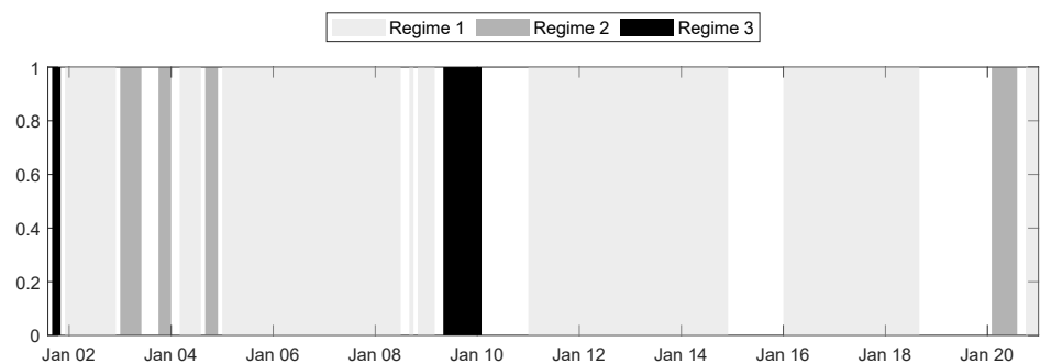
(c) Robustness 3
