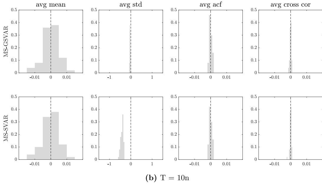
Figure 2.C.10 Posterior predictive checking based on 50 replications for the MS-GSVAR model (first row) and the MS-SVAR model (second row). Performance on a simulated dataset of dimension n = 80 , with two different sample sizes T = 5n (panel (a)), = 10n (panel (b)). Each plot shows the posterior distribution of the discrepancy between the test quantity computed on the simulated and the observed data, averaged over all MCMC iterations for each replication.
