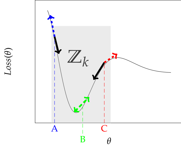
FIGURE 12.1: CSUD behaviour with a single input loss function L(\theta) . \mathbb{Z}_k indicates the constraint zone. At point A , the dashed blue line indicates that a double sided perturbation would violate the constraint. Accordingly, to remain in the constraint zone \mathbb{Z}_k , a single-sided gradient in the opposite direction, indicated by the solid black line is calculated. Point C is evaluated similarly. At point B , the constraint \mathbb{Z}_k is not binding, and a double sided perturbation is used in approximating the gradient.
