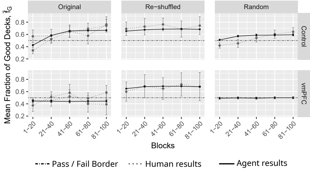
FIGURE 6.4: \epsilon -Greedy Agent 20-draw blocks comparison at CSUD search matches \alpha_1 = 0.417 , \lambda_N = 0.104 , \lambda_{vmPFC} = 0.449 , \epsilon = 0.627 . Human results in light gray. Agent results in dark gray, averaged from 750 samples. All error bars at \pm 2SE . When error bars are taken into account agent and human 20-draw block performance appears relatively similar. Details in text below.
