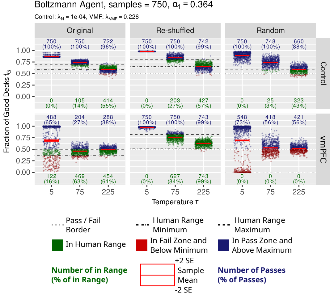
FIGURE 6.12: Boltzmann agent comparison of repeated simulation outcomes to human IGT results. At \tau = 225 and reported CSUD minimum loss hyper-parameter values, the Boltzmann agent achieves the highest matches for the re-shuffled IGT environment. Full details are in the text.
