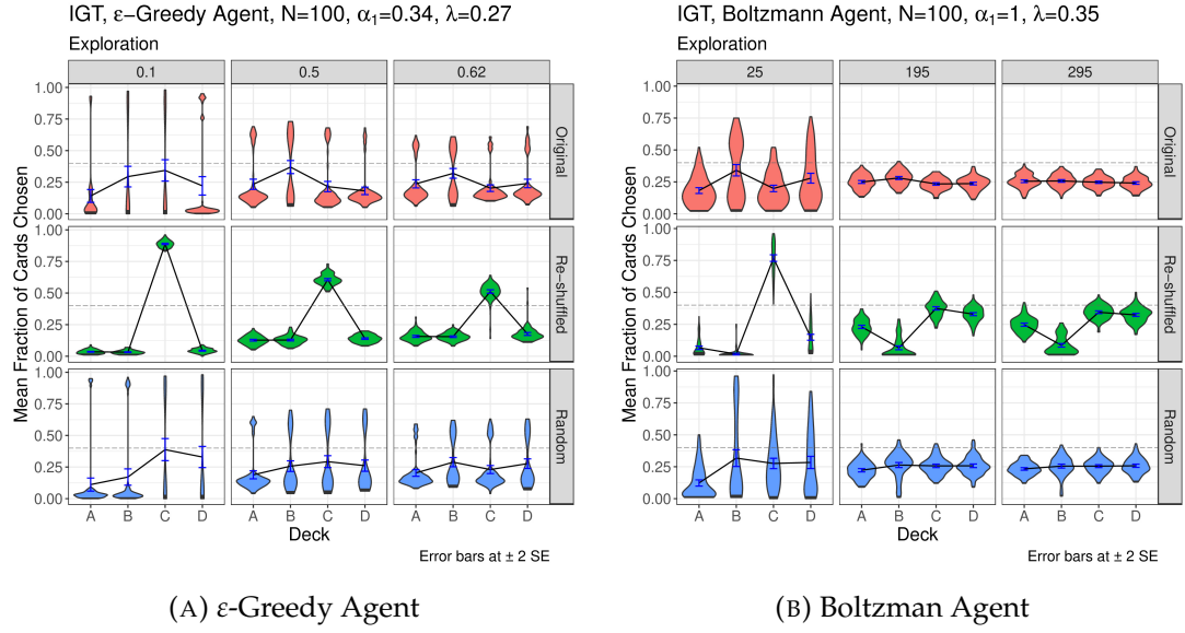
FIGURE B.2: vmPFC Impaired agents deck looping versus exploration at mean fraction of cards per deck at 100 th draw. The dashed line represents the 40 th card. In general, as exploration increases, deck looping decreases on average, but especially for the \epsilon -Greedy case, some agents continue to loop. As expected from the soft-max constraint, Boltzmann agent violin plots approximate a uni-modal symmetric distribution, while \epsilon -Greedy agent violin plots tend to bi-modality and skewness for most decks and IGT variants.
