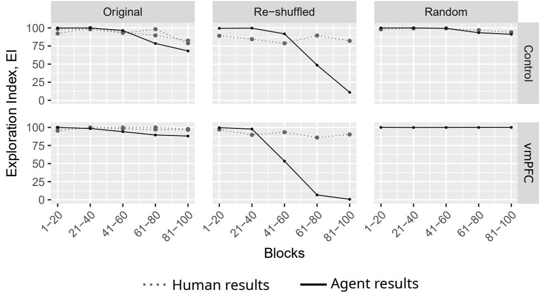
FIGURE 6.18: Adaptive \epsilon -Greedy agent 20-draw blocks exploration index (EI) comparison at CSUD search matches \alpha_1 = 0.591 , \lambda_N = 0.082 , \lambda_{vmPFC} = 0.120 , \tau = 0.383 . Human results in dotted light gray lines. 4 Agent results in solid dark gray lines, averaged from 750 samples. Human subject and agent exploration index responses show comparative differences especially for the re-shuffled IGT environment. Details in text below.
