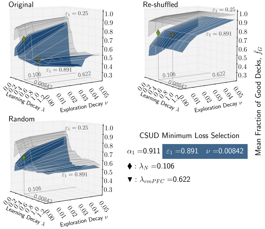
FIGURE 6.23: Decaying \varepsilon -Greedy agent 3D contours with learning decay \lambda , exploration decay \nu , and initial exploration \varepsilon_1 at initial learning rate \alpha_1 = 0.911 . Both learning decay and exploration decay show \bar{f}_G influences in all IGT environments. However, learning decay shows a stronger effect.
