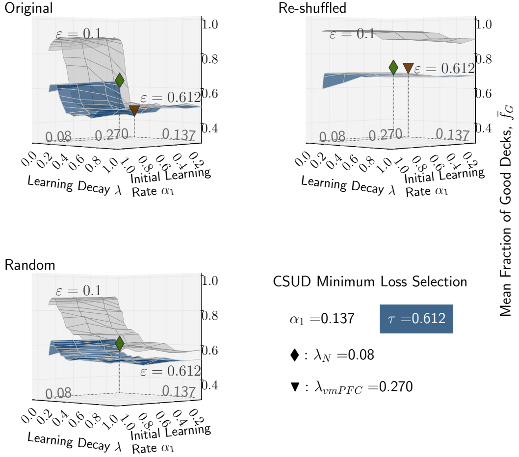
FIGURE 9.4: ARA( \kappa ) \epsilon -Greedy Agent, \gamma = 0.514 , \kappa = 0.264 , CSUD search grid verification 3D contours. Blue coloured surfaces show response to learning decay \lambda at CSUD selected minimum loss hyper-parameter values. The diamond and inverted triangular shapes mark CSUD minimum loss normal and vmPFC impaired learning decay rates respectively.
