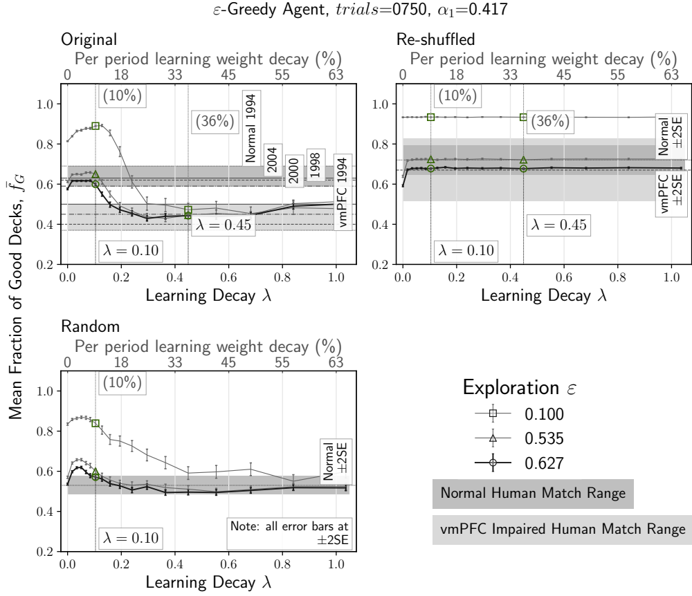
FIGURE 6.2: \varepsilon -Greedy agent 2D contours showing learning decay \lambda and exploration \varepsilon effects. The dark and light gray zones indicate normal and vmPFC impaired human outcome match ranges for the original, re-shuffled, and random IGT environments. Learning decay variation reproduces human IGT outcomes, while exploration variation is responsible for matching human IGT outcome performance ranges.
