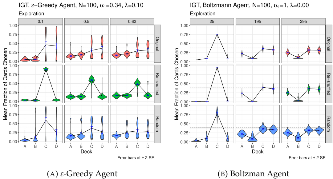
FIGURE B.1: Normal agents deck looping versus exploration at mean fraction of cards per deck at 100 th draw. The dashed line represents the 40 th card. In general, as exploration increases, deck looping decreases on average, but especially for the \epsilon -Greedy case, some agents continue to loop. As expected from the soft-max constraint, Boltzmann agent violin plots approximate a unimodal symmetric distribution, while \epsilon -Greedy agent violin plots tend to bi-modality and skewness for most decks and IGT variants.
