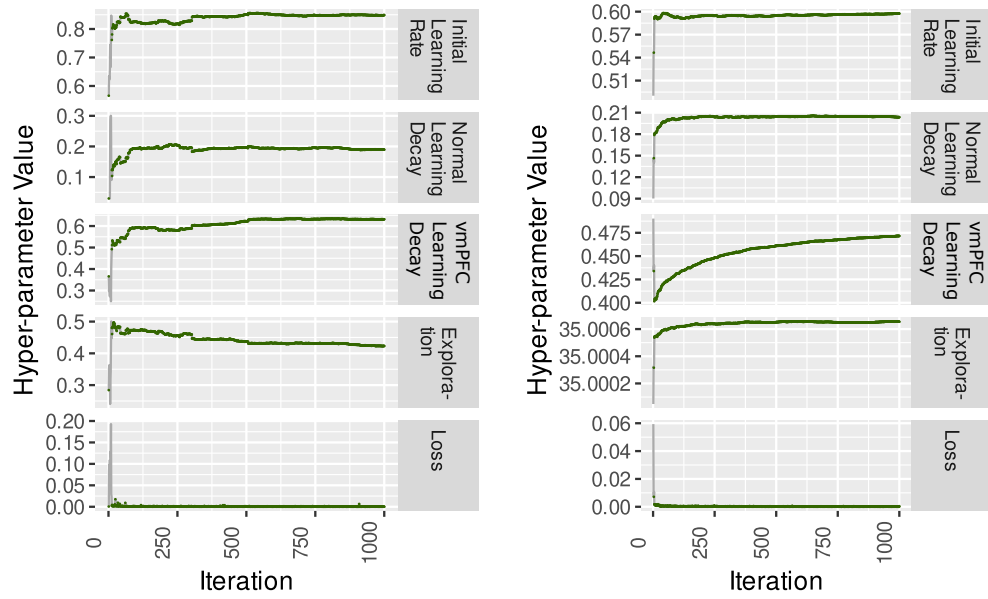
(A) \epsilon -Greedy Agent, 990 matches
