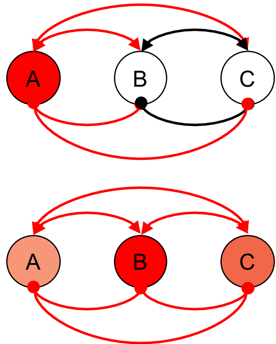
Fig. 1. After an (external) activation of the neuron A (top), excitatory connections as well as external input to B will activate both B and C (bottom). Depending on the balance of excitation and inhibition between A and C , the net input on from C to A might thus be inhibitory on the next time step.
