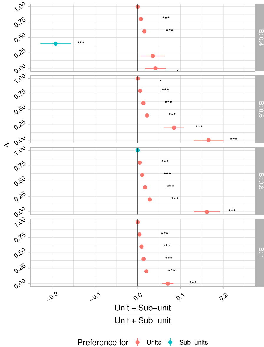
Fig. 2. Normalized average difference scores of network activations after presentation of entire two-syllable units and different types of two-syllable units (i.e., AB and BC from ABC units), as a function of the forgetting rate (y axis) and the interference rate (facets in rows). As in Giroux and Rey (2009) , we do not separate AB and BC sub-units. Positive values indicate stronger activations for units. Significance stars reflect a Wilcoxon test against the chance level of zero. Units generally elicit greater activation compared to the average of AB and BC sub-units. Significance labels: ***: \leq 0.001 ; **: \leq 0.01 ; *: \leq 0.05 ; .: \leq 0.1 .
