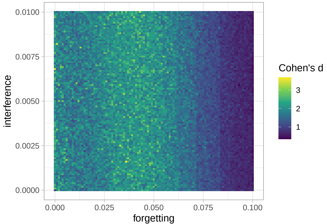
Figure S4. Effect sizes (Cohen's d ) of the preference for words over part-words in simulations with PARSER as a function of the forgetting rate and the interference rate. All simulated experiments yielded a significant preference for words.
