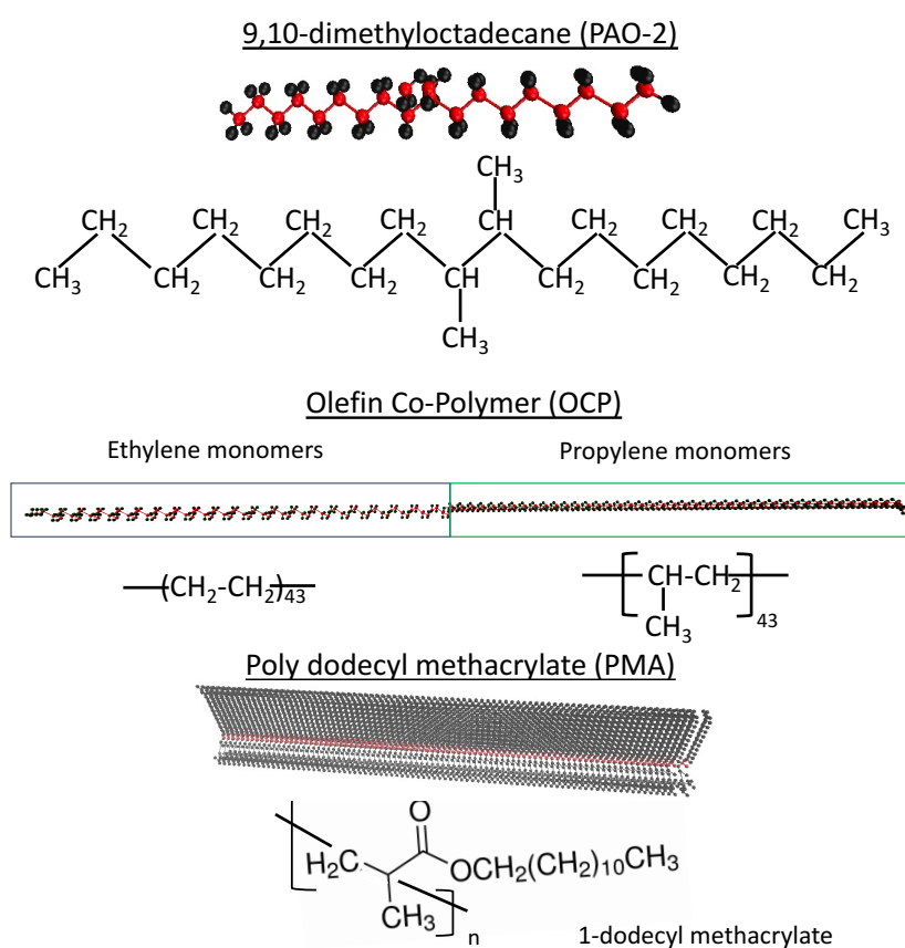
Figure B1: Schematics of the solvent - PAO-2 molecule, and polymer chains - OCP molecule and PMA molecule used in this simulation study.
