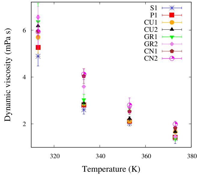
Figure 4.5: Zero-shear dynamic viscosity of the simulated fluids as a function of temperature.
