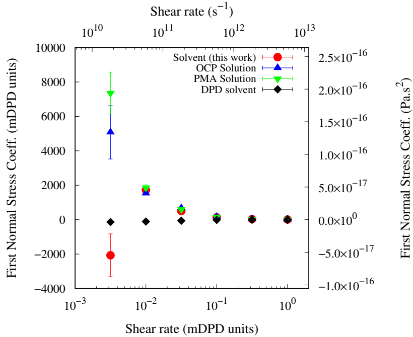
Figure 3.10: First normal stress coefficient, \psi_1 as a function of shear rate, \dot{\gamma} at 313 K computed by mesoscale simulations. DPD solvent has \rho = 7.9 (mDPD units).
