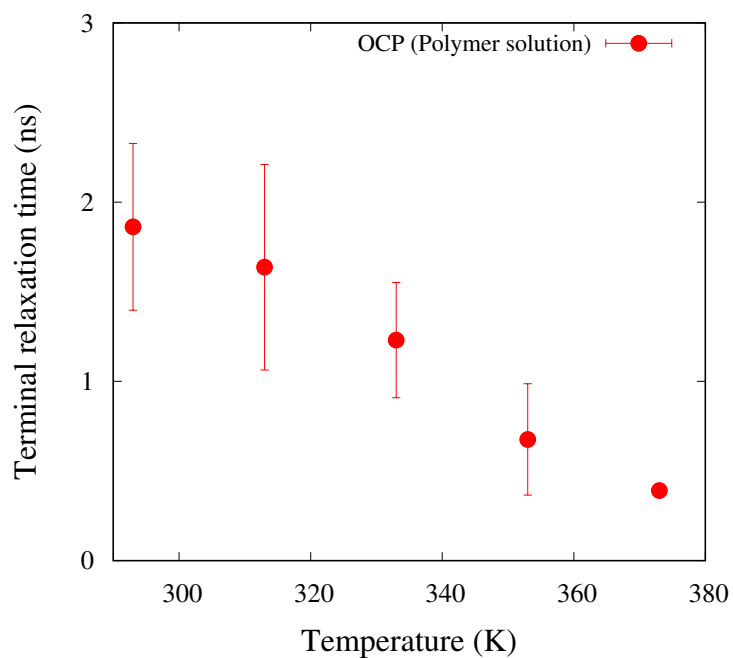
Figure B3: Terminal relaxation time of OCP polymer chain as a function of temperature, T in the atomistic scale simulations.
