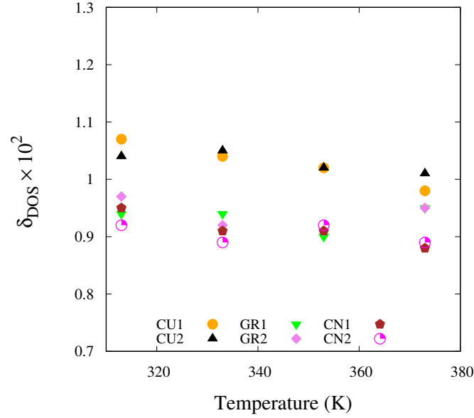
Figure 4.8: \delta_{\text{DOS}} of the simulated nanofluids as a function of temperature.
