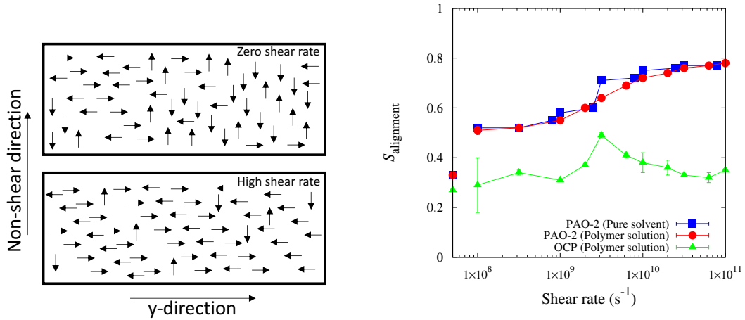
Figure 2.6: (Left) The schematic of molecular alignment in the absence and presence of shear. (Right) S_{\text{alignment}} of PAO-2 and OCP molecules in pure solvent and polymer solution as a function of shear rate at 313 K. The data points on the y-axis show the values of S_{\text{alignment}} at zero shear rate.
