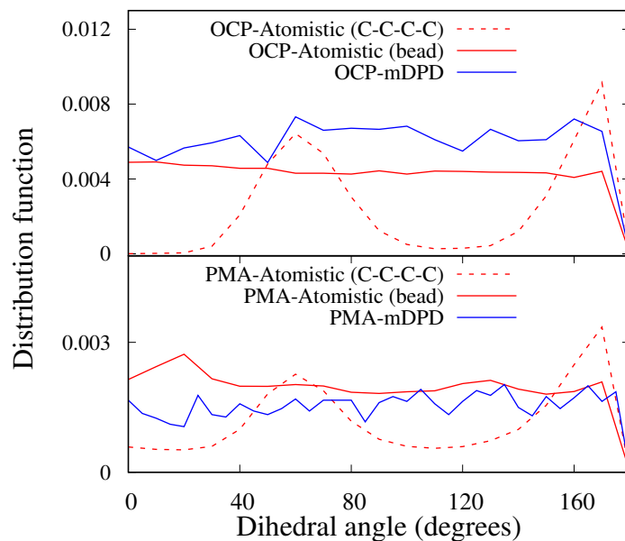
Figure B6: Dihedral distribution function of polymer chains in OCP solution (top) and PMA solution (bottom) at 313 K in the atomistic scale and mesoscale simulations. Under atomistic scale, the red dashed lines show the atomistic dihedral distribution between carbon atoms, and the red solid lines show the distribution of the dihedral angle of center of bonded beads as depicted in Figure 3.4b in Chapter 3.
