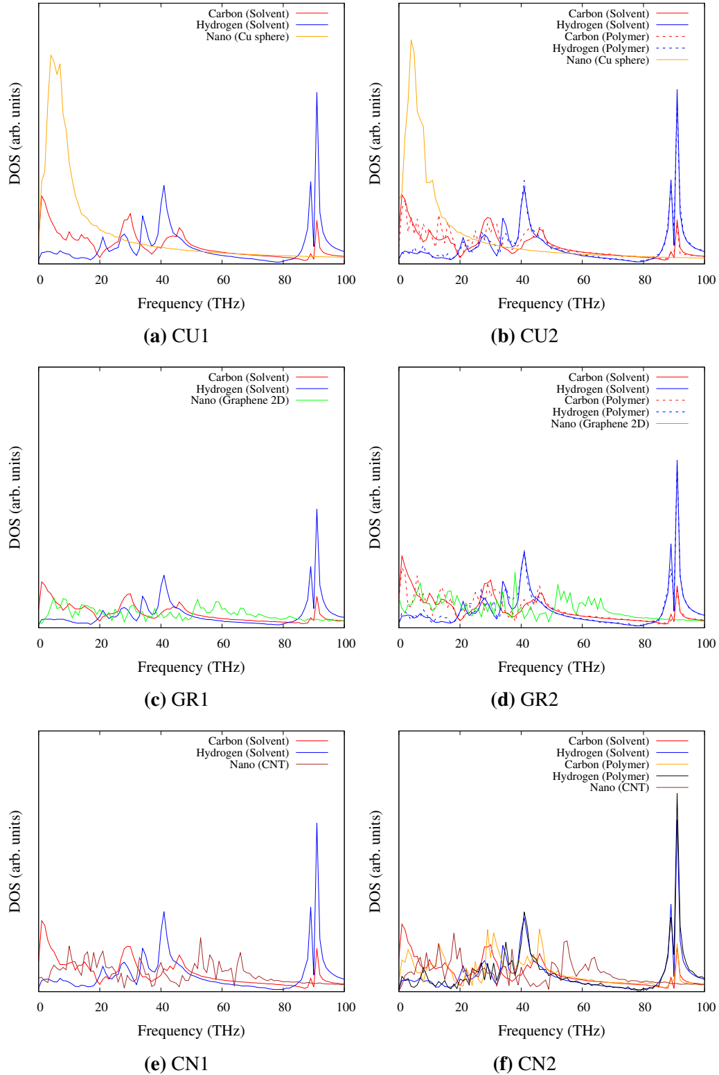
Figure 4.7: The phonon vibrational density of states (DOS) of the different nanofluids at 313 K.
