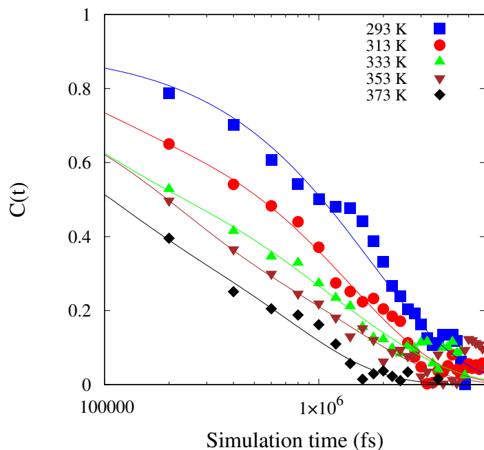
Figure A8: The end-to-end vector autocorrelation ( C(t) ) of OCP as a function of simulation time for a single simulation run of polymer solution at different temperatures. The closed symbols show the simulated C(t) values. The lines show the a fit of a sum of exponential function as described by Equation 2.18 in Chapter 2.
