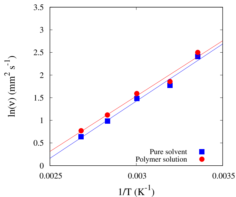
Figure A3: The kinematic viscosity ( v_0 ) of the pure solvent system and polymer solution as a function of temperature. The closed symbols show the simulated values - blue (pure solvent) and red (polymer solution). The lines show the Arrhenius fit as described in Equation 2.6 in Chapter 2.
