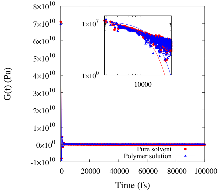
Figure A6: G(t) as a function of simulation time for pure solvent and polymer solution systems at 313 K. Inset shows G(t) values (points) smoothened by doing a running average between 0.9t and 1.1t as described by Sen et al. [200], and their corresponding fits (lines) of Equation 2.13 in Chapter 2.
