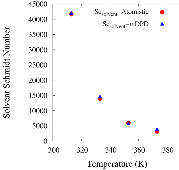
Figure 3.5: Schmidt number of solvent, Sc_{\text{solvent}} as a function of temperature, T .
