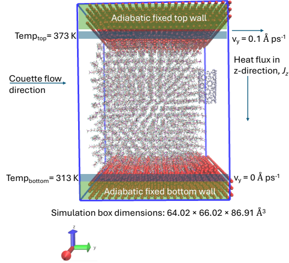
Figure 4.1: Simulation box of nanofluid CN1 after the energy minimisation step. Atoms in red at the top and bottom represent Fe atoms.
