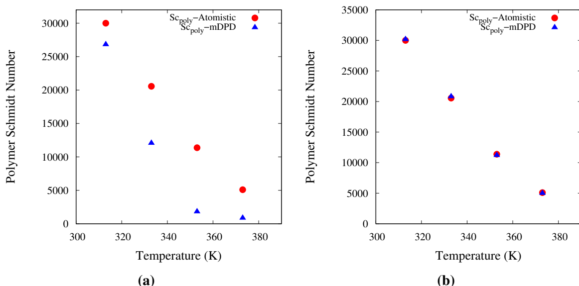
Figure 3.6: Comparison of OCP polymer Schmidt number ( Sc_{poly} ) as a function of temperature: (a) Different concentrations simulated in atomistic MD (5.9% by weight) and mDPD (0.001% by weight). (b) Same concentration simulated in atomistic MD and mDPD (5.9% by weight).
