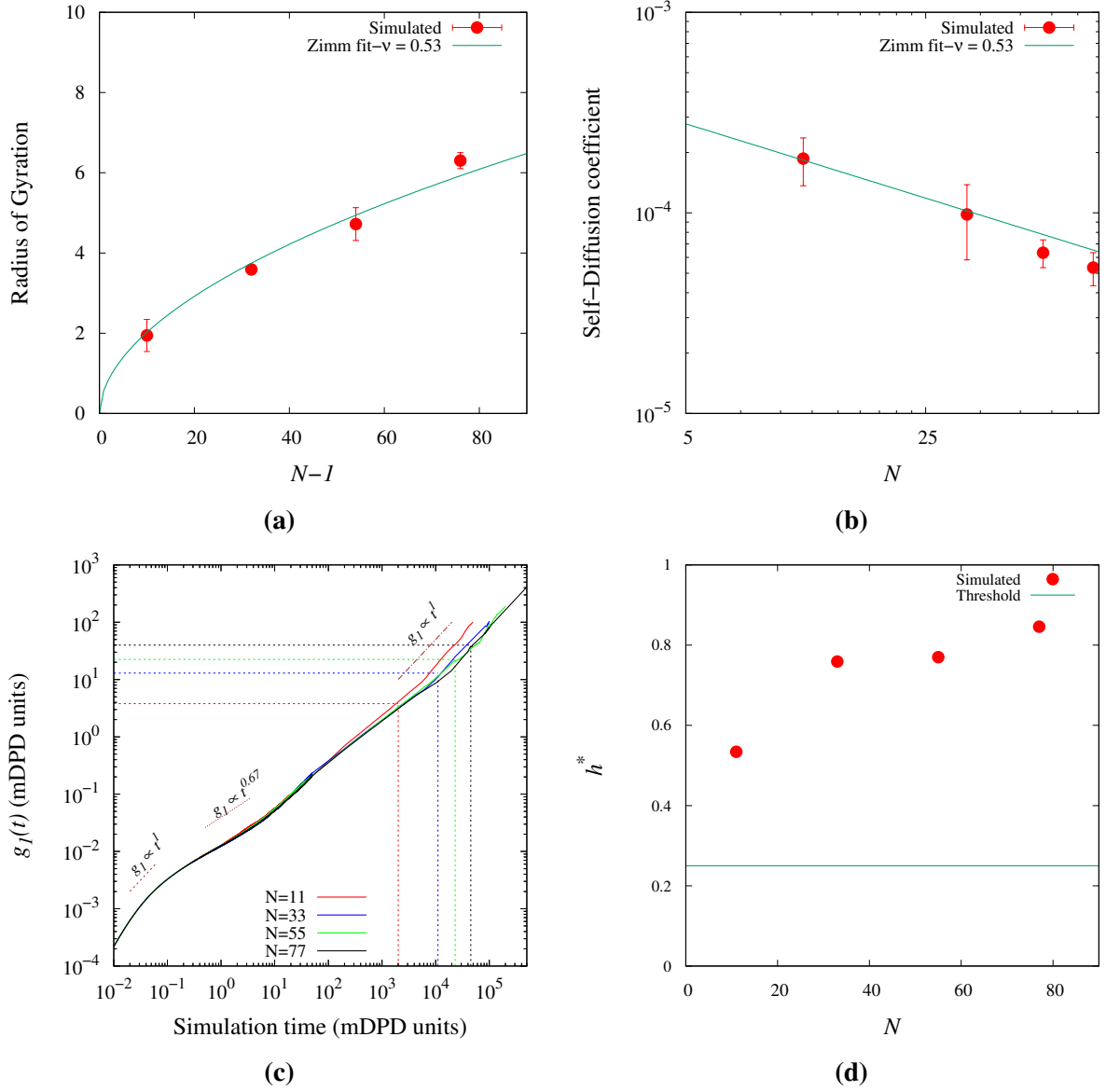
Figure 3.3: (a) Radius of gyration of OCP polymer chain as a function of chain length, N - 1 at T = 313 K. (b) The self-diffusion coefficient of the OCP polymer chain as a function of chain length, N at T = 313 K. (c) g_1(t) as a function of time showcasing different regimes for different chain lengths. Here, the horizontal dashed lines show the value of R_g^2 and the vertical dashed lines show the corresponding values of \tau_z for different values of N . (d) h^* as a function of chain length, N at a temperature, T = 313 K.
