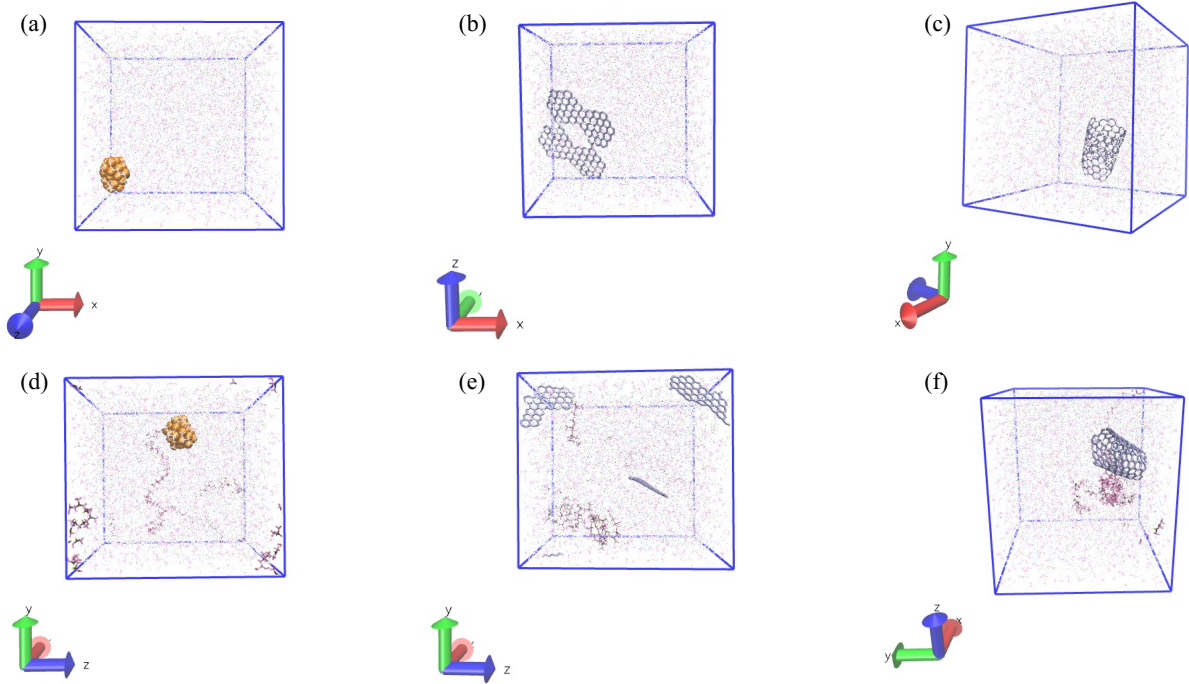
Figure 4.2: Simulation box of nanofluids (a) CU1, (b) GR1, (c) CN1, (d) CU2, (e) GR2, (f) CN2 at the end of the NPT equilibration run at 313 K. The orange coloured atoms represent Cu in (a) and (d). The purple coloured atoms represent 2D graphene in (b) and (e), and CNT in (c) and (f). The pink atoms represent OCP polymer chain in (d), (e) and (f). The translucent atoms represent PAO-2 solvent in all the simulation boxes.
