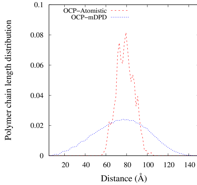
Figure B4: Polymer chain length distribution for OCP at 313 K in atomistic MD and mDPD.
