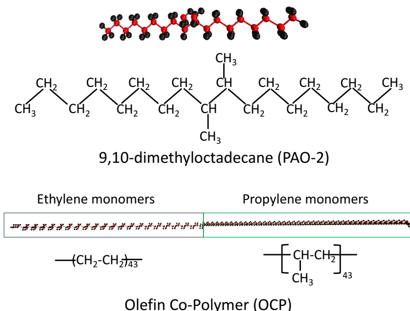
Figure 2.1: Schematics of the solvent - PAO-2 molecule and polymer chain - OCP molecule used in this simulation study.
