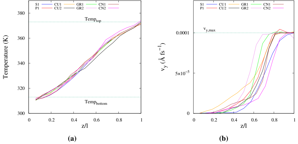
Figure 4.9: (a) The temperature profile in the z -direction during the Couette flow of the different simulated fluids. (b) The velocity profile of the simulated fluids in the y -direction as a function of dimensionless distance with z/l = 0 representing the bottommost layer of the fluid and z/l = 1.0 representing topmost layer of the fluid. Here, v_{y,max} = 0.1 \text{\AA ps}^{-1} = 0.0001 \text{\AA fs}^{-1} , Temp_{top} = 373K , and Temp_{bottom} = 313K .
