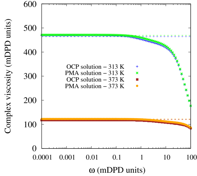
Figure B8: Complex viscosity ( \eta^*(\omega) ) as a function of \omega for the OCP and PMA polymer solutions at 313 K and 373 K. The values agree with the \eta_0 from Green-Kubo equation [188].
