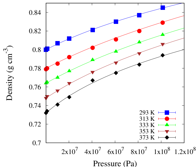
Figure A2: The density ( \rho ) of pure solvent (PAO-2) as a function of pressure at different temperatures. The points show the simulated data, and the lines show the modified Tait equation fit as described in Equation 2.2 in Chapter 2.
