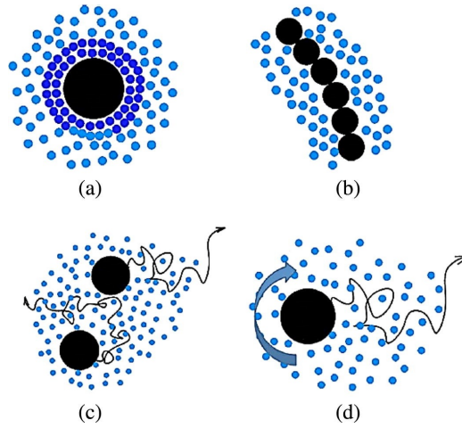
Figure 1.3: Thermal performance enhancement mechanisms in the nanofluids. The nanoparticles are depicted by black spheres and solvent molecules are depicted by blue spheres. The different mechanisms are (a) liquid layering; (b) particle aggregation; (c) particle Brownian motion and (d) Brownian motion induced convection. Figure reproduced from Reference [15] with permission. Copyright 2011, The Americal Society of Mechanical Engineers.
