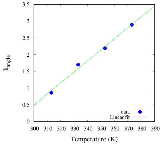
Figure B5: k_{angle} as a function of temperature, T for PMA.
