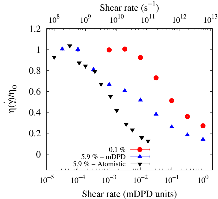
Figure 3.14: The ratio of shear viscosity, \eta(\dot{\gamma})/\eta_0 as a function of shear rate, \dot{\gamma} at 313 K for OCP polymer solution with polymer concentrations of 0.1 % and 5.9% by weight.
