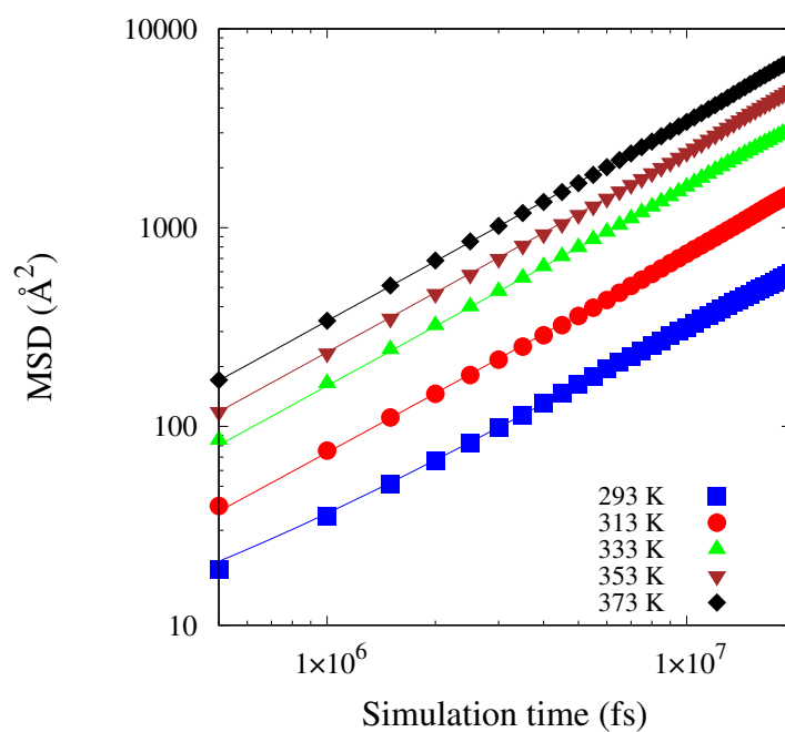
Figure A4: Mean squared displacement (MSD) of the PAO-2 molecules in pure solvent system as a function of simulation time for a single simulation run at different temperatures using multiple time origins. The closed symbols show the simulated MSD values. The lines show the fits of linear functions whose slope is used to compute the centre of mass self-diffusion coefficient, D_{\text{COM}} .
