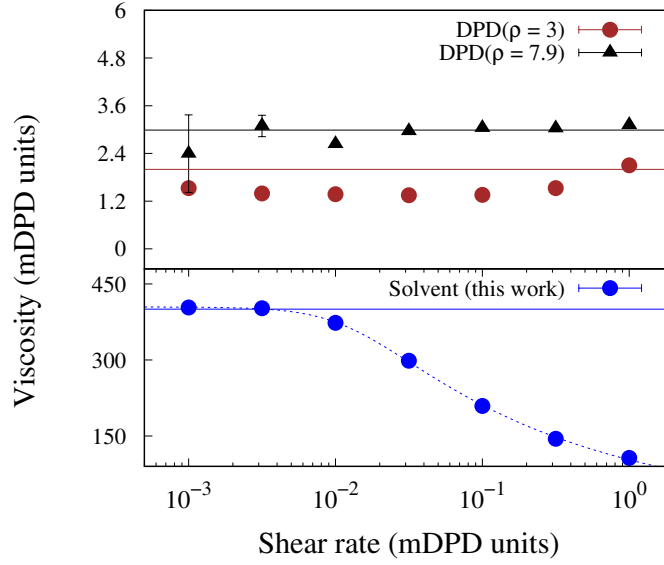
Figure 3.8: Shear viscosity, \eta as a function of shear rate, \dot{\gamma} for solvent molecules computed in the mesoscale simulations. The horizontal lines show the zero-shear viscosity computed using Green-Kubo method under equilibrium conditions and the dashed line shows the Carreau-model fit.
