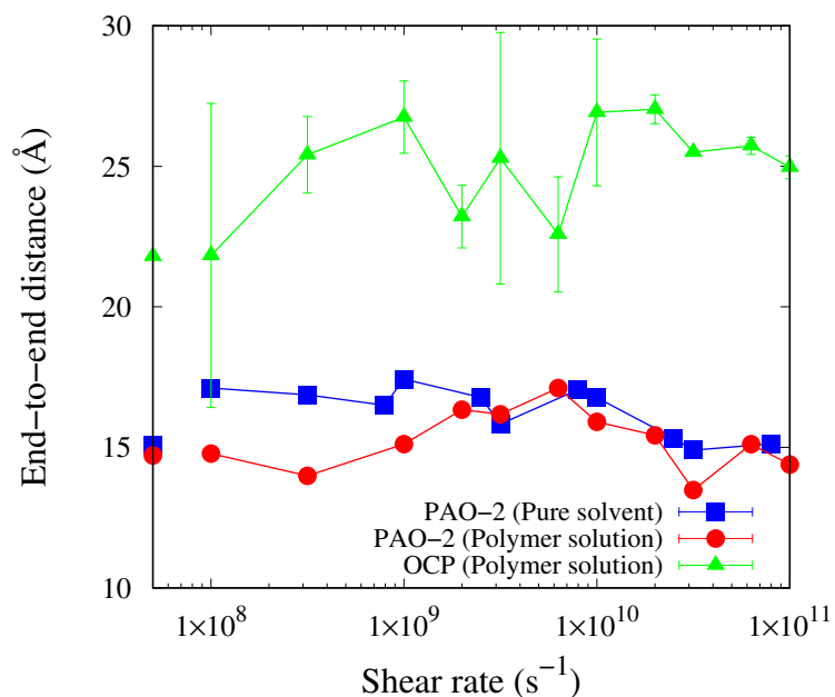
Figure A7: The end-to-end distance ( R_e ) of PAO-2 and OCP in pure solvent and polymer solution as a function of shear rate at 313 K. The data points on the y-axis show the values of R_e at zero shear rate. The data shows that R_e of OCP increases as a function of shear rate whereas that of PAO-2 remains constant.
