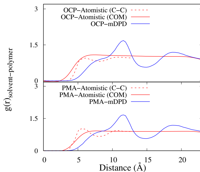
Figure B7: The radial distribution function ( g(r)_{\text{solvent-polymer}} ) between solvent and polymer beads in OCP solution (top) and PMA solution (bottom) at 313 K in the atomistic scale and mesoscale simulations. Under atomistic scale, the red dashed lines show the g(r) between the carbon atoms of the solvent and polymer molecules, whereas the red solid lines show the g(r) between the centre of mass (COM) of solvent bead and polymer chain beads equivalent to that in the mesoscale simulation. Mesoscale model shows more structural ordering than the atomistic scale model while comparing the blue and red solid lines.
