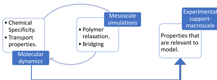
Figure 1.6: Schematic of the objectives of the research.
