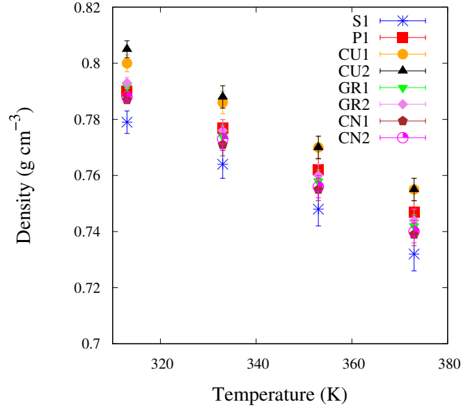
Figure 4.3: Density of the simulated fluids as a function of temperature.
