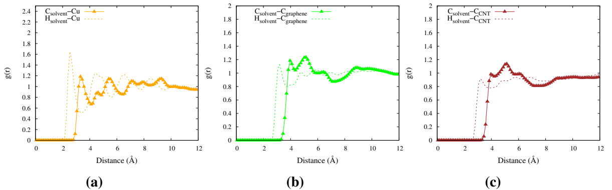
Figure 4.4: Radial distribution functions, (a) g_{C_{\text{solvent}}, Cu}(r) in CU1, (b) g_{C_{\text{solvent}}, C_{\text{graphene}}}(r) in GR1 and (c) g_{C_{\text{solvent}}, C_{\text{CNT}}}(r) in CN1 at 313 K.
