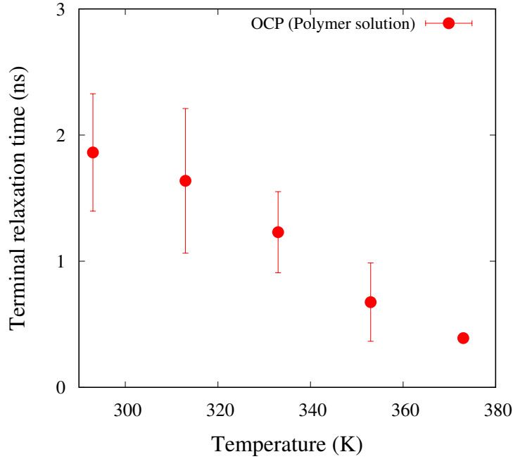
Figure 2.7: The terminal relaxation time ( \tau_{term} ) of OCP in the polymer solution as a function of temperature.
