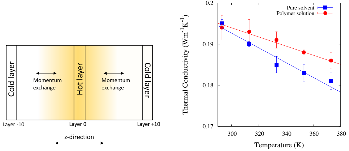
Figure 2.9: (Left) The schematic of reverse-NEMD applied in case of the present simulation study. (Right) The thermal conductivity ( k ) of the pure solvent and polymer solution as a function of temperature. The closed symbols show the simulated data and the lines show the linear function fits as described in Equation 2.21.
