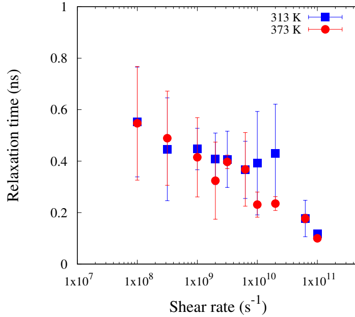
Figure 2.8: The terminal relaxation time ( \tau_{term} ) of OCP in the polymer solution as a function of shear rate at two different temperatures (313 K and 373 K).
