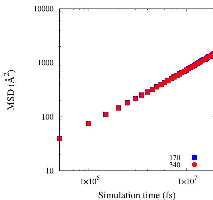
Figure A5: MSD of the PAO-2 molecules in pure solvent as a function of simulation time for a single simulation run at 313 K using multiple time origins. The closed symbols show the simulated values - blue (170 molecules) and red (340 molecules). The computed MSD shows that it is independent of the system size and the trajectories evolve similarly over time.
