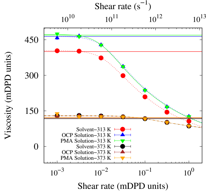
Figure 3.9: Shear viscosity, \eta as a function of shear rate, \dot{\gamma} at 313 K and 373 K in the mesoscale simulations. The horizontal lines show the zero-shear viscosity computed using Green-Kubo method under equilibrium conditions. The dashed and dash-dotted lines show the Carreau-model fit.
