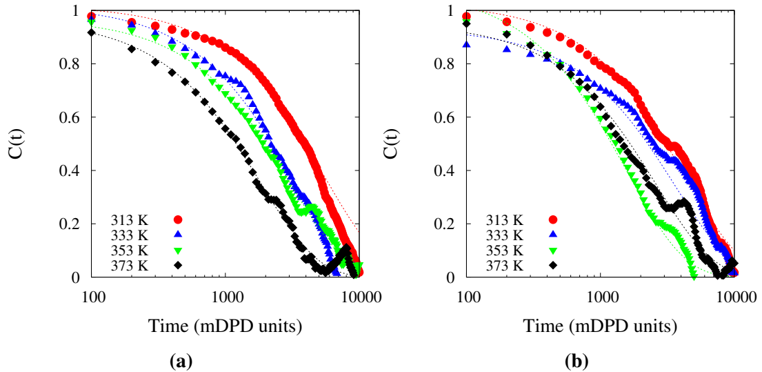
Figure B9: C(t) as a function of time for (a) OCP polymer chain and (b) PMA polymer chain at different temperatures. The dashed lines show the exponential fit.
