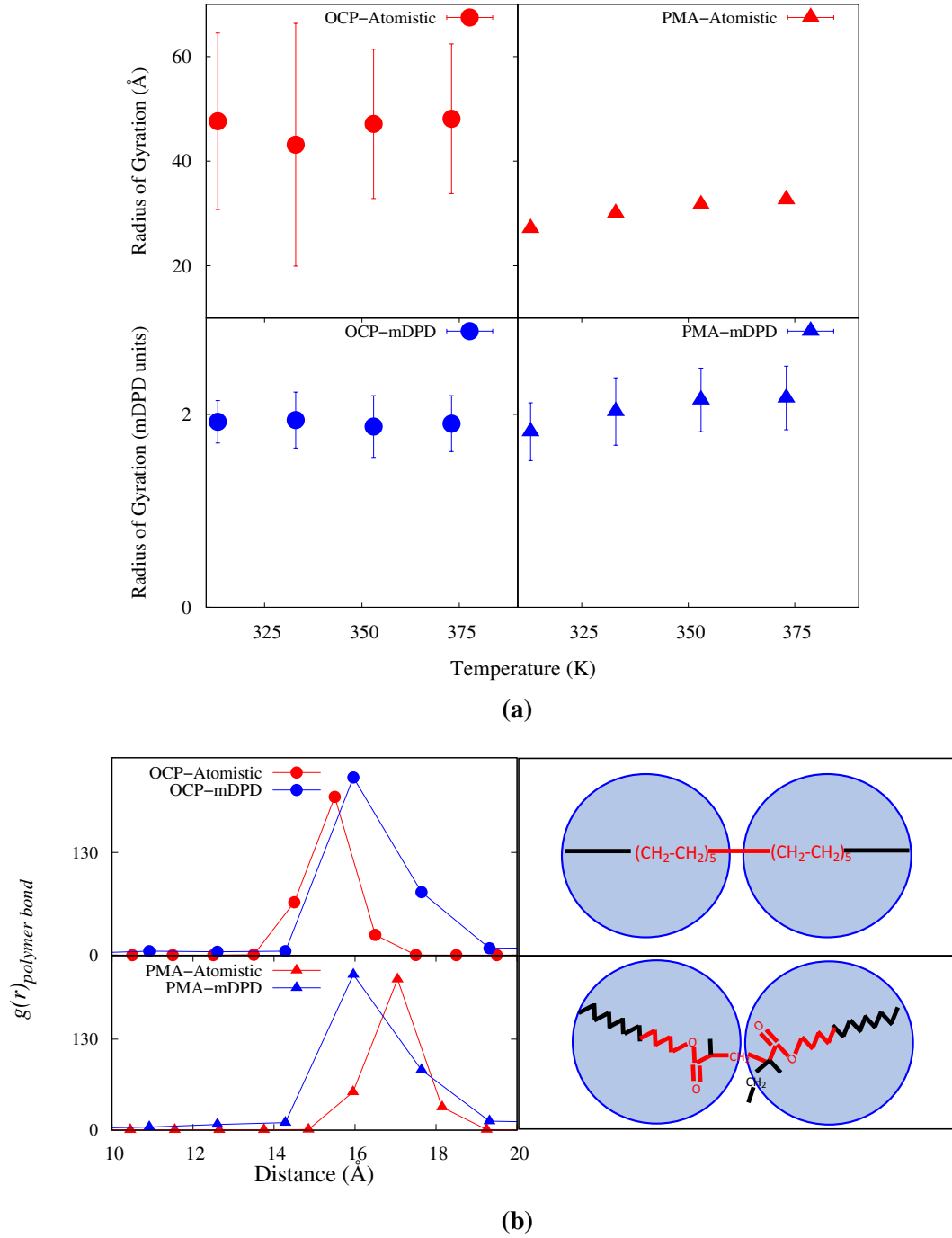
Figure 3.4: (a) Radius of gyration as a function of temperature, T for OCP and PMA solutions in atomistic and mDPD simulations. (b) Intramolecular bond distribution of OCP and PMA polymer chains at 313 K in the atomistic and mDPD simulations. The schematic here compares the equivalent bonded distance of the beads in mesoscale with that in atomistic scale.
