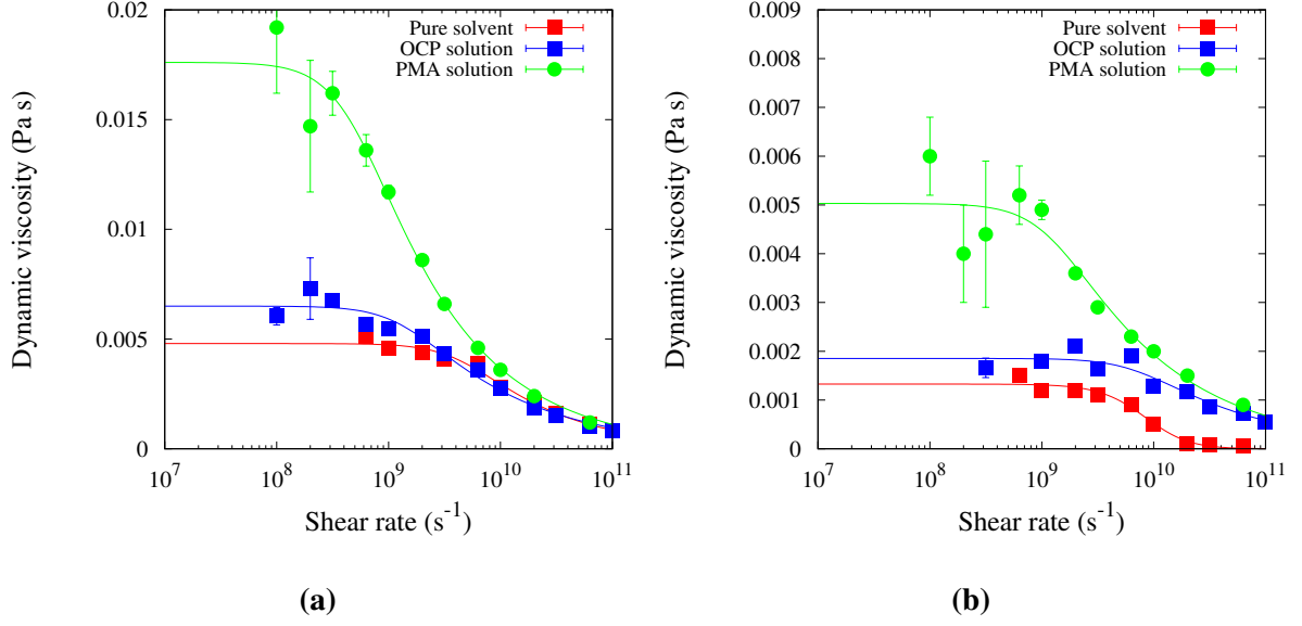
Figure 3.7: Viscosity ( \eta(\dot{\gamma}) ) as a function of shear rate ( \dot{\gamma} ) at (a) 313 K and (b) 373 K for pure solvent and polymer solution systems simulated via atomistic MD. The symbols with the error bars show the simulated dynamic viscosity values, \eta(\dot{\gamma}) at different shear rates, \dot{\gamma} . The lines depict the Carreau-model fittings.
