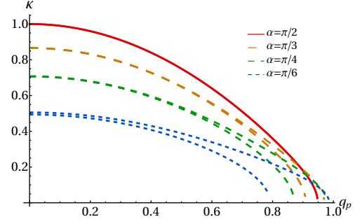
Figure 8. Inverse penetration depth of surface states as a function of the transverse momentum for L = 10 and various values of the boundary angle.
