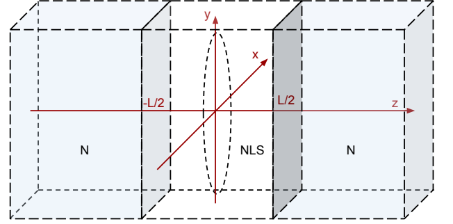
Figure 9. Scheme of a N-NLS-N junction, infinitely extended in the x and y directions. The metallic leads are at z < -L/2 and z > L/2 and the nodal line is in the plane parallel to the interfaces.
