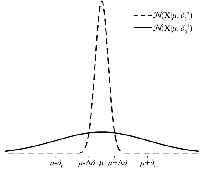
Figure 7. Illustration of the mixture of Gaussian distributions in Equation (6) for vessel matching. The two Gaussian distributions centre on the same mean \mu = f_j(s, t, \theta) but have different standard deviations satisfying \delta_1 \ll \delta_0 . The two Gaussian distributions intercept at two points that are \Delta\delta from \mu .
