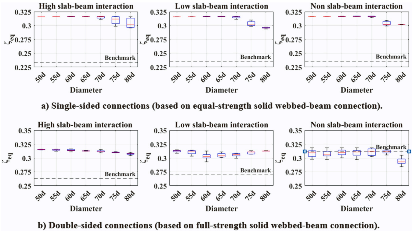
Fig. 18. Equivalent viscous damping coefficient at 0.04 rad, the benchmark = the connection with solid webbed-beam (without web opening).
