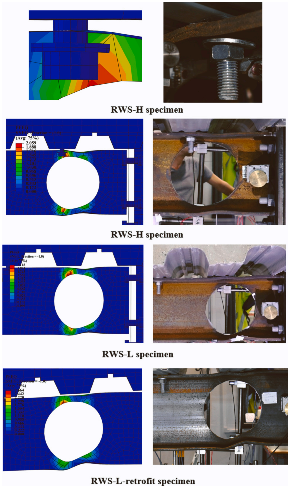
Fig. 10. Comparison between FE models and tested specimens [7] (without rendering the thickness of shell element).
