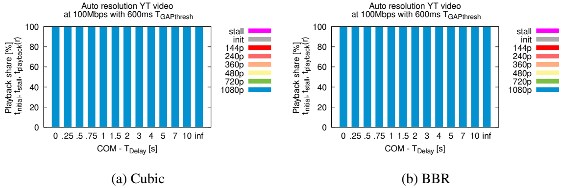
Fig. 5.18 QoE parameters of adaptive resolution YT video at 100 Mbps DSL rate, t_{GAPthres} = 600\text{ms} , t_{nottraffic} = 50\text{ms} and V_{max} = 100\text{pkts}
