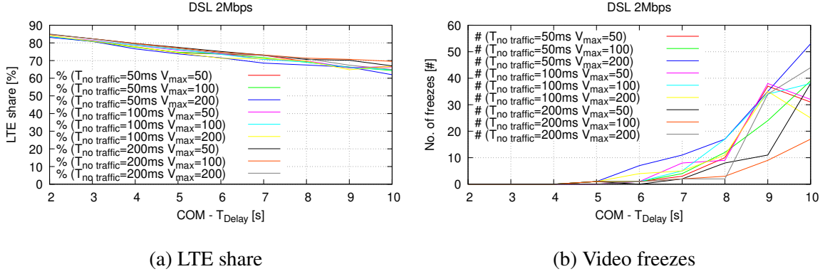
Fig. 5.7 LTE share and video freezes for variable t_{notraffic} and V_{max} at 2 Mbps DSL rate and t_{GAPthresh} = 600\text{ms}
