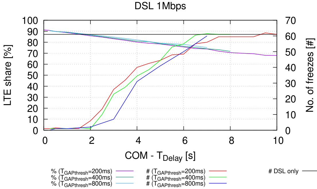
Fig. 5.3 LTE share and video freezes for variable t_{GAPthresh} at 1 Mbps DSL rate, t_{notraffic} = 50\text{ms} and V_{max} = 100\text{pkts}
