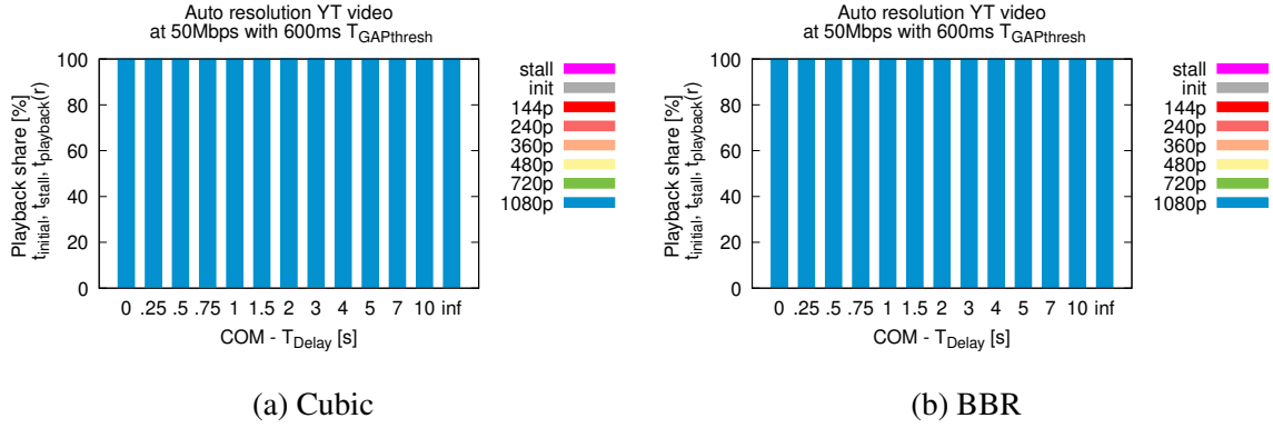
Fig. 5.17 QoE parameters of adaptive resolution YT video at 50 Mbps DSL rate, t_{GAPthres} = 600\text{ms} , t_{nottraffic} = 50\text{ms} and V_{max} = 100\text{pkts}
