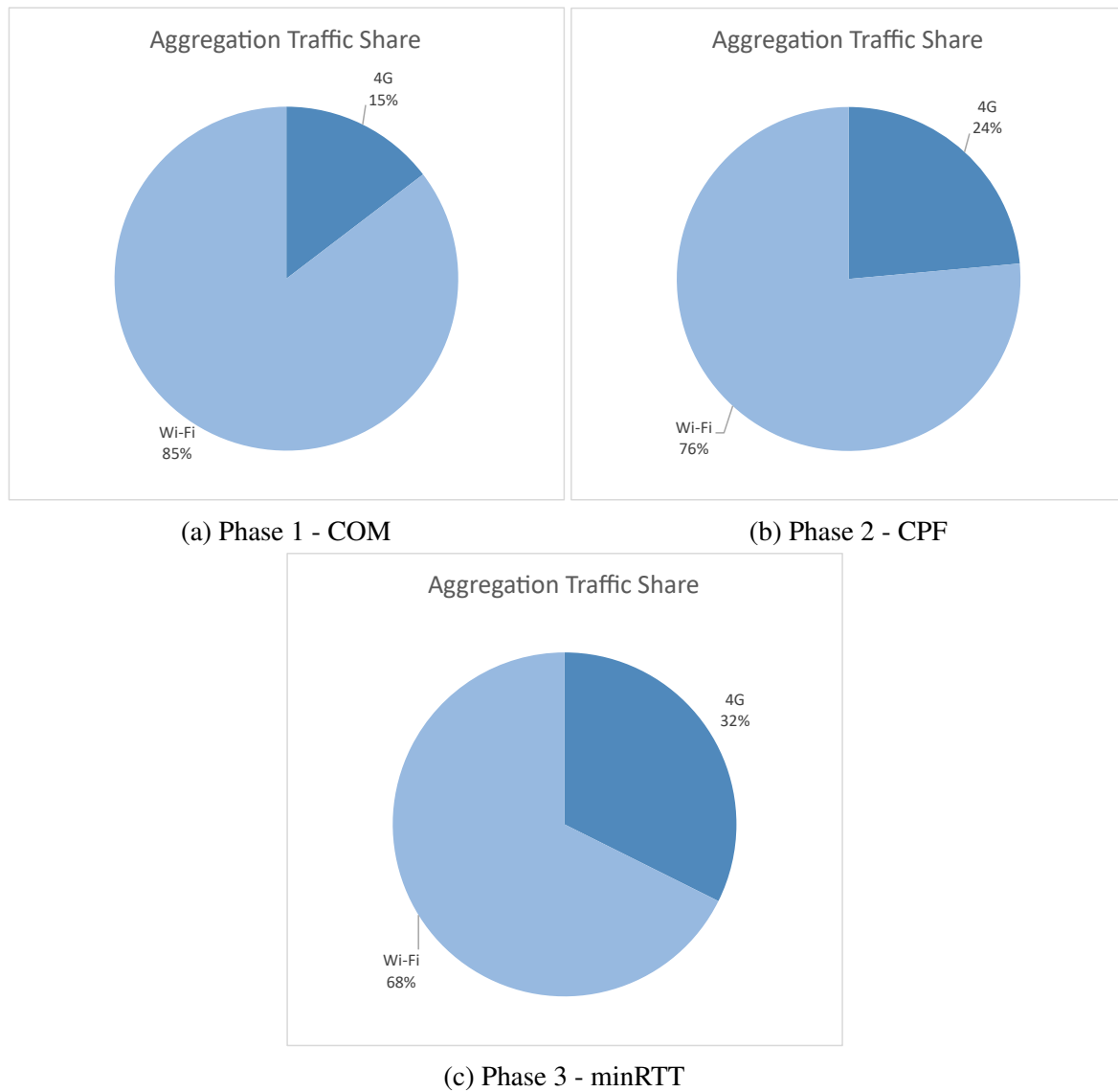
Fig. 5.26 Percentage distribution of data traffic across all trial participants if the combination of Wi-Fi and LTE allows MPTCP traffic to be split, separated according to the phases
