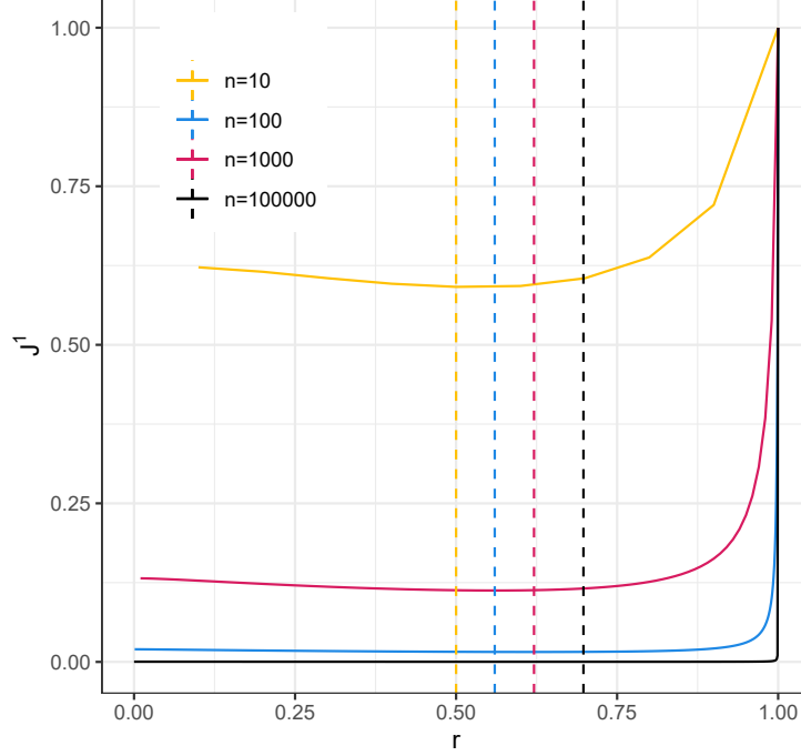
Figure 2.9: Values of J^1 on trees of different sizes calculated using equation (2.34) for different values of r = k/n . The dashed lines are at values of r which minimise J^1 .
