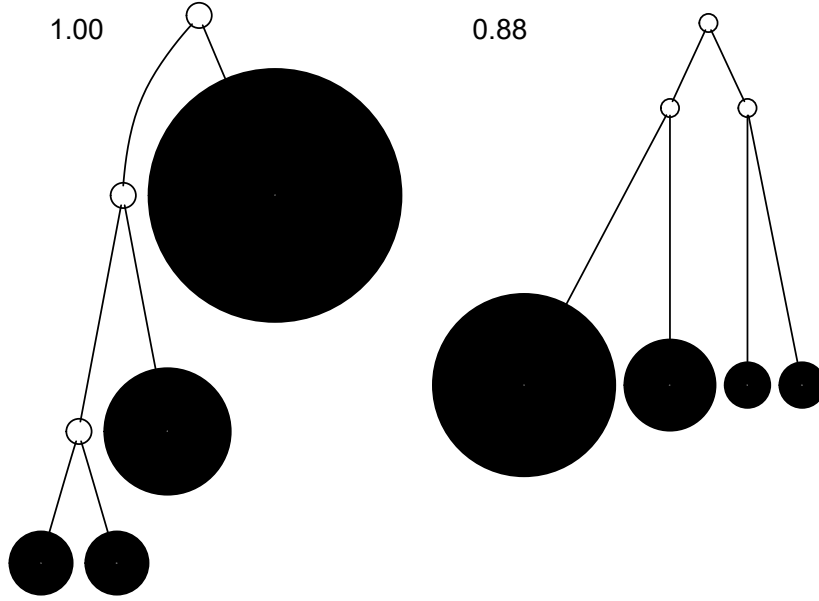
Figure 2.6: By including the node-balance function W^1 in J^1 , we allow for the possibility of perfectly balanced caterpillars (left) and less balanced fully symmetric trees (right) based on the node size distribution in the tree. The leaf sizes in these two trees are identical, with a ratio 4 : 2 : 1 : 1 from largest to smallest.
