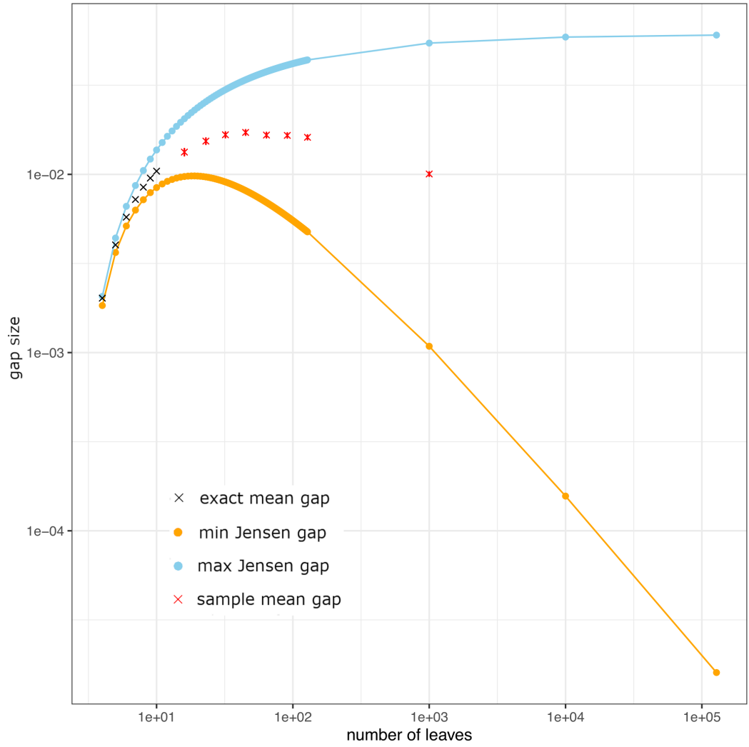
Figure 2.4: Extended figure 2.3C — uniform process. The convergence of the upper bound to \frac{4}{3}\pi is much slower than the convergence of the lower bound to 0, and the maximum it reaches over the plotted range is 0.0604 for n = 128000 . The red crosses, as in figure 2.3, suggest convergence of the gap size.
