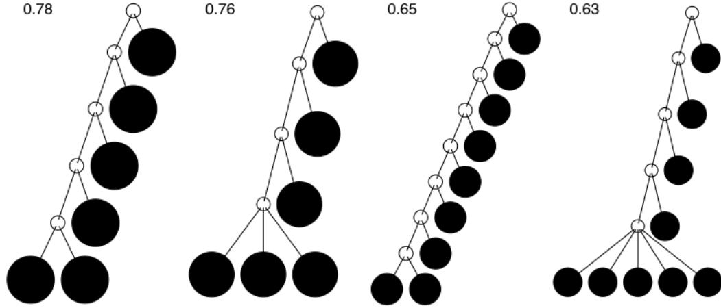
Figure 2.7: If we limit our search to leafy trees with equal leaf sizes, the least balanced tree on a given number of leaves is not necessarily the caterpillar. Pictured are the caterpillar trees on 6 and 9 leaves, as well as minimally balanced brooms for 6 and 9 leaves, with corresponding J^1 values.
