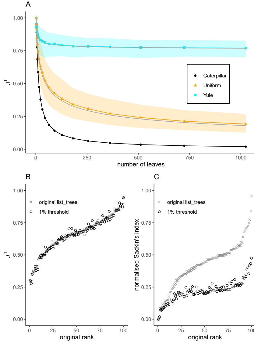
Figure 1.2: A Sample mean J^1 values for trees generated under the Yule process and the uniform model. Solid grey curves represent the approximate expected values, and the shaded areas the 5th and 95th percentiles. Each point was averaged over 100 random trees generated under the Yule or uniform models, and caterpillar tree J^1 values were calculated exactly.
