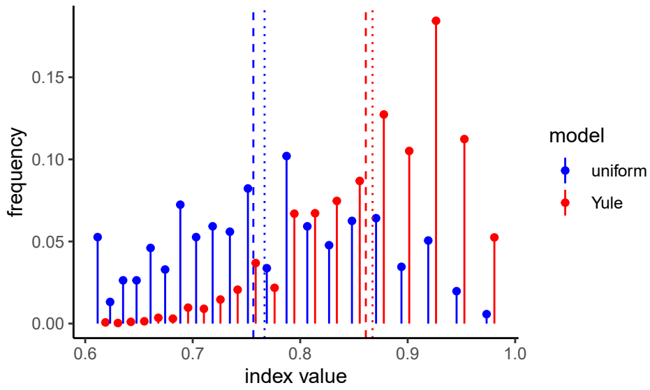
Figure 2.5: Higher variance in the uniform model leads to a non-zero upper bound on the Jensen gap. Shown are frequencies of J^1 values on 10-leaf trees generated under the Yule and uniform models. The dashed lines represent the true expected value of J^1 , and the dotted lines the approximate value calculated as \frac{n \log_2 n}{\mathbb{E}(I_S)} .
