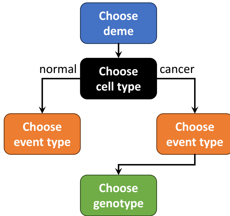
Figure 1.3: Event hierarchy in the demon-warlock framework. The algorithm works on a top-down basis, choosing first a deme, then a cell within the deme, and finally an event to perform on the cell. Figure reproduced from (Bak et al. 2023) with the authors' permission.
