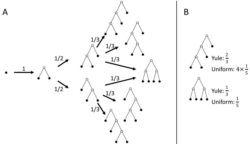
Figure 2.2: Comparison of probabilities for generation of trees on 4 leaves under the Yule and uniform models. A: Arrows show generation under the Yule model. Each of the trees shown on 4 leaves has the same probability under the uniform model. B: Comparison of probabilities of tree topologies on 4 leaves under the Yule and uniform models.
