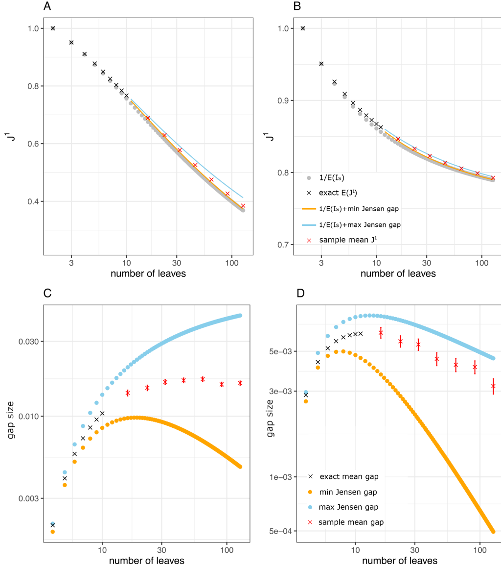
Figure 2.3: Top row: True values of \mathbb{E}(J^1) for up to 10 leaves were calculated manually, and the approximations up to 128 leaves were calculated as n \log_2 n / \mathbb{E}(I_S) . A — uniform model, B — Yule model.
