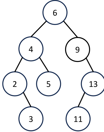
Figure 2.1: A simple example of a binary search tree over the set of labels S = \{2, 3, 4, 5, 6, 9, 11, 13\} .
