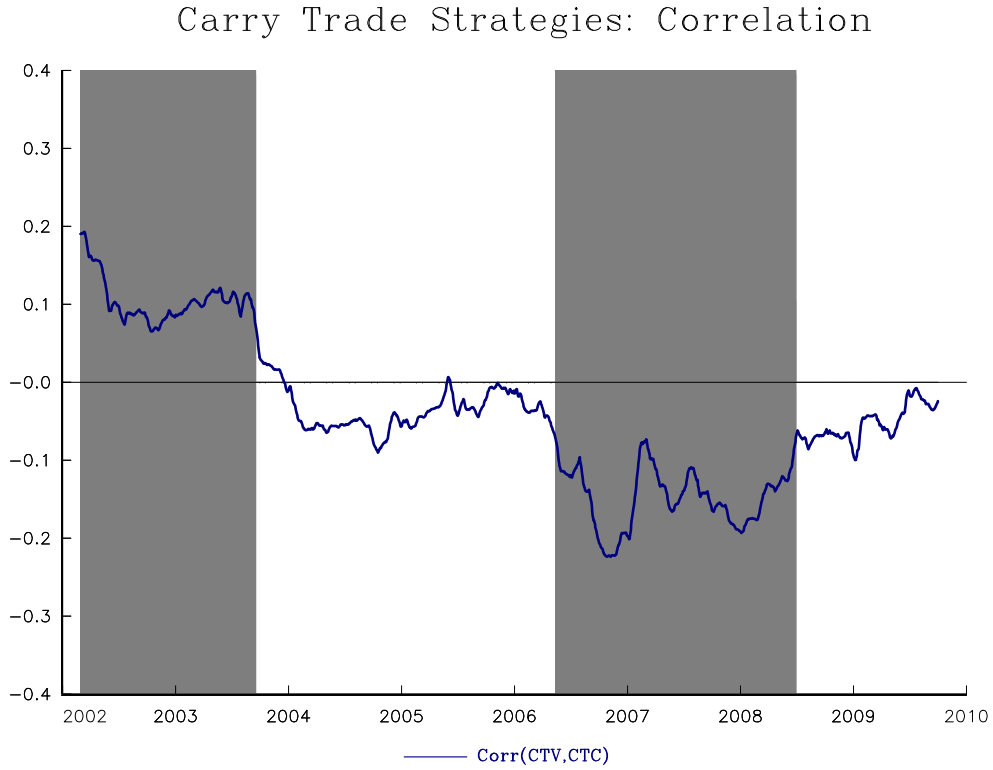
Figure 2. Out-of-Sample Correlation of Carry Trade Strategies
