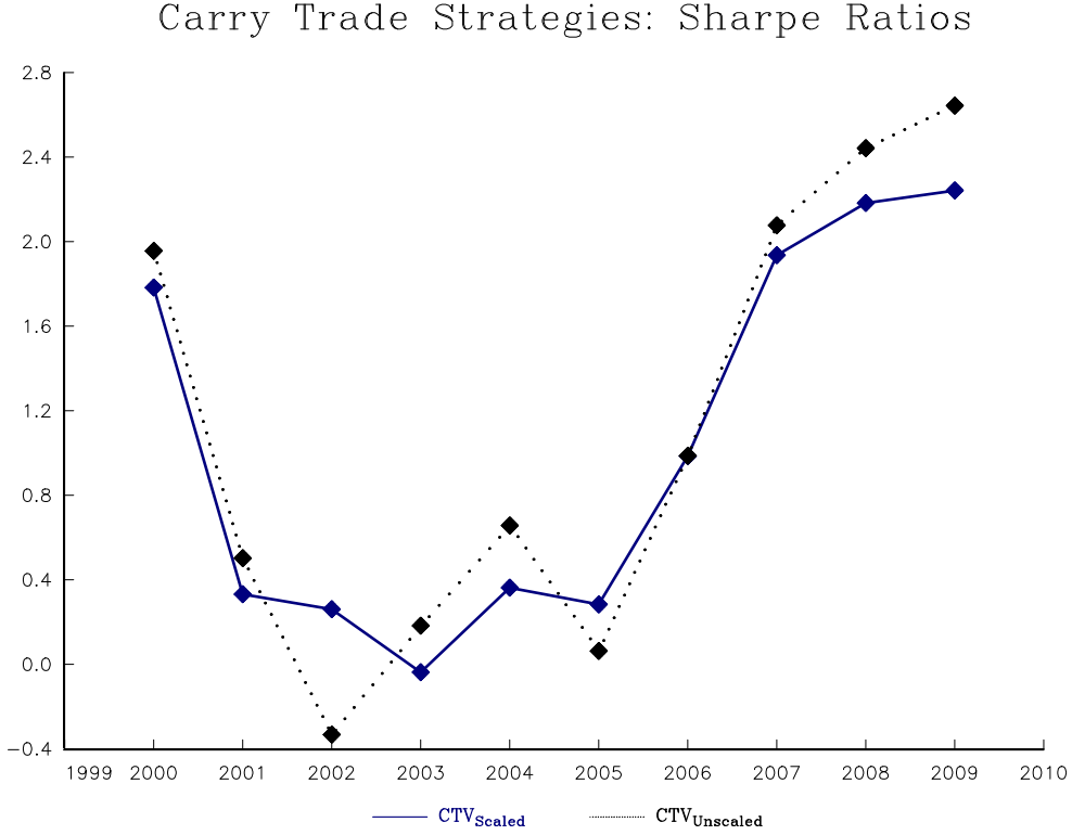
Figure 4. Out-of-Sample Sharpe Ratio of Carry Trade Strategies
