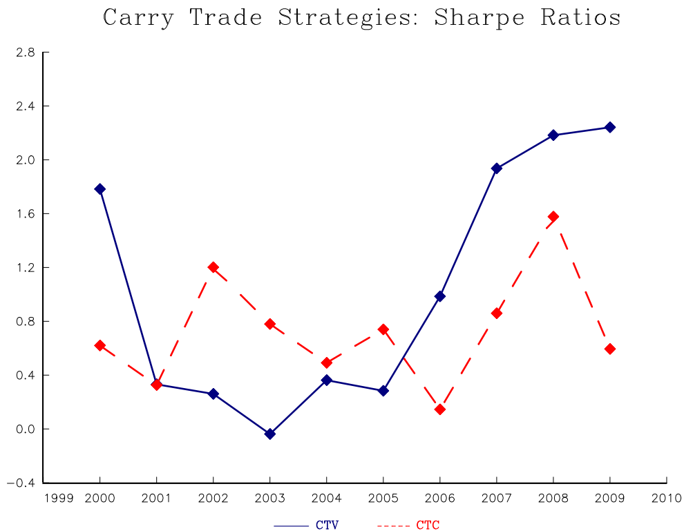
Figure 3. Out-of-Sample Sharpe Ratio of Carry Trade Strategies
