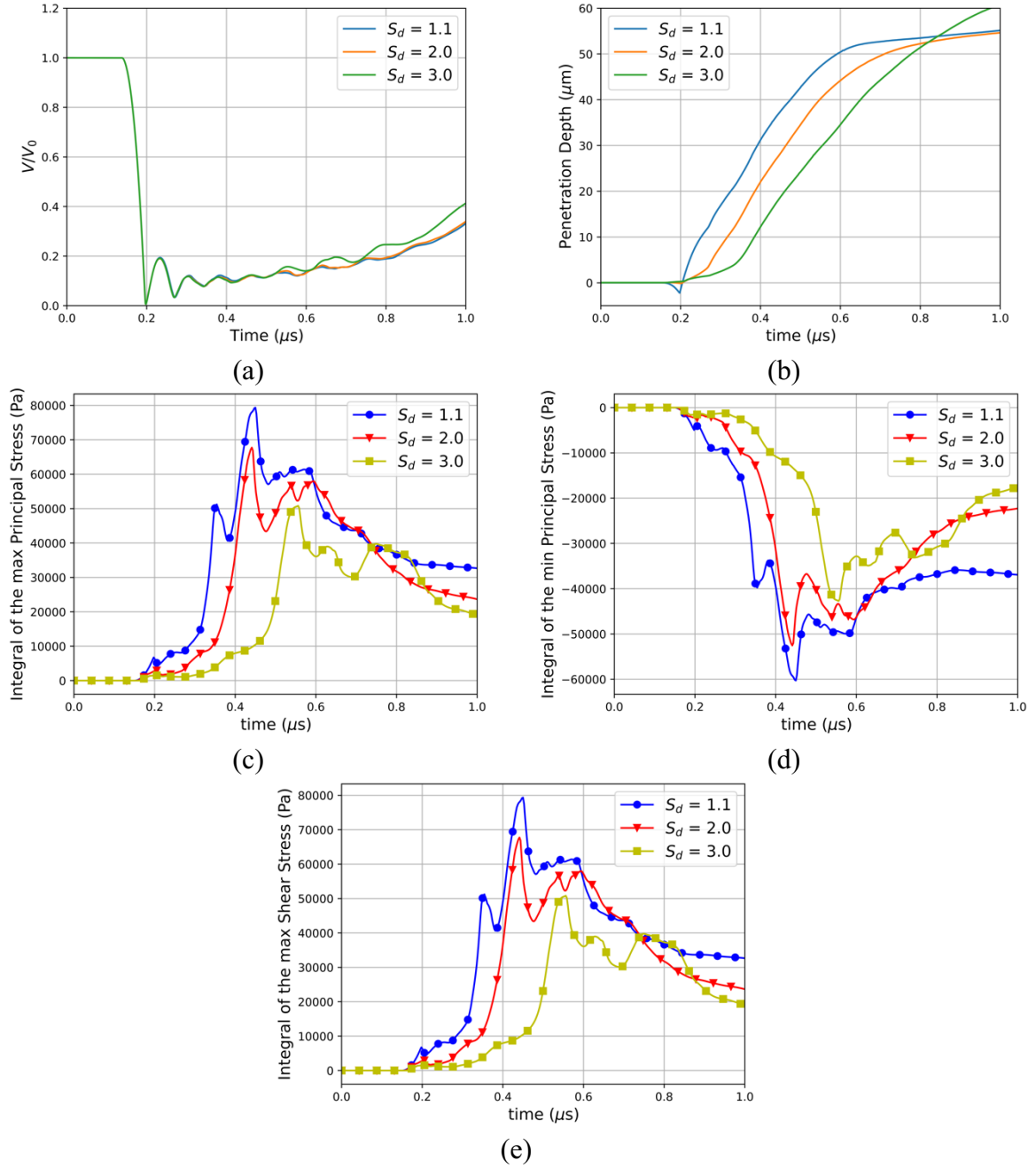
Figure 3-10. Effect of the standoff distance (a) Temporal evolution of the normalized air volume (b) Temporal evolution of the penetration depth of the liquid jet for 3 different standoff distances (c) Integral of the maximum principal stress for 3 different standoff distances (d) Integral of the minimum principal stress for 3 different standoff distances (e) Integral of the maximum shear stress for 3 different standoff distances.
