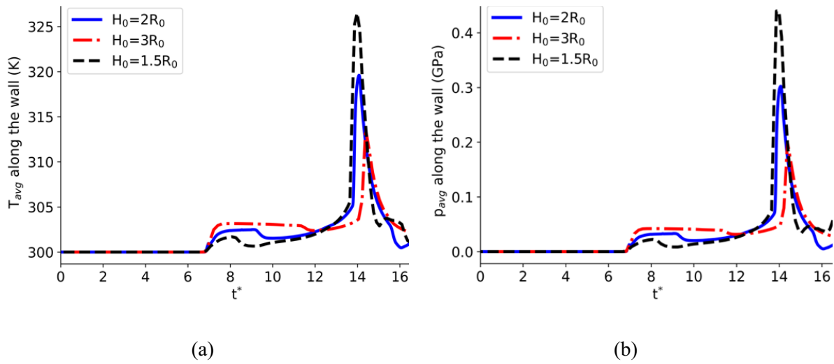
Figure 4-10. Space-averaged (in r < R_0 ) liquid temperature (a) and pressure (b) along the wall over time.
