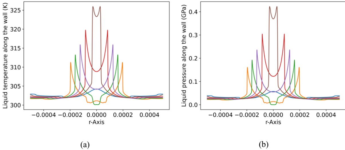
Figure 4-8. Liquid temperature (a) and pressure (b) along the wall at different times after the shock hits the wall.
