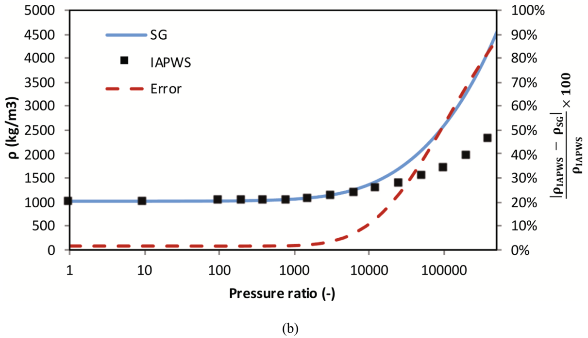
Figure 2-3. Comparison of temperature (a) and density (b) obtained with the SG EoS commonly used in bubble dynamic studies and the IAPWS data at different compression ratios. Squares represent the IAPWS reference, the blue line results of the SG EoS and the red line is the error in percentage corresponding to the right axis.
