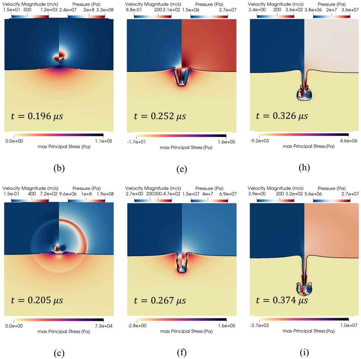
Figure 3-4. Ultrasound-induced collapse of an air bubble of R_0 = 10 \mu m with an initial stand-off d/R_0 = 1.1 near gallbladder at different timesteps. The black isosurface separates the three materials and is defined by \alpha_k = 0.5 . Upper left hand: contour of velocity magnitude. Upper right hand: contour of pressure. Bottom half: contour of the maximum principal stress.
