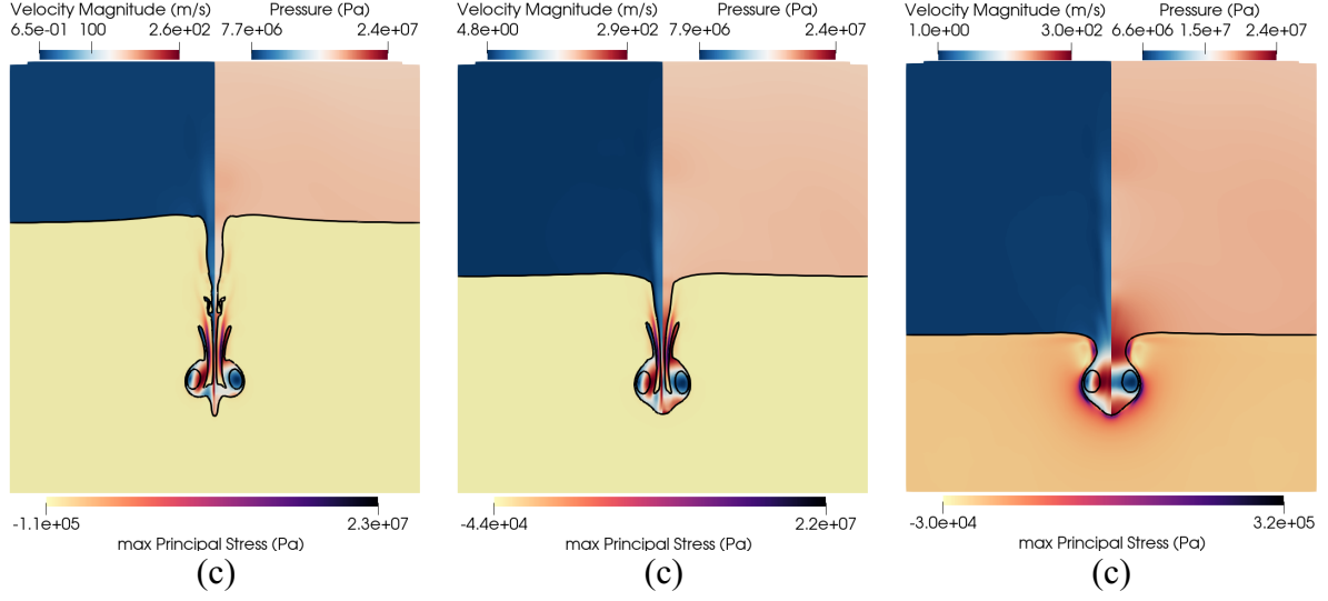
Figure 3-11. Effect of the standoff distance. Ultrasound-induced collapse of an air bubble of R_0 = 10 \mu m near bileduct at t = 0.19 \mu s , t = 0.31 \mu s , and t = 0.44 \mu s for standoff distances S_d = 1.1R_0 , S_d = 2.0R_0 and S_d = 3.0R_0 . The black isosurface separates the three materials and is defined by \alpha_k = 0.5 . Upper left hand: contour of velocity magnitude. Upper right hand: contour of pressure. Bottom half: contour of the maximum principal stress.
