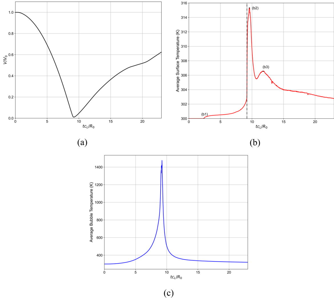
Figure 5-4. The ultrasound-induced collapse of an air bubble of R_0 = 50 \mu m with an initial stand-off D/R_0 = 1.1 near a soft material. The dash-dotted line represents the collapse time. (a) Temporal
