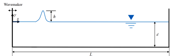
Fig. 11. Schematic wave tank for solitary wave.
