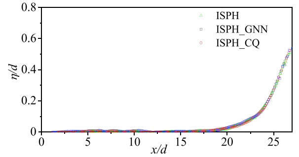
Fig. 22. Comparisons of wave profiles between different ISPH results in the case of solitary wave propagation on a slope ( h = 0.24d ).
