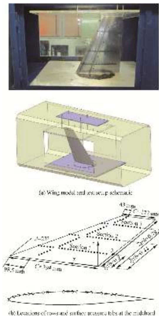
Fig. 2 Wing model and test setup schematic, and locations of rows and surface pressure tabs at the midchord.
