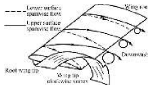
Fig. 1 Wing tip vortex.
