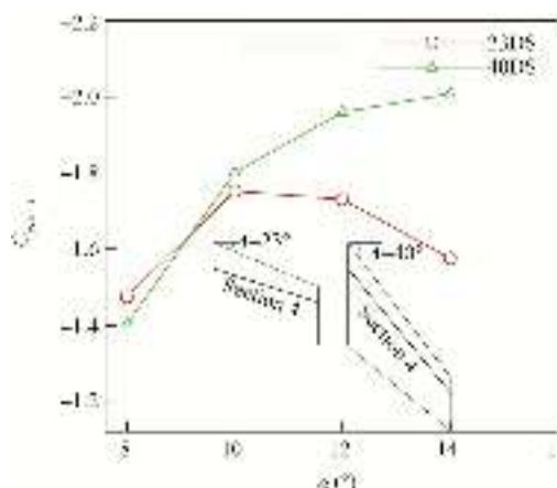
Fig. 10 Variation of spanwise C_{p,min} .
