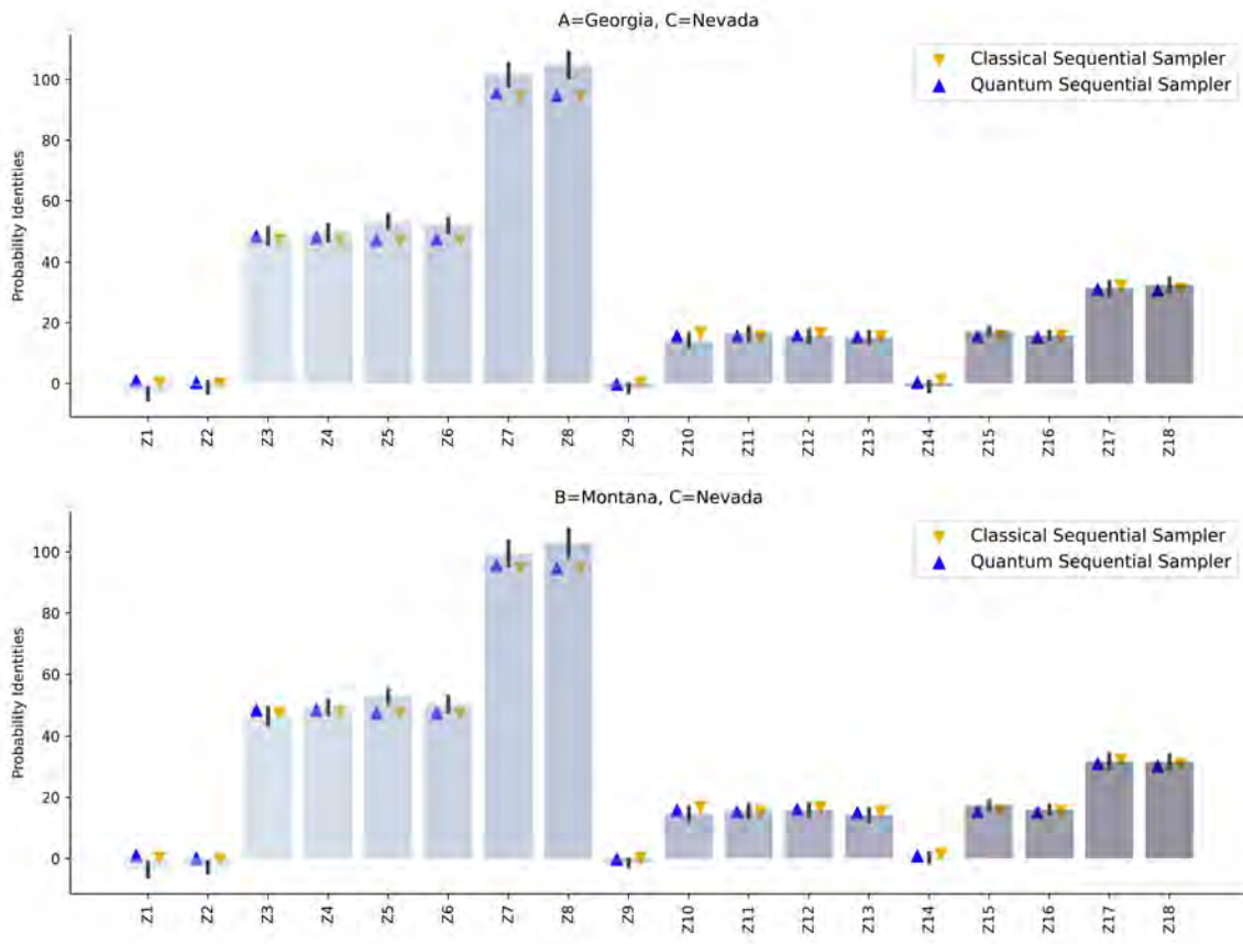
Figure S.4.3. The empirical value of probabilistic identities in Table 2, together with values computed from best-fit predictions, from the quantum and classical variants of the Quantum Sequential Sampler.
