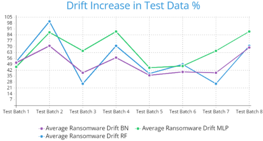
Figure 4.18: Drift Increase in Test Data
