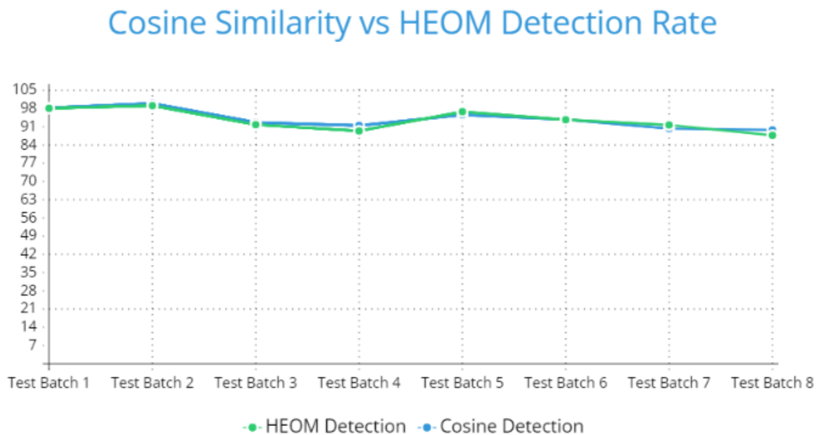
Figure 4.22: Cosine vs HEOM Detectionk
