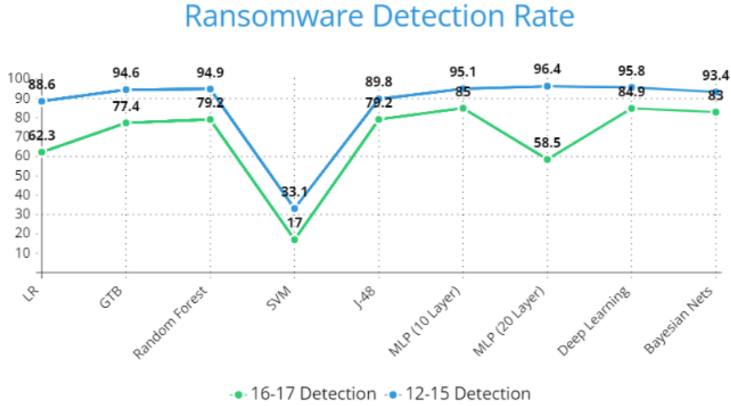
Figure 4.2: API-Call Dataset Ransomware Detection Rates
