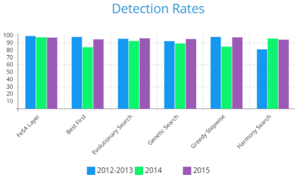
Figure 4.5: EldeRan Dataset Ransomware Detection Rates
