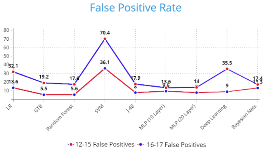
Figure 4.3: API-Call Dataset False Positive Rates
