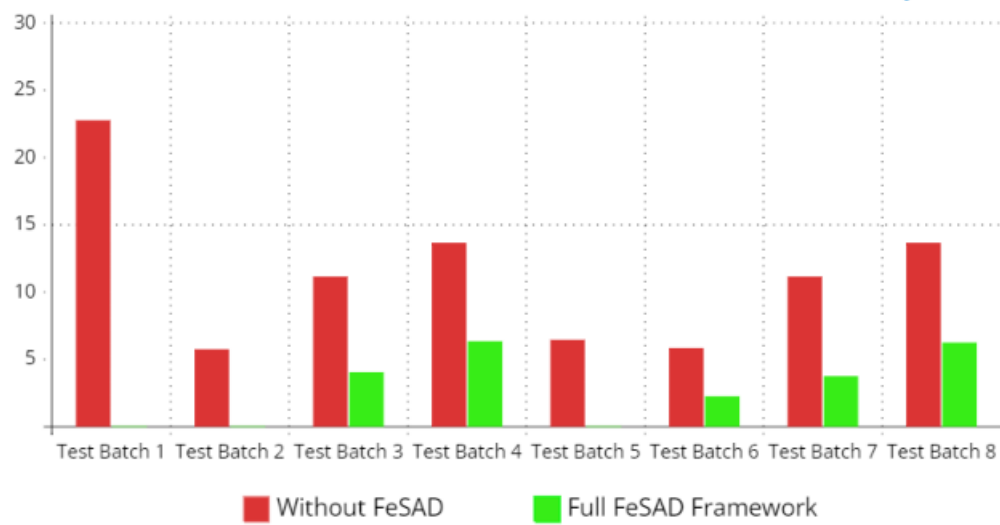
Figure 4.14: Concept Drift Data Random Forest Detection Reduction
