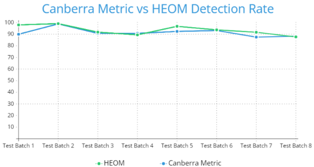
Figure 4.24: Canberra Metric vs HEOM Detection
