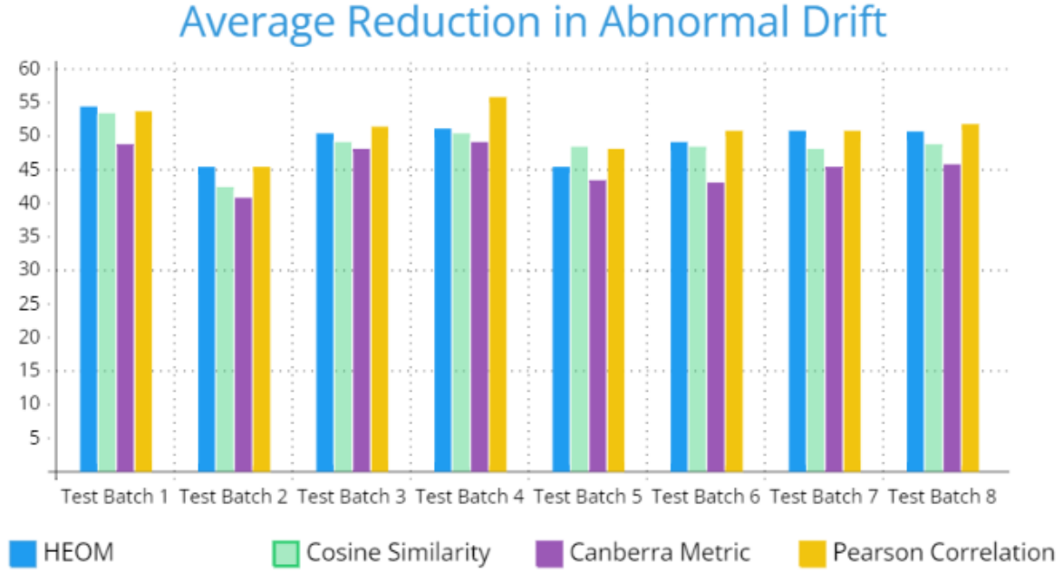
Figure 4.34: Average Abnormal Reduction
