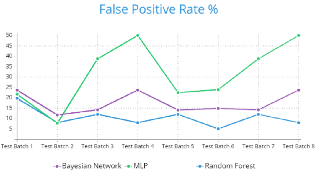
Figure 4.9: False Positive Rate without FeSAD
