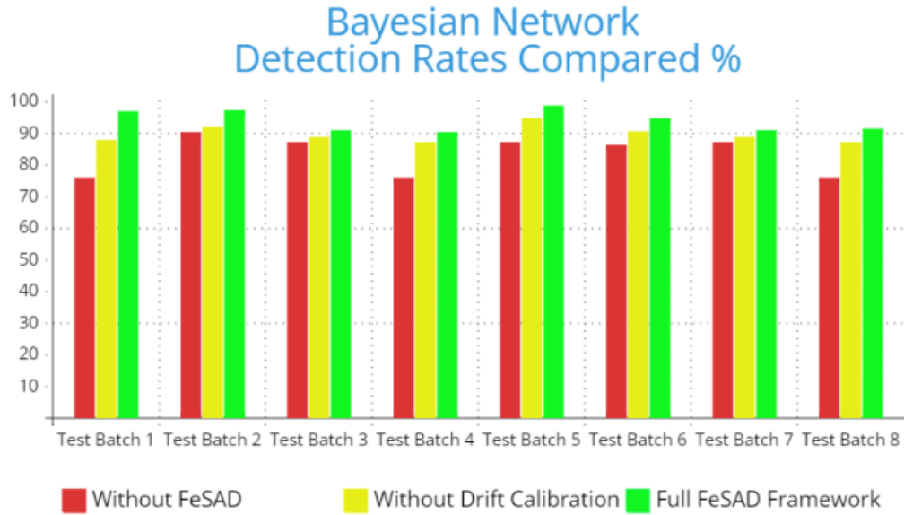
Figure 4.13: Bayesian Network Detection Rates Compared
