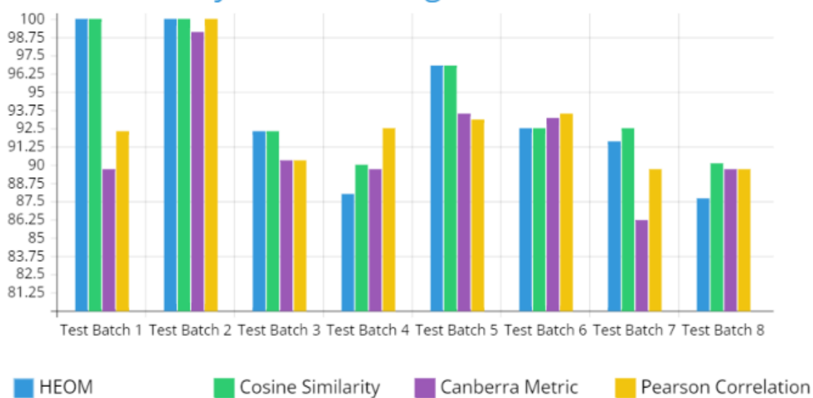
Figure 4.29: MLP Performance per Similarity Measure
