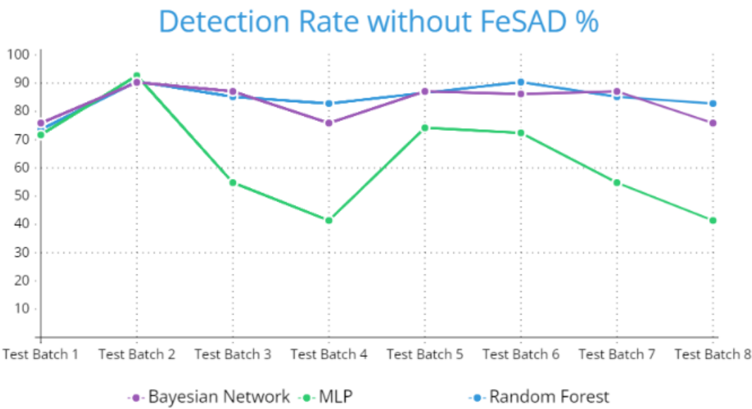
Figure 4.10: Detection Rate Without FeSAD
