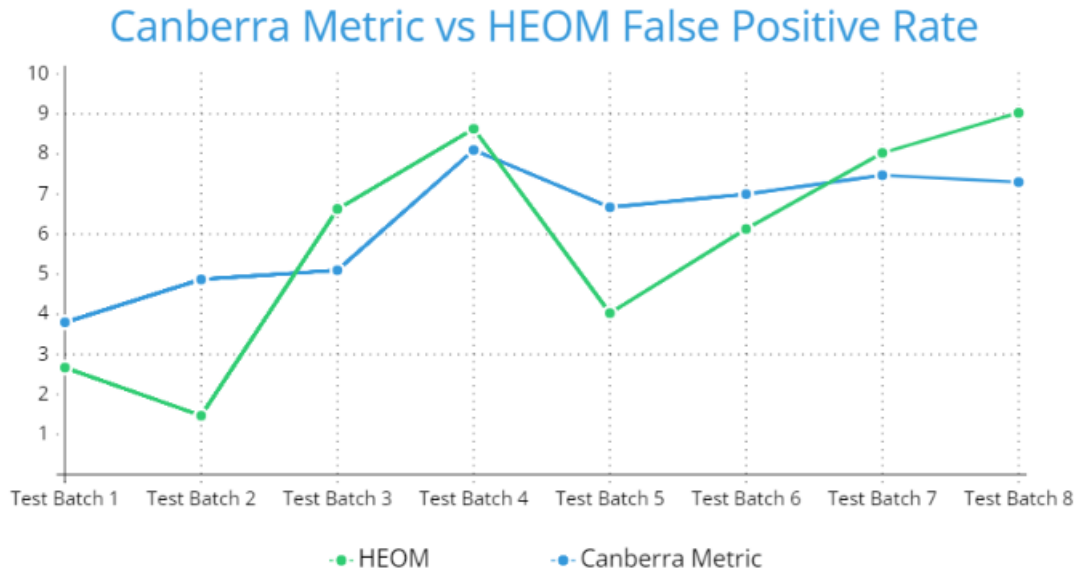
Figure 4.25: Canberra Metric vs HEOM False Positive Rate
