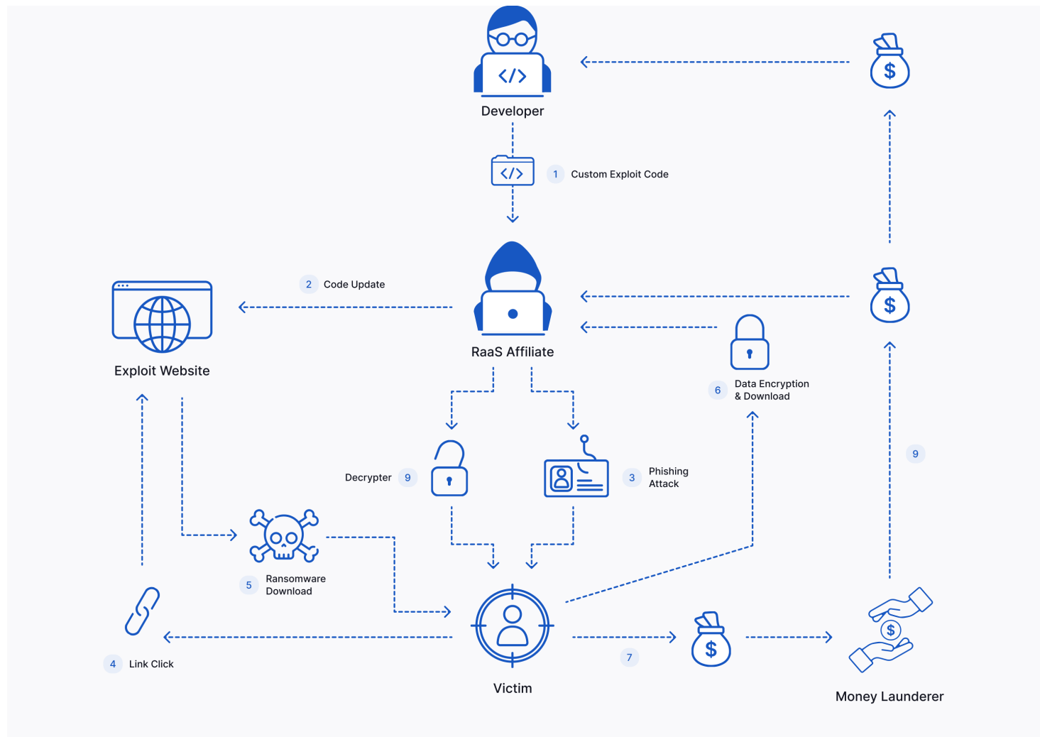
Figure 2.2: Ransomware Threat Model
