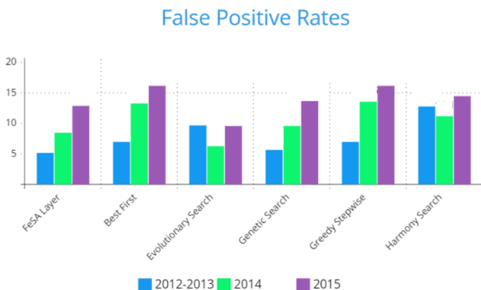
Figure 4.6: EldeRan Dataset False-Positive Rates
