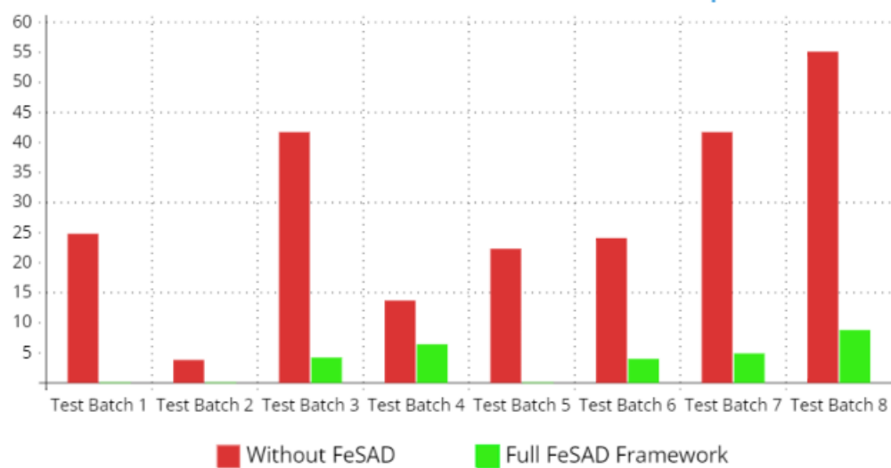
Figure 4.15: Concept Drift Data MLP Detection Rate Reduction
