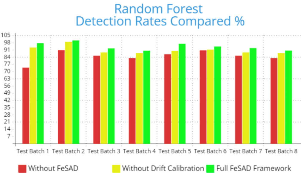
Figure 4.11: Random Forest Detection Rates Compared
