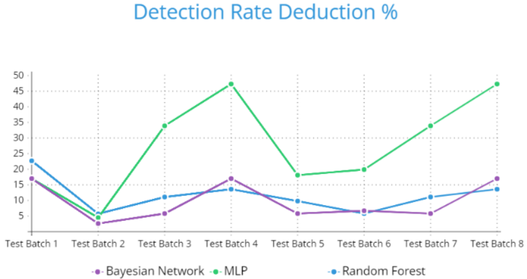
Figure 4.8: Detection Rate Deduction
