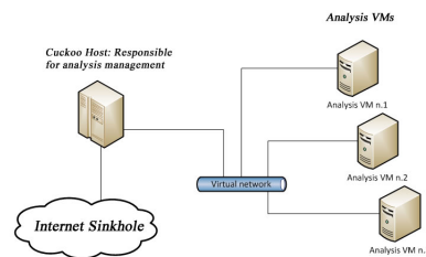
Figure 4.1: Cuckoo Sandbox Setup
