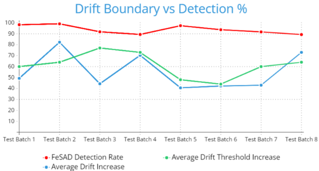
Figure 4.20: Drift Boundary vs Detection
