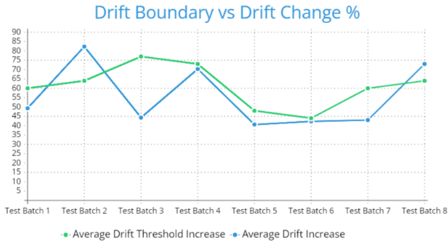
Figure 4.19: Drift Boundary vs Drift Change
