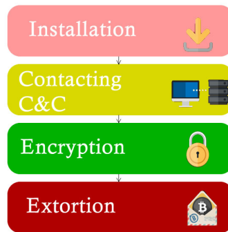
Figure 2.1: Ransomware Methodology
