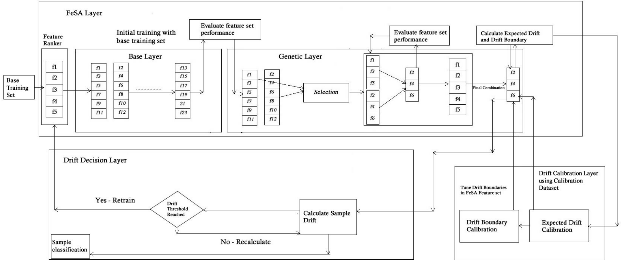
Figure 3.1: FeSAD Framework
