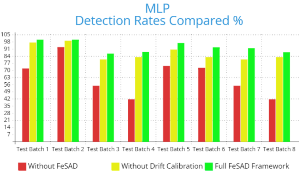
Figure 4.12: MLP Detection Rates Compared
