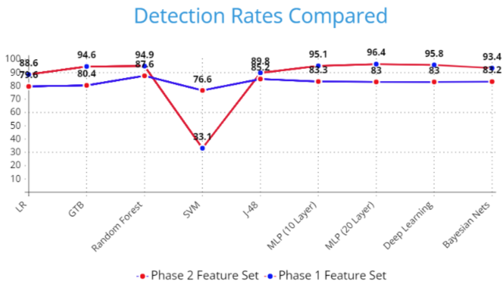
Figure 4.4: API-Call Dataset Detection Rates Compared
