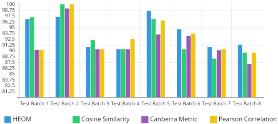
Figure 4.30: Bayesian Network Performance per Similarity Measure
