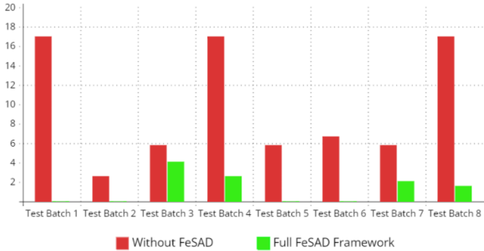
Figure 4.16: Concept Drift Data Bayesian Network Detection Reduction
