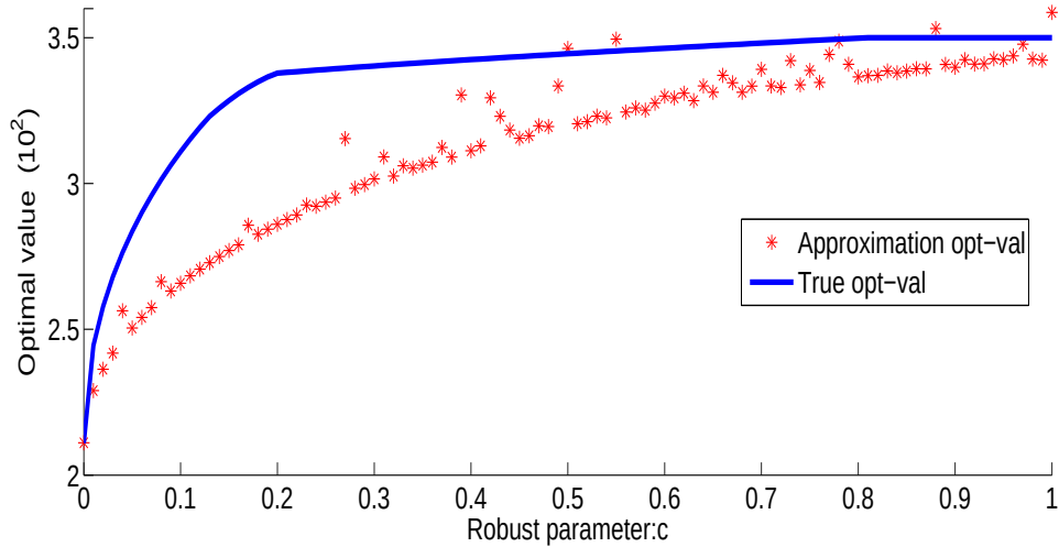
FIG. 6.1. Optimal value of problem (6.2)
