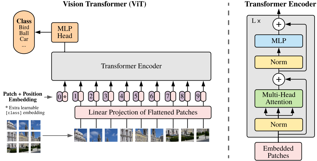
FIGURE 2.3: Vision Transformer. Images are split into fixed-size patches and linearly embedded as sequences. Then position embeddings are added and the resulting vectors are fed to a standard Transformer encoder. Source: Dosovitskiy et al. (2021) .
