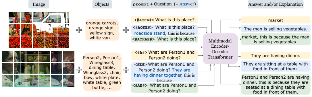
FIGURE 6.1: Illustration of UMAE: we train a multimodal encoder-decoder model on the mix of VQA tasks for jointly optimising answer and explanation, where we distinguish the training instances and target output with artificial prompt tokens (e.g., <#AOKA#>). The top and bottom examples are from A-OKVQA and VCR, respectively.
