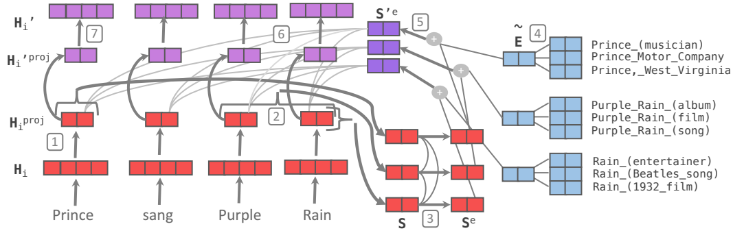
FIGURE 2.6: Illustration the Knowledge Attention and Recontextualisation (KAR) component in KnowBert. BERT word piece representations ( H_i ) are first projected to H_i^{\text{proj}} (1), then pooled over candidate mentions spans (2) to compute S , and contextualised into S^e using mention-span self-attention (3). An integrated entity linker computes weighted average entity embeddings \tilde{E} (4), which are used to enhance the span representations with knowledge from the KB (5), computing S^e . Finally, the BERT word piece representations are recontextualised with word-to-entity-span attention (6) and projected back to the BERT dimension (7) resulting in H_i' . Source: Peters et al. (2019) .
