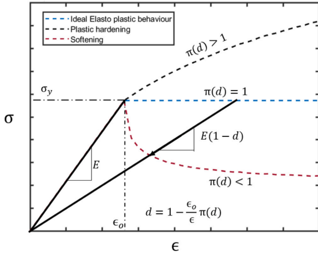
Fig. 6. (a) Strain vs. stress behavior of one-dimensional damage hyperelasticity model for ideal elasto plastic behavior, plastic hardening and softening (Einaiv et al., 2007).
