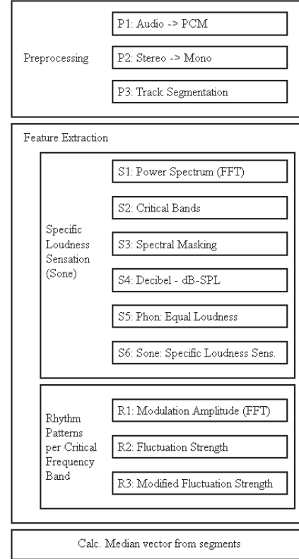
Figure 1: Block diagram of Rhythm Pattern extraction.
