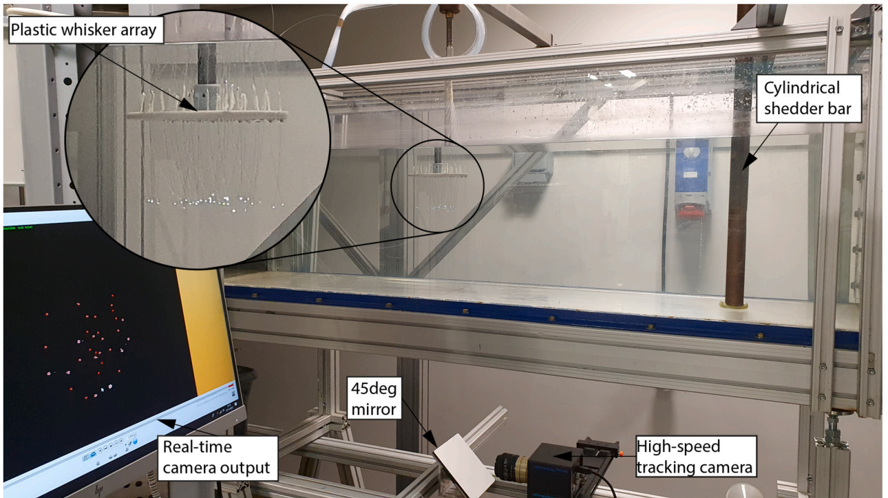
Fig. 1. Pictured is the experimental setup for flow disturbances in established flow, using a spiral array of visually tracked plastic fibre whiskers.
