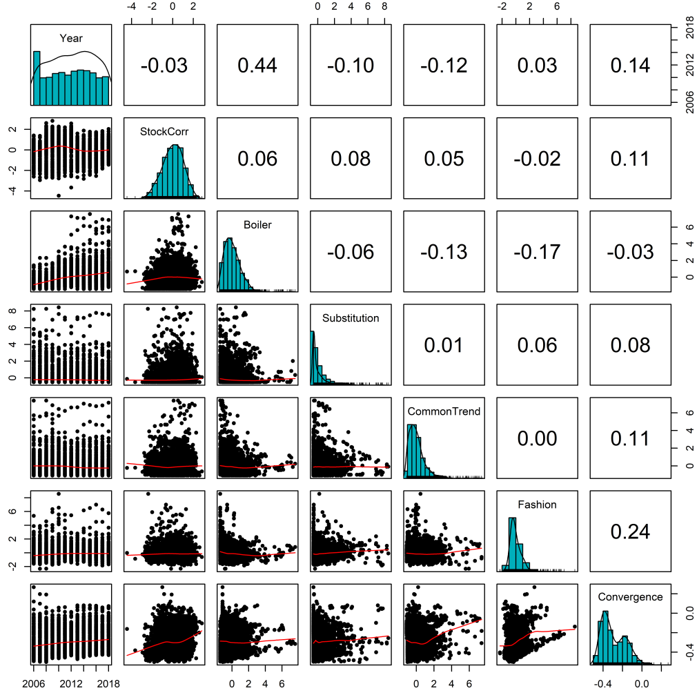
Figure 3: Scatter plot matrix of Convergence , control variables and antecedents.
