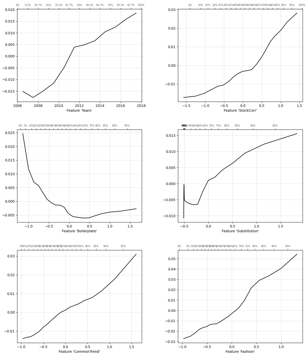
Figure 4: ALE plots for the Random Forest regression model.
