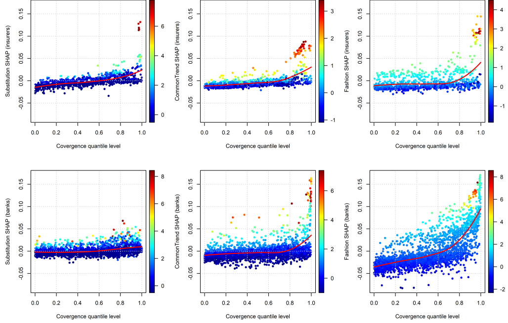
Figure 6: Sensitivity analysis based on Shapley values: feature contributions to predicted value, against quantile level of predictions; color represents the feature value. Top: insurers; bottom: banks.
