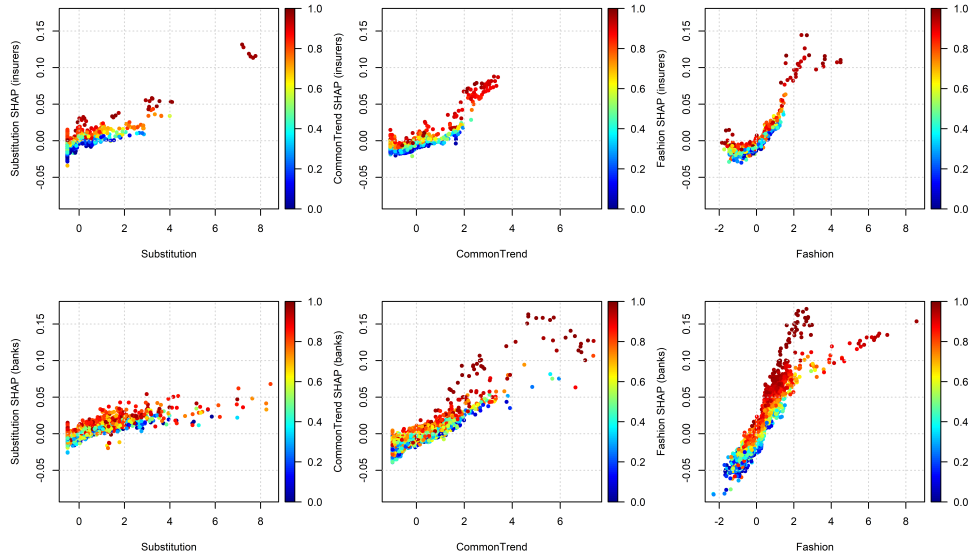
Figure 7: Sensitivity analysis based on Shapley values: feature contributions to predicted value, against feature values; the colors represent the quantile level of predictions. Top: insurers; bottom: banks.
