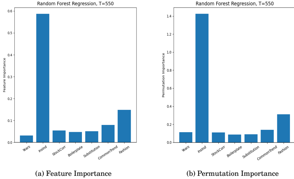
Figure 5: Variable importance of each antecedent: (a) impurity-based feature importance; (b) permutation importance.
