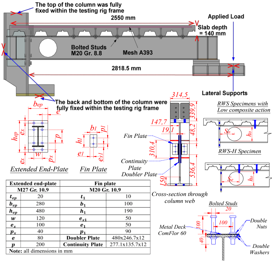
Fig. 1: Dimensions of test specimens (mm) [6].
