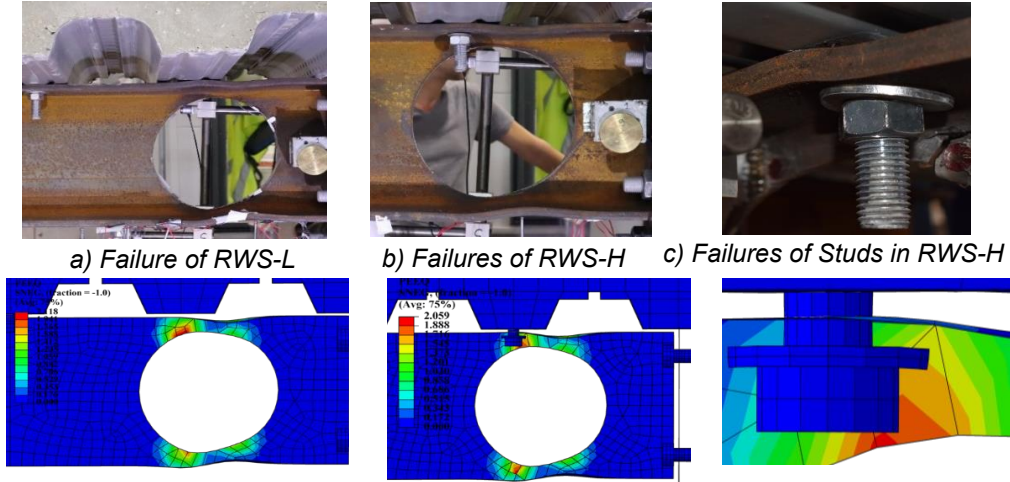
Fig. 3: Comparison between tests and FE models.
