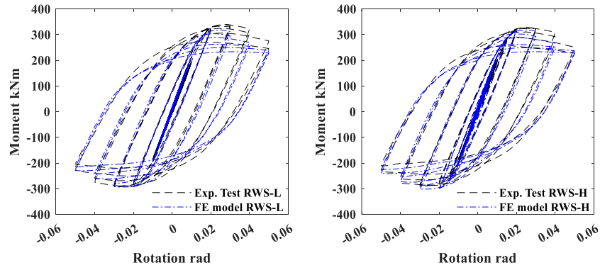
Fig. 2: Comparing between FE and experimental results.
