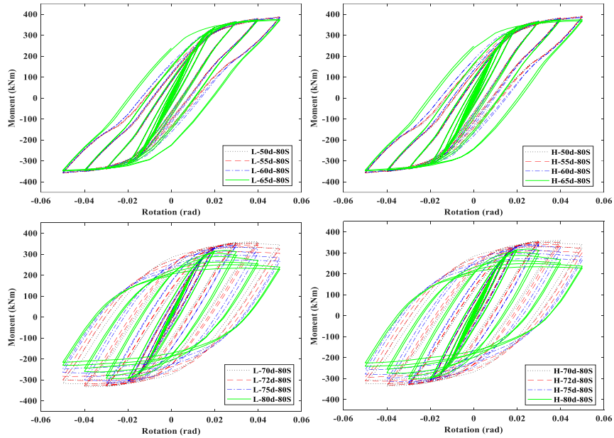
Fig. 5: Moment-Rotation curves for all FE models.
