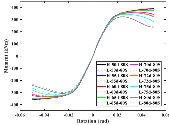
Fig. 6: Skeleton curves for all FE models.
