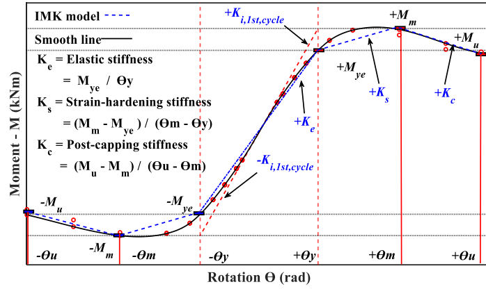
Fig. 4: Backbone curve for hysteretic models using IMK
