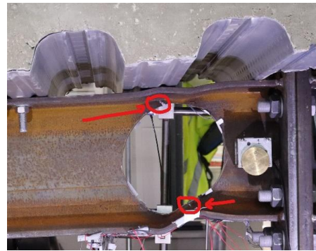
Second and third cracks in RWS-L connection.
