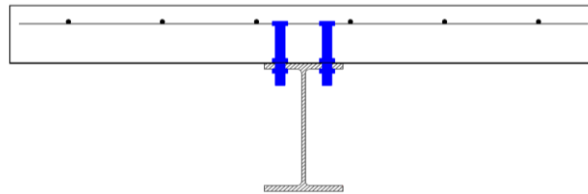
Figure 1. Demountable bolted
