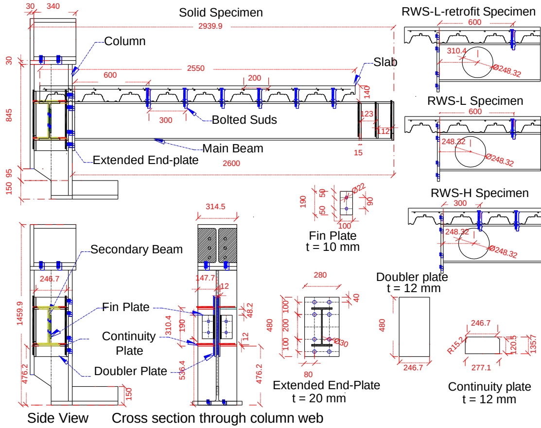
Figure 2. Dimensions of test specimens (mm)
