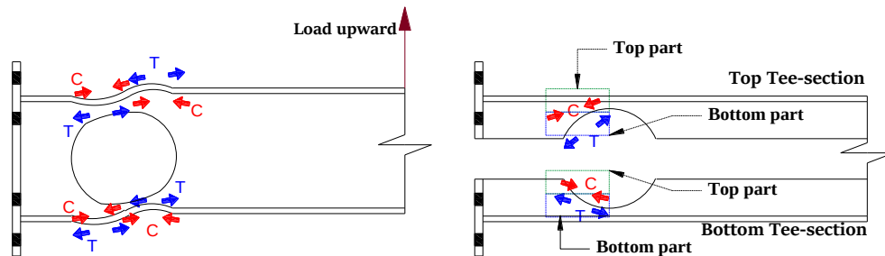
Figure 5. Illustration of the behaviour of Tee-sections.
