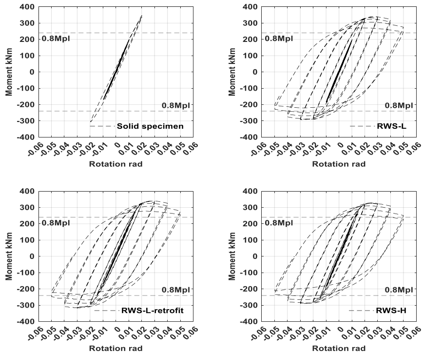
Figure 4. Hysteretic curve of the specimens.
