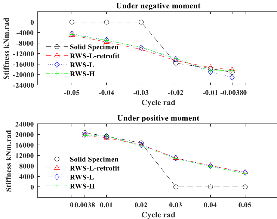
Figure 6. Degradation in the stiffness for all tested specimens
