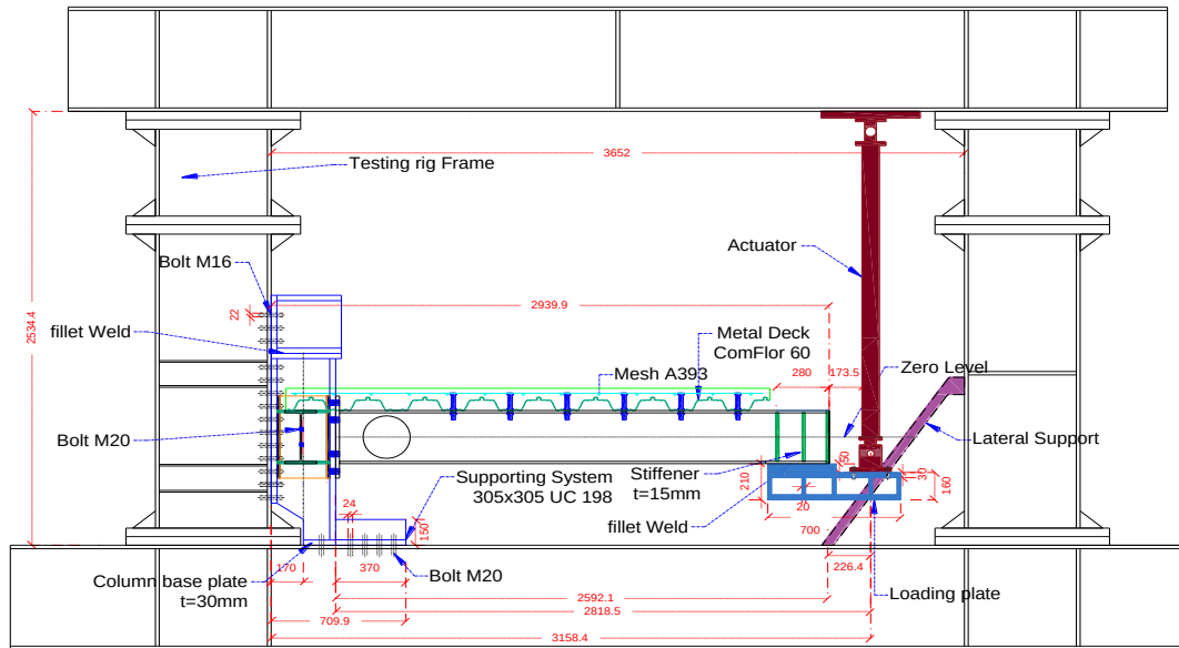
Figure 3. Experimental test setup – side view (mm)
