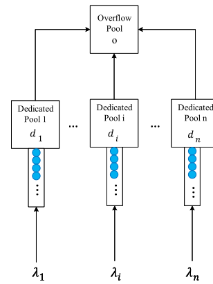
Fig. 3. The schematic diagram of an overflow system.
