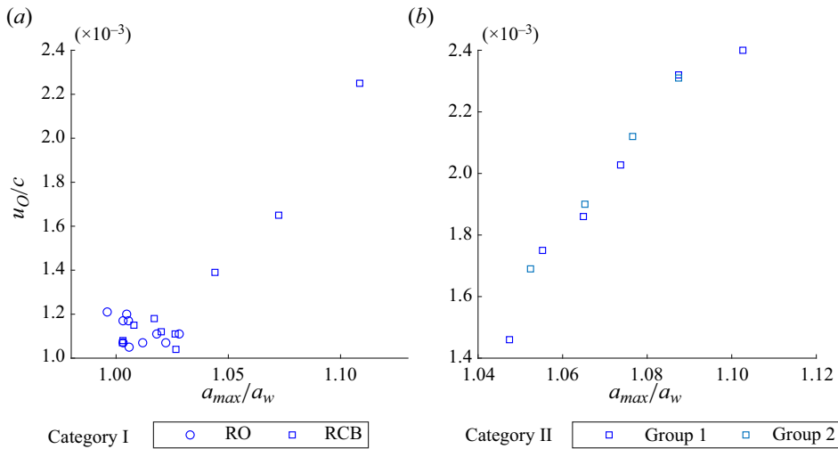
Figure 9. The celerity-normalized object drift u_O/c as a function of the local maximum wave amplitude normalized by the input wave amplitude a_{max}/a_w : (a) the results for the RCBs and ROs of different sizes (category I simulations); (b) the results for the objects of l/\lambda = 10\% with different round-corner radii and depths of submergence (category II simulations). All results shown are for the same input wave condition: a_w = 0.02 m and u_S/c = 0.0012 .
