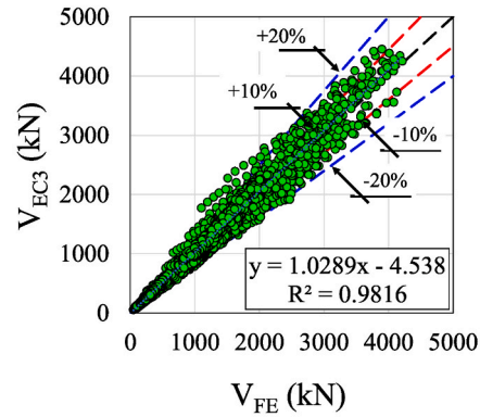
(d) Ferreira et al. [4] based on EC3
