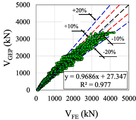
(c) GEP
