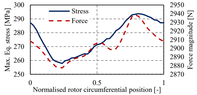
FIGURE 12: AERODYNAMIC FORCE MAGNITUDES ON THE LAST ROTOR BLADES ALONG THE CIRCUMFERENTIAL DIRECTION OBTAINED FROM THE STEADY STATE MODEL
