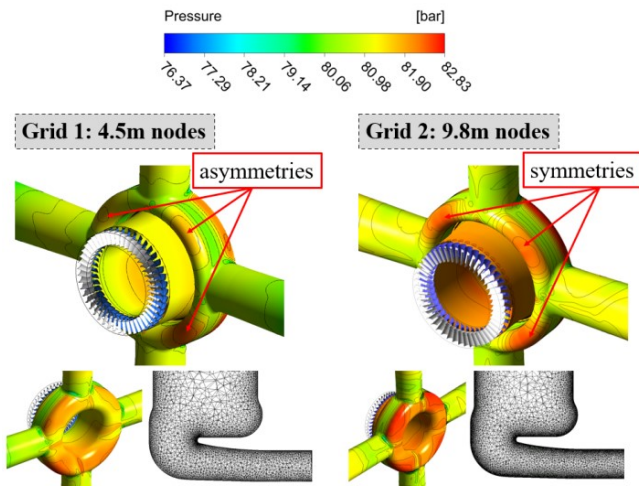
FIGURE 4: EFFECT OF GRID STRUCTURE ON THE PRESSURE DISTRIBUTION PATTERNS ON THE EXHAUST SECTION WALLS
