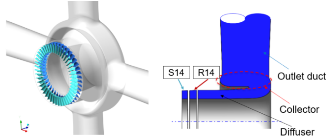
FIGURE 2: GEOMETRY DEFINITION OF MODEL 3: THE FULL ANNULUS OF THE LAST TURBINE STAGE WITH THE EXHAUST SECTION CROSS-SECTION
