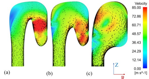
FIGURE 9: FLOW FIELD IN THE DIFFERENT CROSS SECTION MODIFICATIONS AT AN INCLINED CUT MIDWAY BETWEEN THE PERIODIC PLANE AND THE OUTLET DUCT. (A) M_1 , (B) M_2 , AND (C) M_3
