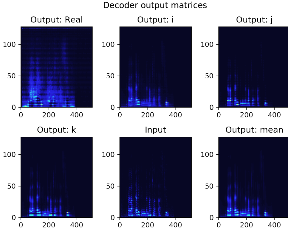
FIGURE 6.6: Example of RH-emo quaternion reconstruction of a speech spectrogram. Input is the magnitudes-only input spectrogram, Output: real , \hat{i} , \hat{j} , \hat{k} are the four output matrices of RH-emo, respectively reconstructed from the discrete emotion, valence, arousal and dominance axes of the embeddings, Output: mean is the pixel-wise average of Output: real , \hat{i} , \hat{j} , \hat{k} and is the matrix that is compared to the input in the loss function.
