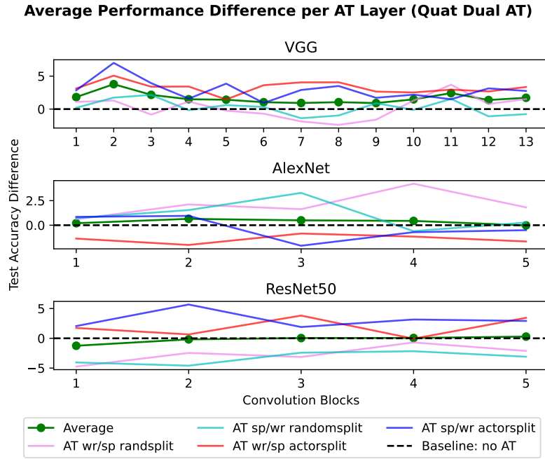
FIGURE 7.3: Average test accuracy for quaternion-valued dual AT for each AT layer in different modalities.
