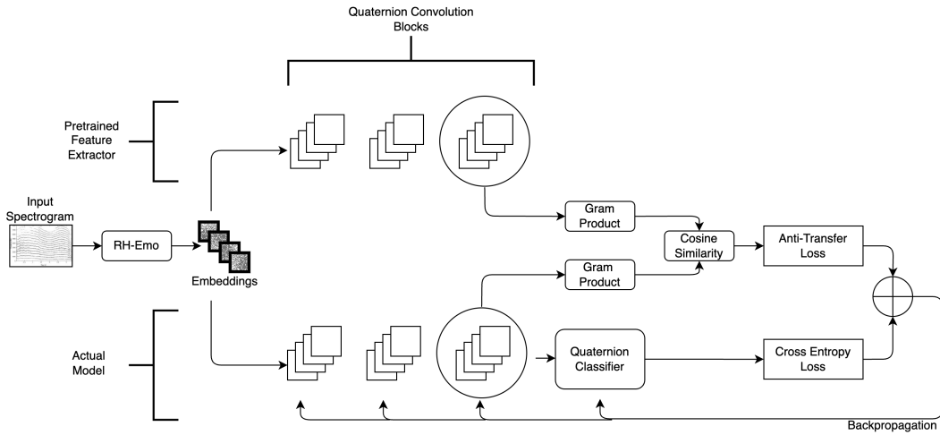
FIGURE 7.1: Block diagram of a QCNN network with anti-transfer learning applied to a SER classification task. The input spectrogram is first propagated to RH-emo, which generates quaternion emotional embeddings that feed the QCNNs. Anti-transfer is applied to the feature maps generated by selected quaternion convolution blocks.
