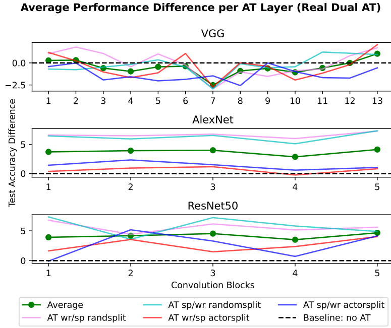
FIGURE 7.5: Average test accuracy for real-valued dual AT for each AT layer in different modalities.
