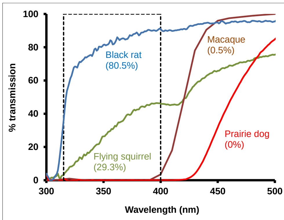
Supplementary figure S2 The proportion of UVA transmitted by the lenses of four species of mammal. This represents the area under the curve for each species within the rectangle shown expressed as a percentage of the area of the entire rectangle. Equivalent values for all species are shown in table 1.
