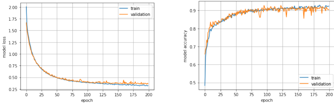
Figure 8: Training curves for the quinary classification problem for A_m , plotted against number of epochs.
