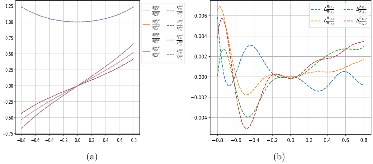
Figure 31: (a) 8-vertex model with Hamiltonian of type H_{8v,3} , with parameters a_1 = 1 , b_1 = -0.45 , d_1 = 0.6 , d_2 = 0.75 , (b) errors
