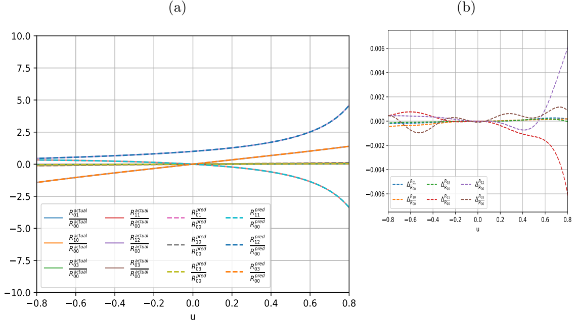
Figure 14: (a) Predicted R-matrix component ratios w.r.t. R_{00} , for conjugated XXZ model with \eta = \frac{\pi}{3} and similarity matrix \Omega = \begin{pmatrix} 0.4 & 0.5 \\ -1.2 & 1 \end{pmatrix} , (b) Absolute error between predicted and actual R-matrix ratios
