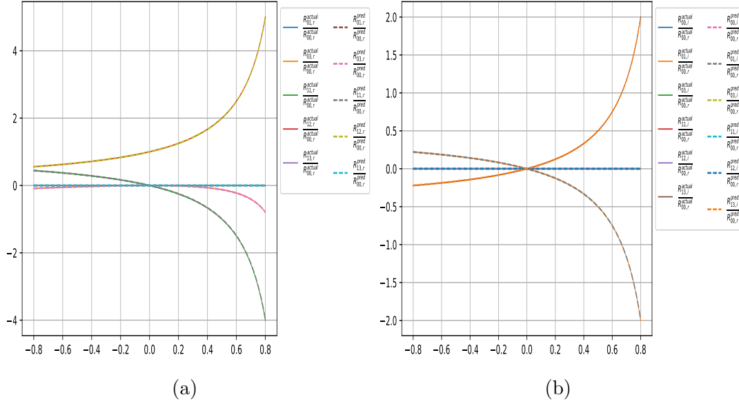
Figure 33: (a,b) class 5, with H_2 parameters a_1 = -0.5 , a_2 = -0.5i , a_3 = -0.5i : real and imaginary parts
