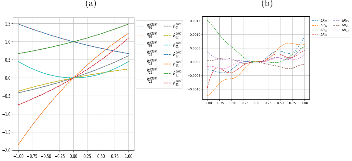
Figure 13: (a) Predicted vs actual R-matrix components for the Hamiltonian of class-1, with coefficients a_1 = .5 , a_2 = .3 , a_3 = .9 , a_4 = 1.5 , a_5 = .4 . Note here the R-matrices are automatically normalised since R_{00} was fixed to the constant value of 1, (b) Absolute error between predicted and actual R-matrix components
