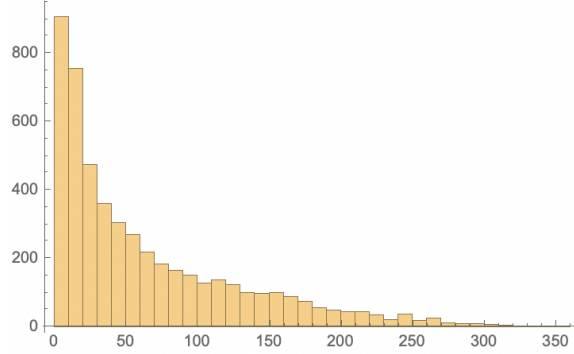
Figure 3: Distribution of the number of distinct irreps in the tensor decomposition of R_{\vec{v}_1} \otimes R_{\vec{v}_2} for A_m with randomized 1 \leq m \leq 8 and randomized ternary weight vectors \vec{v}_{1,2} . The horizontal axis denotes the length of R_{\vec{v}_1} \otimes R_{\vec{v}_2} and the vertical axis denotes the corresponding frequency.
