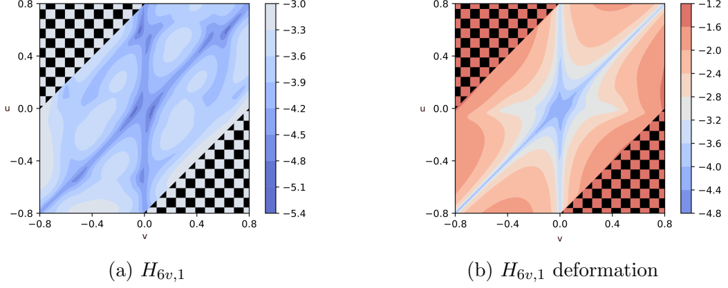
Figure 16: (a) The normalized Yang-Baxter error (6.29) plotted in the logarithmic scale at the end of training for the Hamiltonian H_{6v,1} with a_1 = 0.3, a_2 = 0.3, b_1 = 0.45, b_2 = 0.6, c_1 = 0.4, c_2 = 0.25 , and (b) its non-integrable deformation with a_1 = -1.3, a_2 = 1.3 and other parameters kept constant. In order to keep all three arguments appearing in YB equation inside the same interval |u|, |v|, |u-v| < 0.8 we cut out the area |u-v| > 0.8 with chess-pattern triangles.
