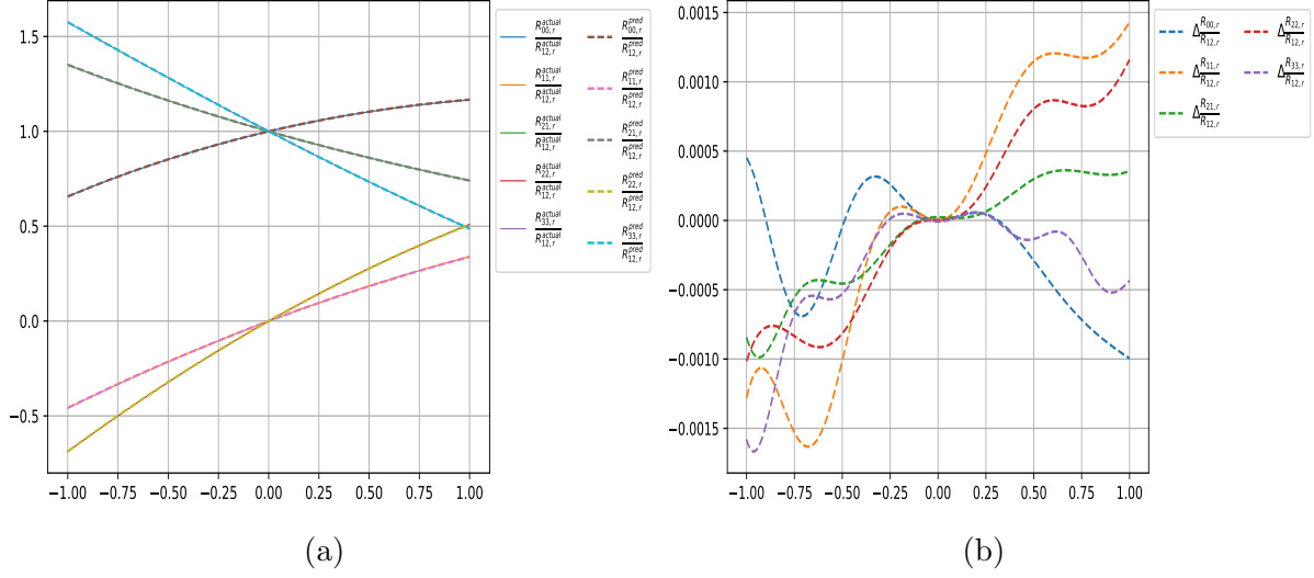
Figure 26: (a) 6-vertex model with Hamiltonian of type H_{6v,2} , with parameters a_1 = 1, a_2 = 0.2, b_1 = 0.45, b_2 = 0.75, c_1 = 0.4, c_2 = 0.6 , (b) errors
