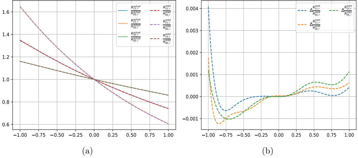
Figure 25: (a) 4-vertex model, with H_2 parameters a_1 = 0.9 , b_1 = 0.4 , b_2 = 0.6 , a_2 = 0.75 , (b) errors
