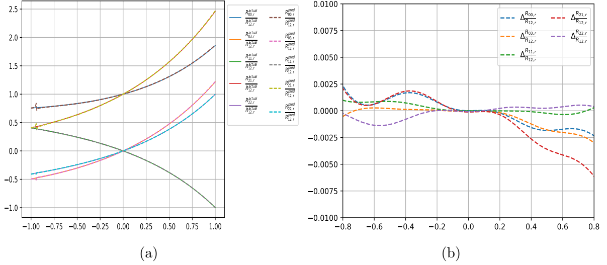
Figure 27: (a) 7-vertex model with Hamiltonian of type H_{7v,1} , with parameters a_1 = 1, b_1 = 0.45, c_1 = 0.6, d_1 = 0.75 , (b) errors
