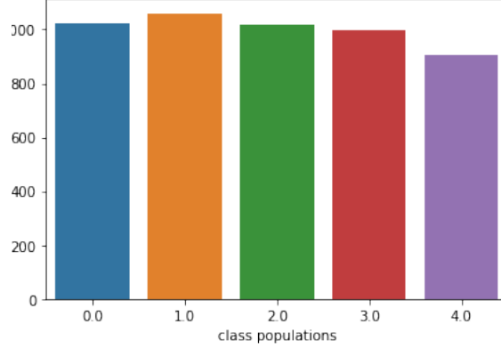
Figure 7: Class Populations of length bins for A_m irreps.
