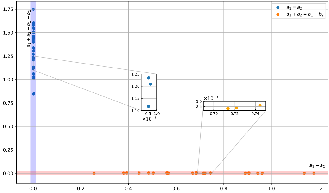
Figure 22: The 6-vertex models learnt by exploration. The graph visualizes the obtained Hamiltonians by plotting their values along the a_1 + a_2 - b_1 - b_2 and the a_1 - a_2 axes. The models H_{6v,1} lie along the y -axis and the models H_{6v,2} along the x -axis with an error margin of order 10^{-3} as shown in the telescoped inset plots.
