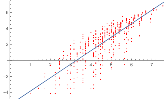
Figure 9: Plot and fit of log of the time in seconds of the branching of irreps of SU(5) versus the length of the weight-vector.
