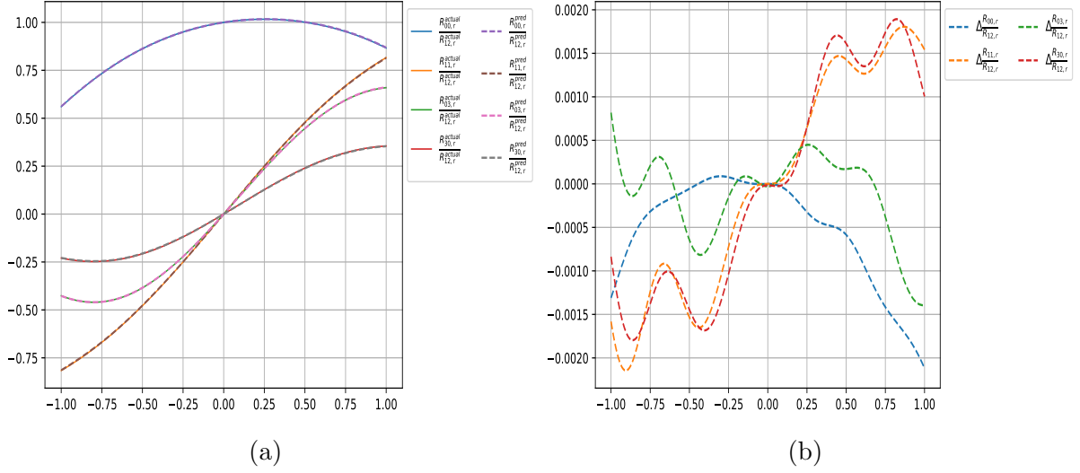
Figure 29: (a) 8-vertex model with Hamiltonian of type H_{8v,1} , with parameters b_1 = 0.4, \eta = 0.8, m = 0.5, \delta_1 = 1.3, \delta_2 = 0.7 , (b) errors
