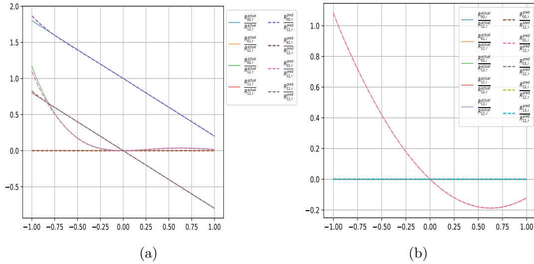
Figure 34: (a,b) class 6, with H_2 parameters a_1 = -0.4 , a_2 = -0.6i : real and imaginary parts
