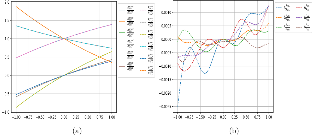
Figure 28: (a) 7-vertex model with Hamiltonian of type H_{7v,2} , with parameters a_1 = 1, c_1 = 0.45, c_2 = 0.75, d_1 = 0.5 , (b) errors
