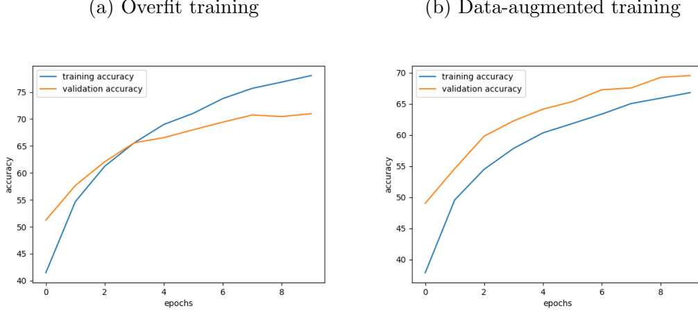
Figure 2: Overfitting during training (for 10 epochs) remedied by enlarging the CIFAR-10 dataset using data-augmentation techniques. Here, we measure the training and validation accuracies in percentage.
