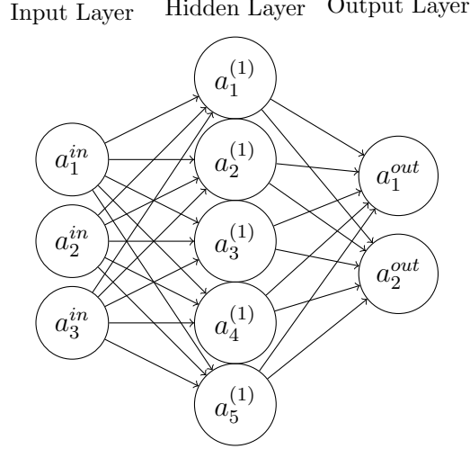
Figure 1: Multilayer Perceptron with one hidden layer L = 1 of width n_1 = 5 , input of size n_0 = 3 and output of size n_2 = 2
