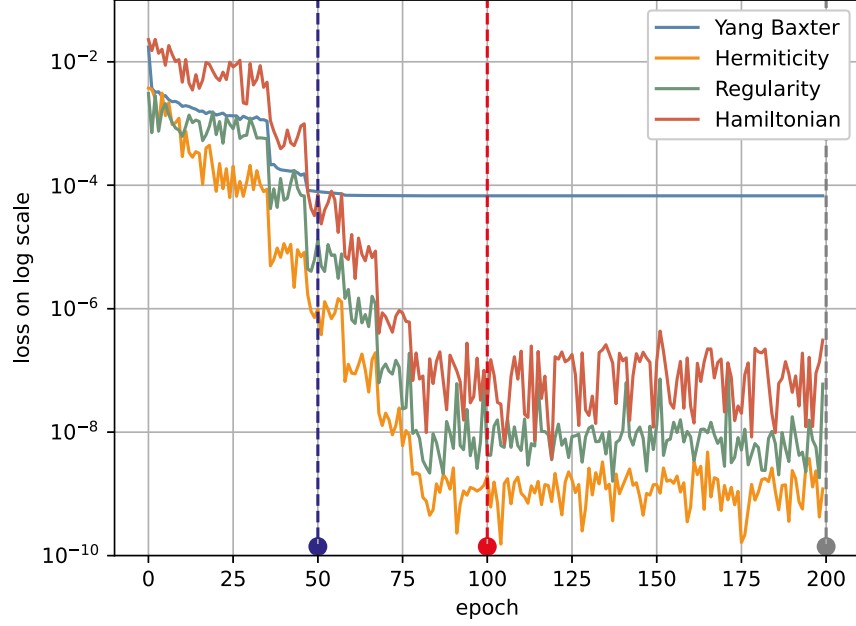
Figure 10: The evolution of training losses for the XYZ model, shown on the log scale. The losses tend to fall in a step-wise manner, which corresponds approximately to the learning rate schedule the network is trained with.
