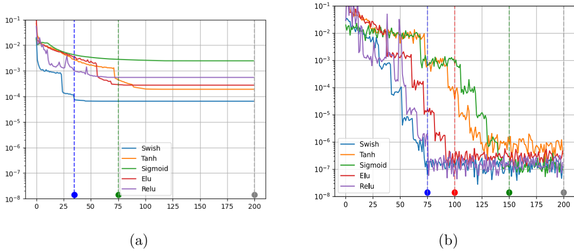
Figure 37: The evolution of the Yang-Baxter loss (left) and the Hamiltonian loss (right) for a variety of activation functions when training for 200 epochs. The swish activation tends to outperform the others. The precise numbers are given in Table 5.
