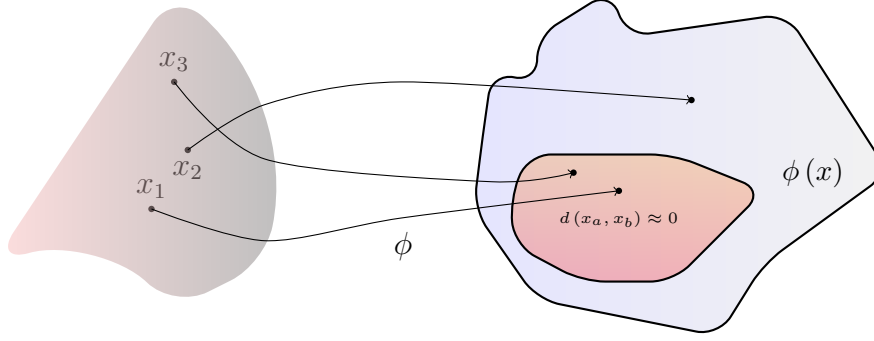
Figure 35: Visualizing the map \phi which is learnt by the Siamese architecture. The points x_1 and x_3 are similar to each other while x_2 is dissimilar to both of them.
