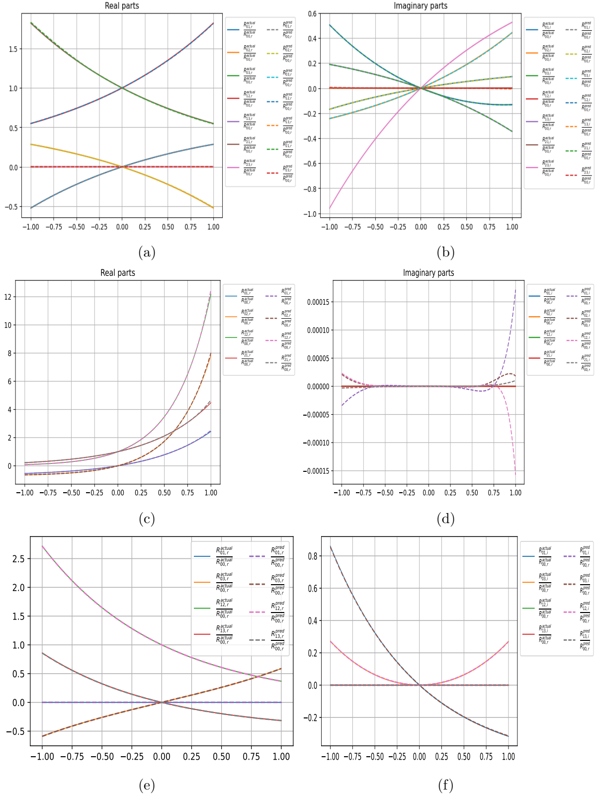
Figure 32: (a,b) class 2, with H_2 parameters a_1 = -0.6 , a_2 = 0.381 + 0.123i , a_3 = 0.447i , a_4 = 0.7i , a_5 = -0.3i : real and imaginary parts, (c,d) class 3, with H_2 parameters a_1 = 1 , a_2 = 0.5 , a_3 = 0.7 : real and imaginary parts, (e,f) class 4, with H_2 parameters a_1 = 0.5 , a_2 = -0.5i , a_3 = 0.5 , a_4 = -0.5 : real and imaginary parts
