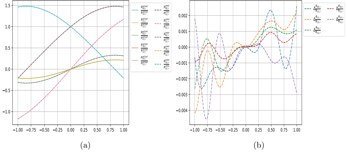
Figure 30: (a) 8-vertex model with Hamiltonian of type H_{8v,2} , with parameters b_1 = 0.4, \alpha_1 = 0.5, \beta_1 = 0.7, \delta_1 = 0.3, \delta_2 = 0.2 , (b) errors
