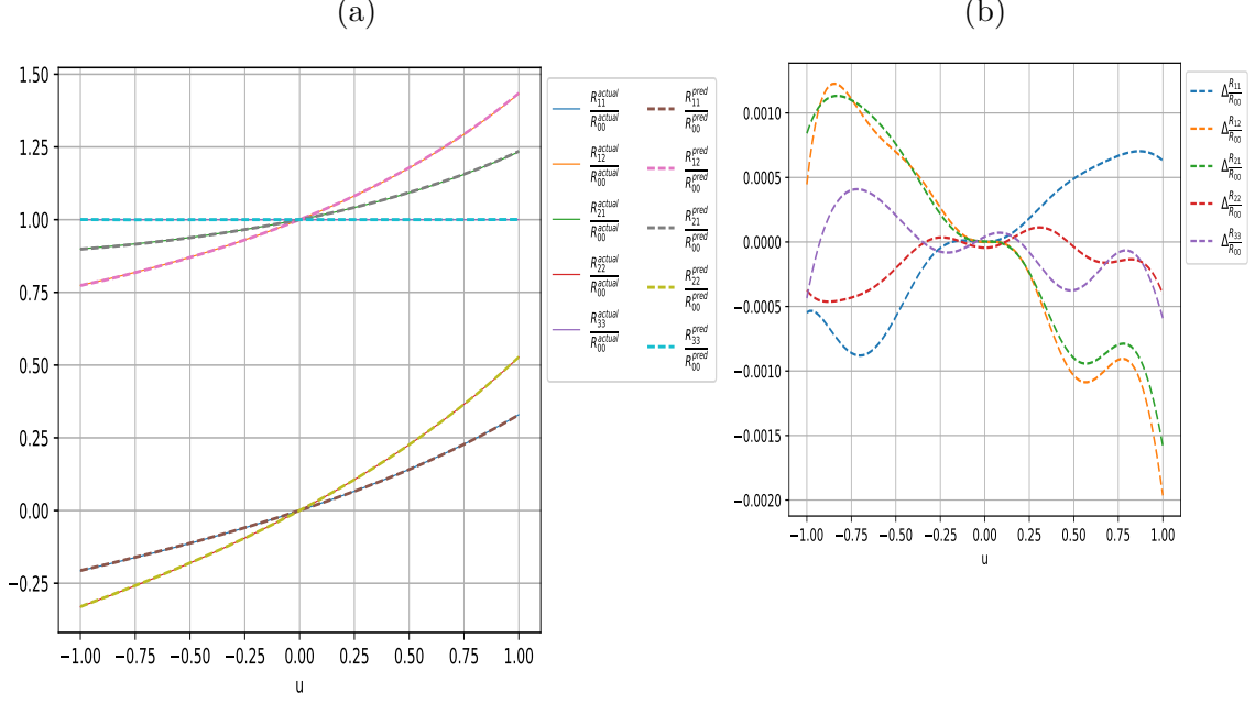
Figure 12: (a) Predicted vs actual R-matrix component ratio w.r.t. R_{00} for XXZ-type model with a_1 = a_2 = 0.3, b_1 = 0.45, b_2 = 0.6, c_1 = 0.4, c_2 = 0.25 , (b) Absolute error between predicted and actual R-matrix component ratios
