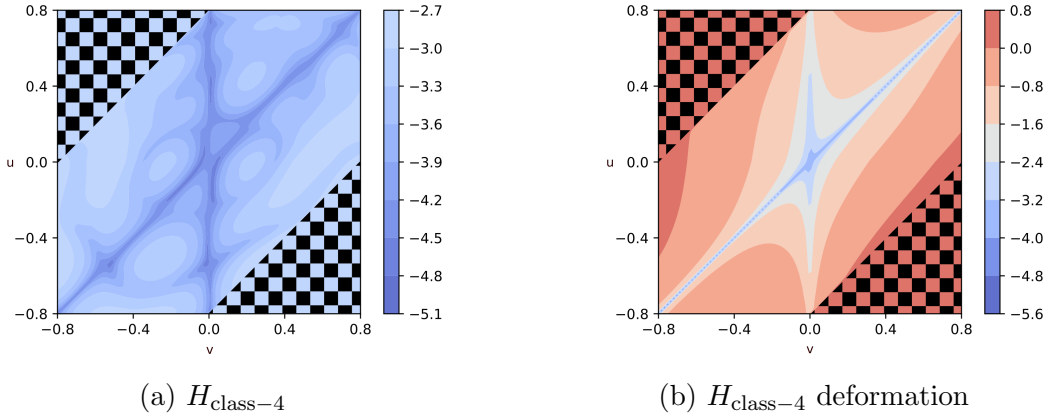
Figure 17: (a) The normalized Yang-Baxter error (6.29) plotted in the logarithmic scale at the end of training for the Hamiltonian H_{\text{class-4}} from (E.19), with a_1 = 0.5, a_2 = 0.3, a_3 = 0.4, a_4 = 0.9 , (b) Non-integrable deformation with same Hamiltonian parameters as in the integrable case, except for H_{13} = -0.9 .
