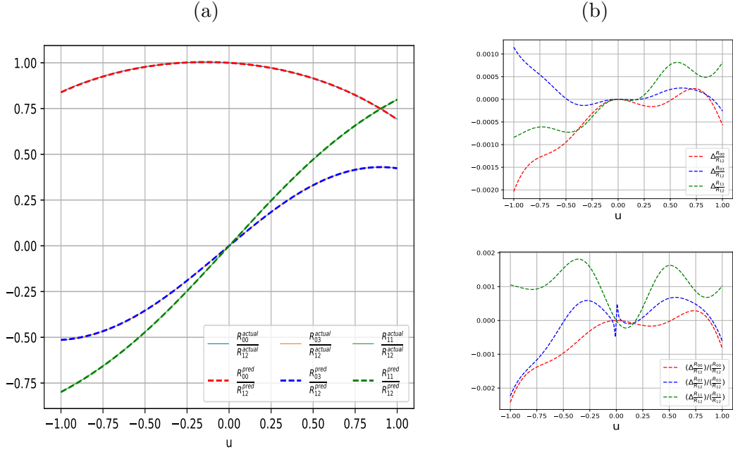
Figure 11: (a) XYZ R-matrix as ratios with respect to the (12) component for \eta = \pi/3, m = 0.6 , (b) Relative and absolute errors for R-matrix.
