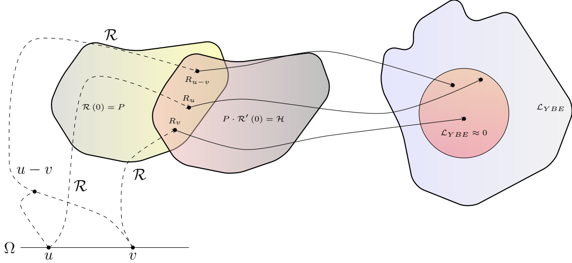
Figure 36: Visualizing the forward propagation of the neural network \mathcal{R}(u) . This has a very strong parallel to Figure 35, with the function \mathcal{R}(u) playing the role of the map \phi . The only difference is that \mathcal{R}(u) also has additional constraints on \mathcal{R}(0) and \mathcal{R}'(0) which are unique to our problem.
