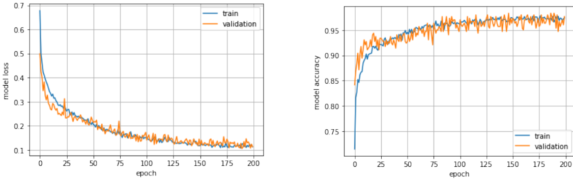
Figure 6: Loss-function (top), and model accuracy (below) for training on A_m irreps, plotted against number of epochs.
