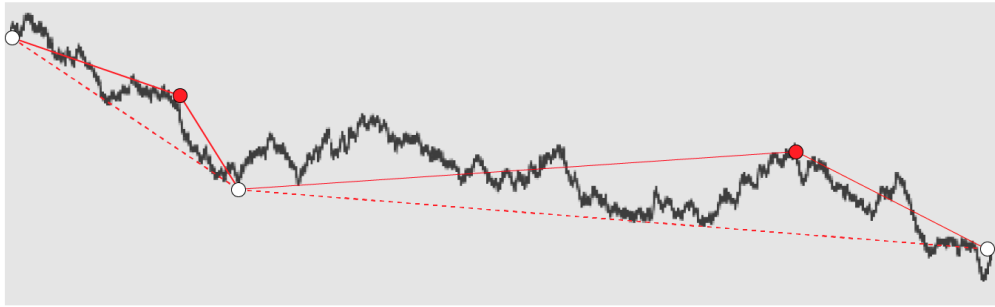
Figure 3: Dividing time intervals by iterative application of the largest triangle algorithm [30]. In the initial iteration (top), the algorithm finds the peak or trough point that forms the largest triangle in the time series, then segments the time interval at this identified time point. Subsequently, in the second iteration (bottom), the algorithm discovers peak or trough points in the time intervals obtained in the first iteration. The iterative process continues until the area of the largest triangle falls below a chosen threshold.
