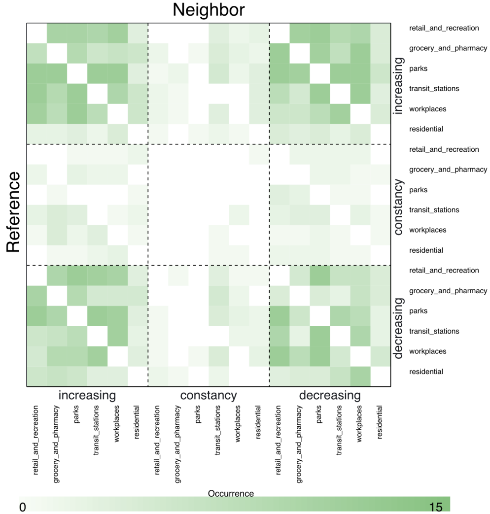
Figure 7: Relation occurrences matrix: Each cell represents the frequency of the target relation ( before in this example) between two patterns across various attributes. The matrix rows and columns are divided into three blocks corresponding to increase, constancy, and decrease patterns. Darker shades indicate more frequent occurrences, while lighter ones signify fewer.
