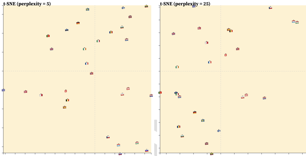
Figure 10: t-SNE projections of the set of countries obtained with perplexity values of 5 (left) and 25 (right), based on the similarity between the matrices of the normalized occurrence frequencies of the before relation. The projection provides a spatial representation of the similarities.
