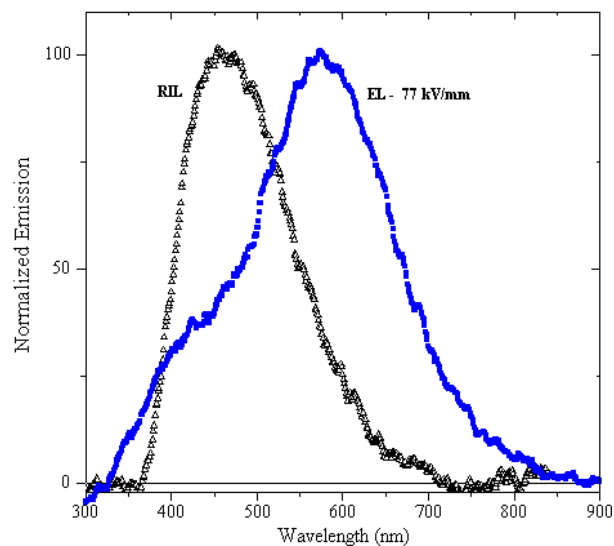
Figure 3: EL spectrum under AC compared to the luminescence spectrum due to charge recombination (RIL)
