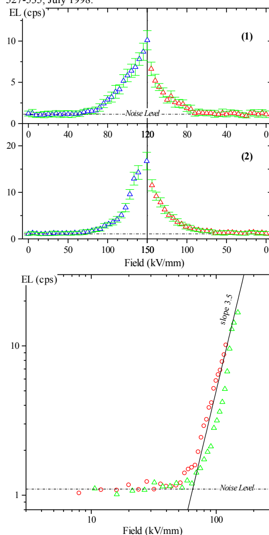
Fig. 1(b): EL versus DC field characteristics obtained during voltage increases for the two cycles
