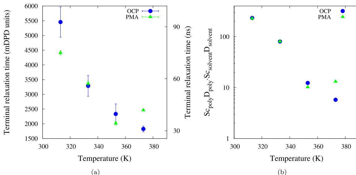
Fig. 12. (a) Terminal relaxation time, \tau_{term} as a function of temperature, T at zero shear rate for OCP and PMA solutions. (b) Sc_{poly} D_{poly} \cdot Sc_{solvent} D_{solvent} as a function of temperature (refer to Eq. (25)).
