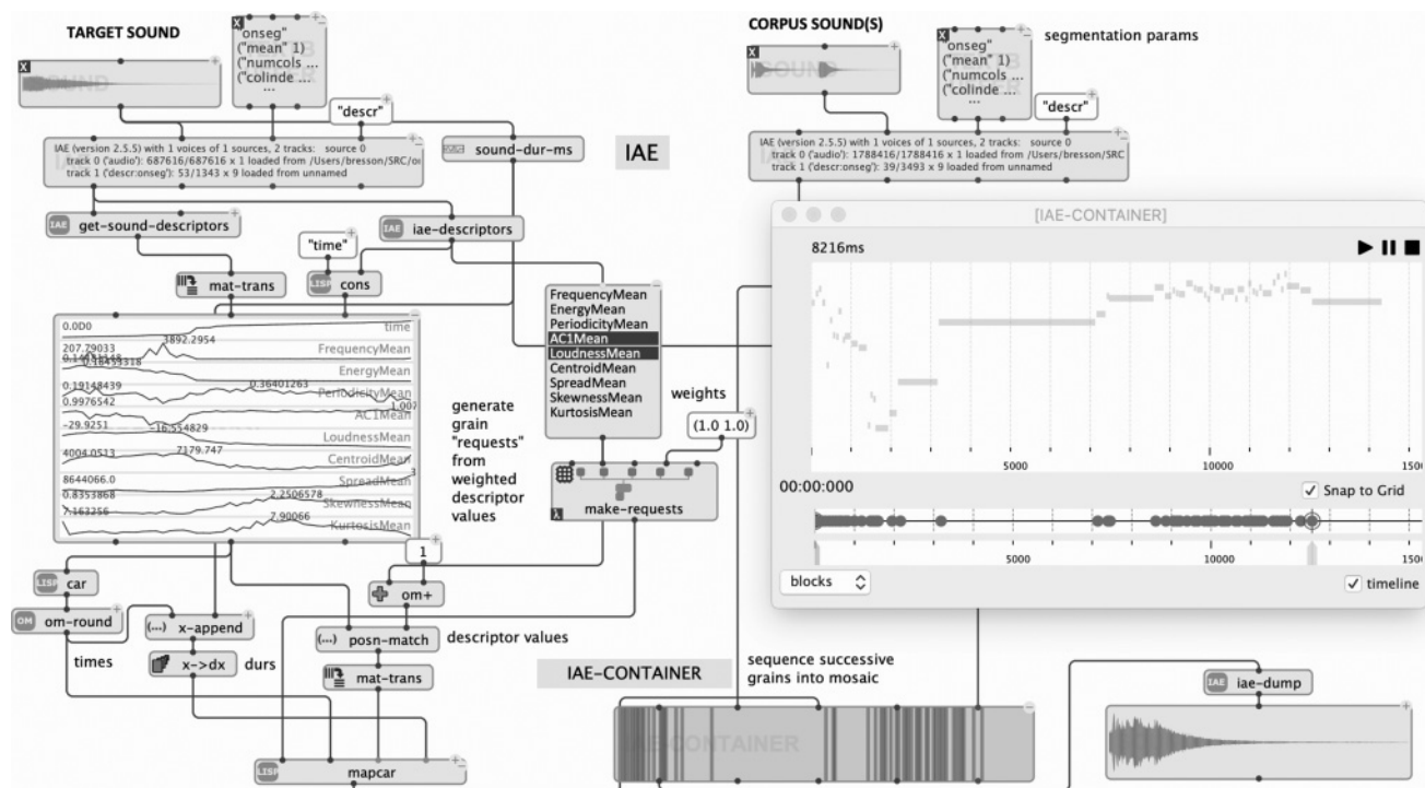
Figure 5. Audio mosaicking with OM# and IAE: audio segmentation and descriptor analysis of a target (top left); generation of descriptor queries (lower left);
