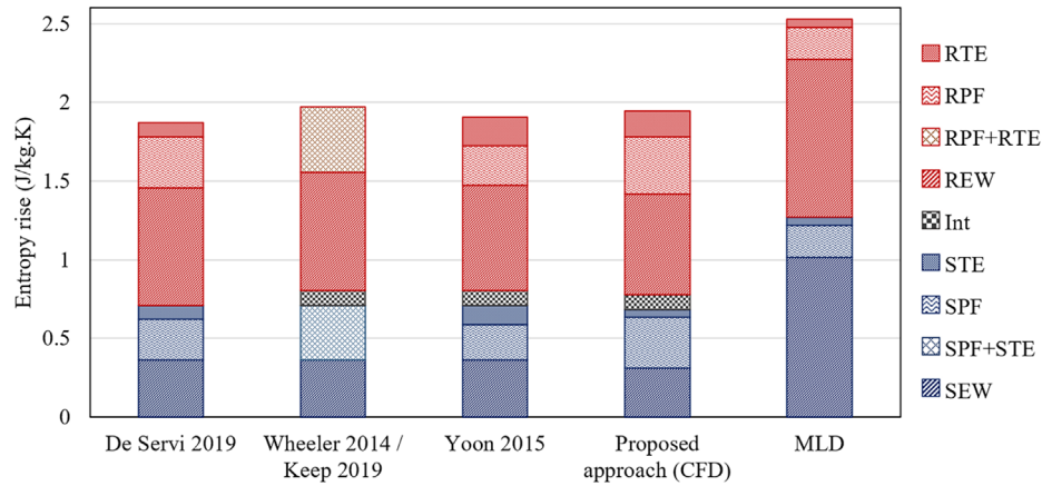
Fig. 11 Comparison between different loss breakdown approaches applied to the first stage of the \text{sCO}_2\text{-C}_6\text{F}_6 four-stage design
