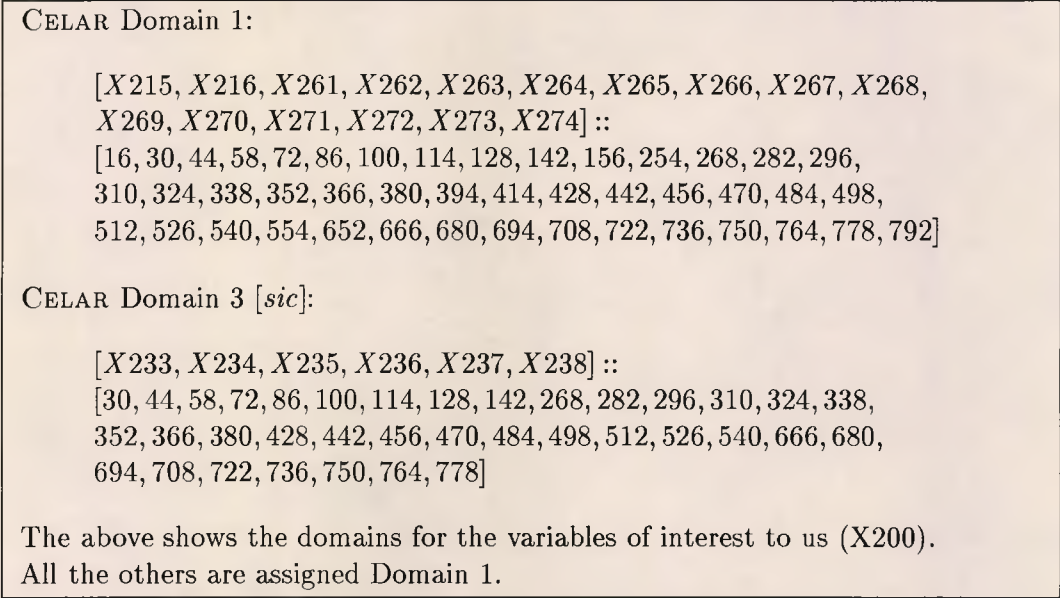
Figure 12.2: \zeta variable domains
