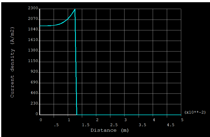
Figure 5.3.13 – Variation of current density through the solid conductor ( d = 25.23 \text{ mm} ) as in [98-99] with distance from its centre – I = 1 \text{ A} , 50 \text{ Hz}
