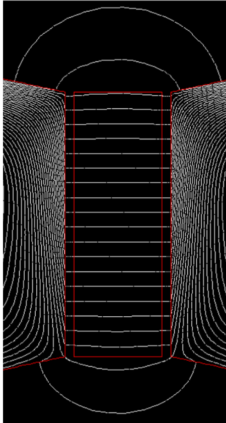
Figure 5.4.13 – Magnetic flux lines through the MSM element and the airgap between the poles of the magnetic circuit
