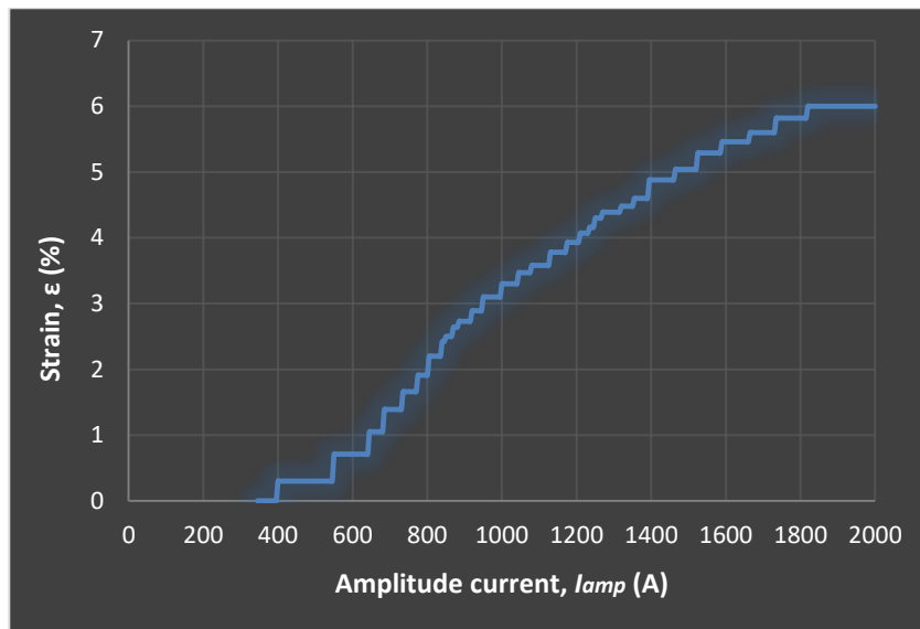
Figure 5.5.4 – Variation of strain of the MSM element, \varepsilon with amplitude current in the conductor I_{amp} ( r = 80 mm, w = 20 mm, t = 50 mm)
