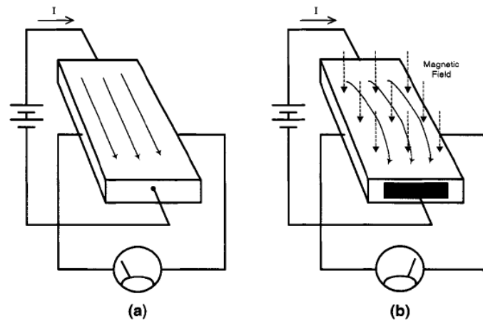
Figure 2.4.1 – Hall effect [36]
