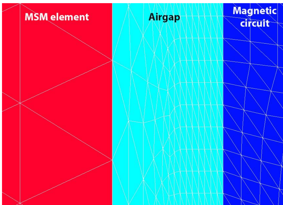
Figure 5.4.9 – Mesh of the airgap between the MSM element and the poles of the rectangular magnetic circuit
