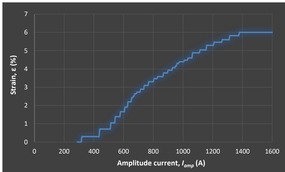
Figure 5.5.3 – Variation of strain of the MSM element, \epsilon with amplitude current in the conductor I_{amp} ( r = 55 mm, w = 20 mm, t = 35 mm)
