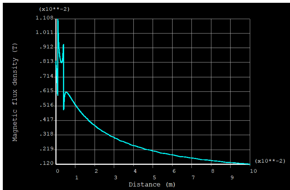
Figure 5.4.2 – Variation of magnetic flux density with distance from the surface of the conductor when an MSM element is placed at the distance of 1 mm from its surface (amplitude current 1000 A, 50 Hz)
