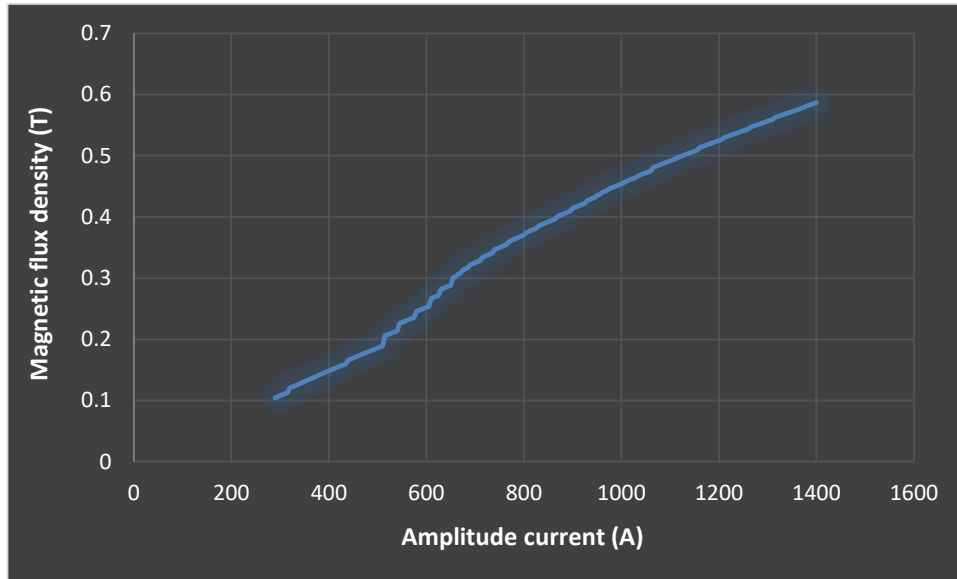
Figure 5.5.2 – Variation of magnetic flux density on the surface of the MSM element, B_{surface} with amplitude current in the conductor, I_{amp} ( r = 55 mm, w = 20 mm, t = 35 mm)
