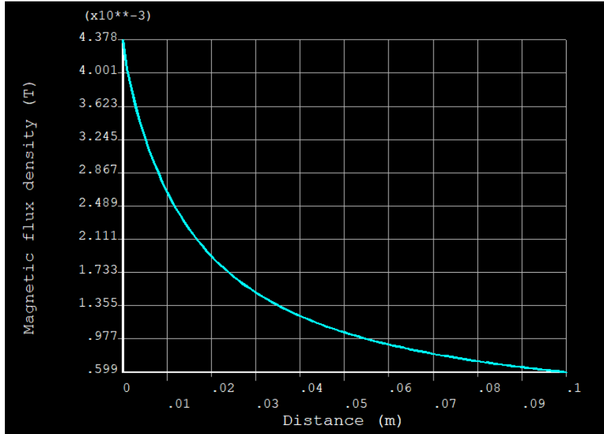
Figure 5.3.8 – Variation of magnetic flux density with distance from the surface of the ACSR 528-Al1/69-ST1A conductor (amplitude current 500 A, 50 Hz)
