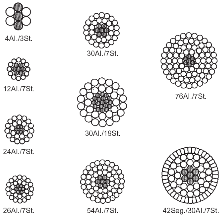
Figure 3.1.2 – Typical stranding of ACSR conductors (part2) [43]
