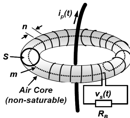
Figure 2.2.1 – Rogowski coil [25]
