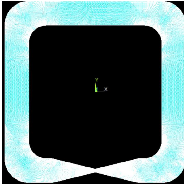
Figure 5.6.1 – Finite element mesh in the rectangular magnetic circuit with rounded corners ( w = 20 \text{ mm} , t = 35 \text{ mm} , r = 55 \text{ mm} )
