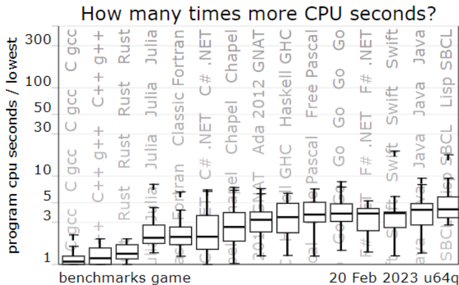
Figure 2.3: Performance of top 15 implementations of tested algorithms in Benchmarks Game.
