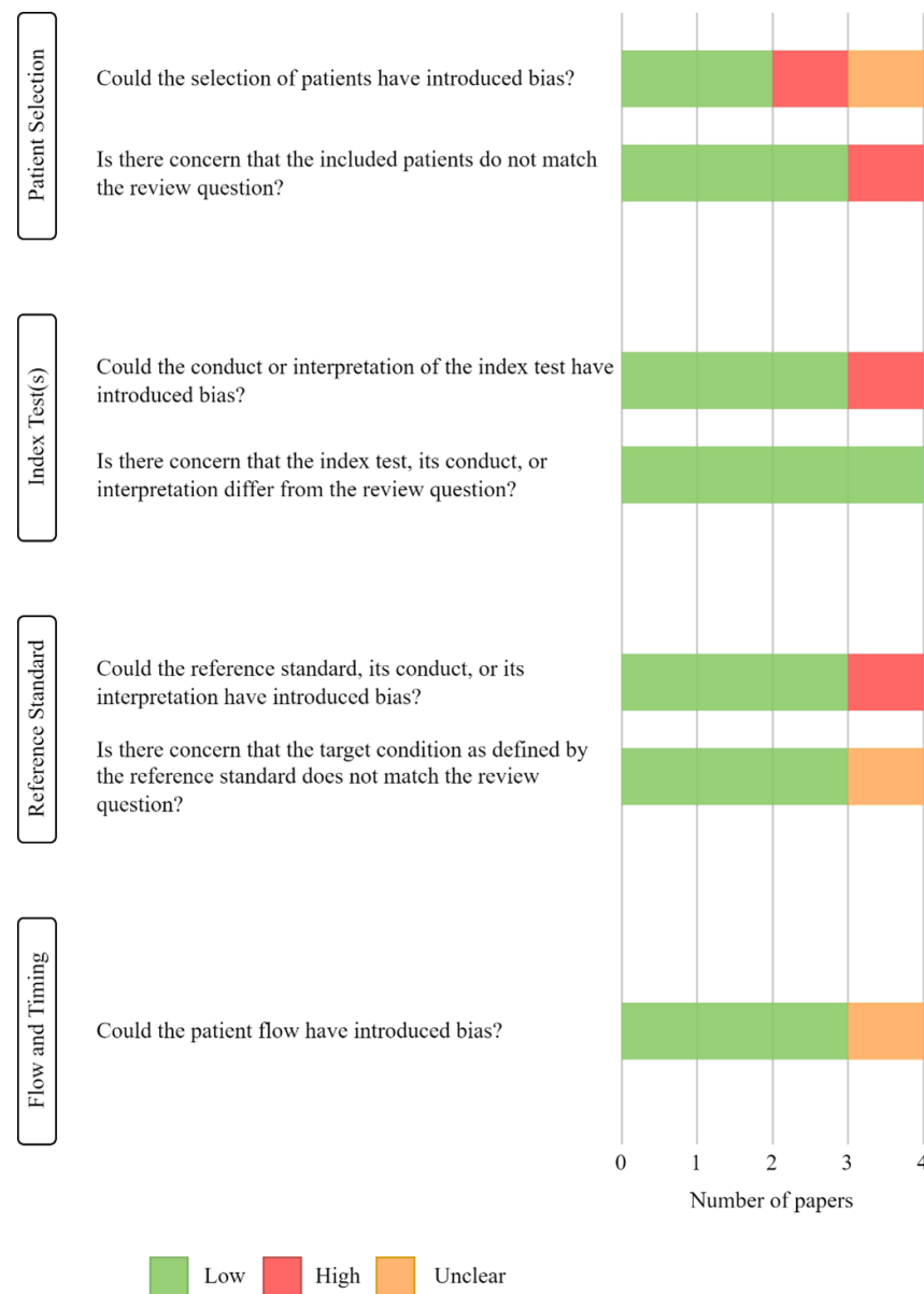
Figure 2. Results of QUADAS-2 tool assessment, displaying the quality and the risk of bias of the included studies.
